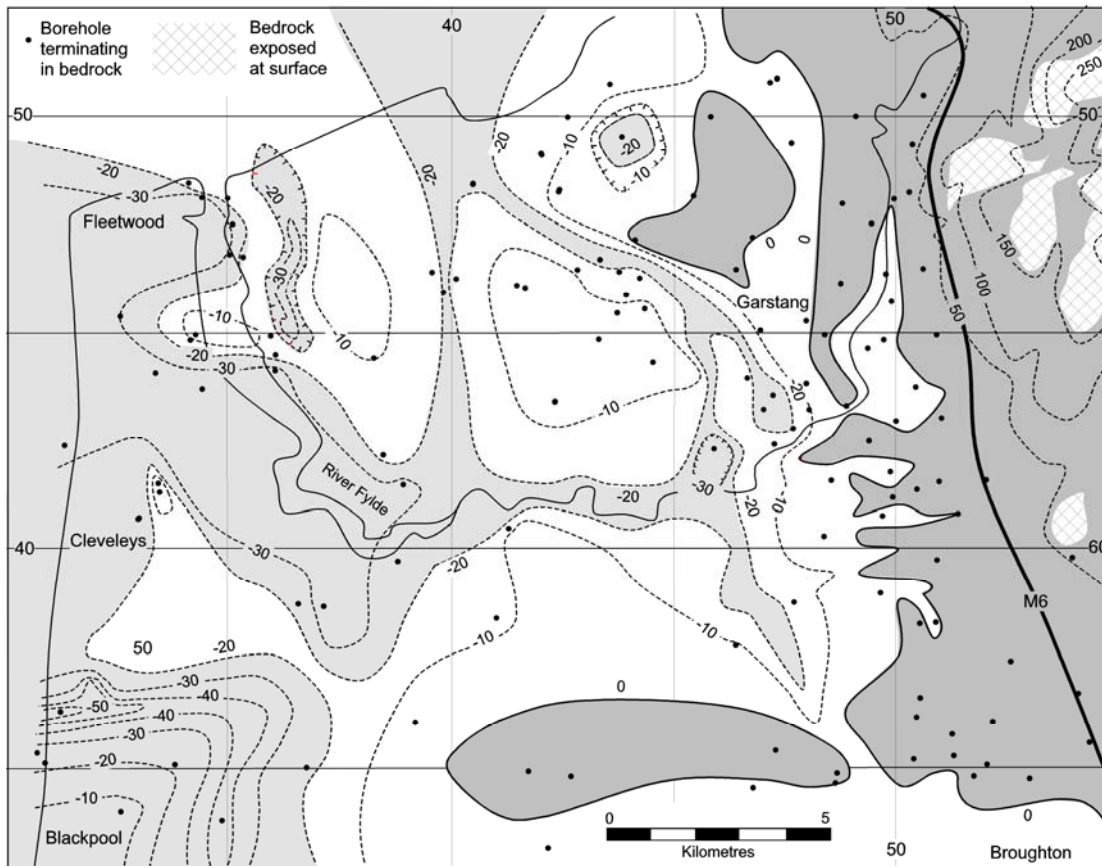
Figure 4: Depth of the rock-head beneath the lowlands of the Fylde derived from the borehole coverage, based on Ordnance Survey 1:50,000 series
