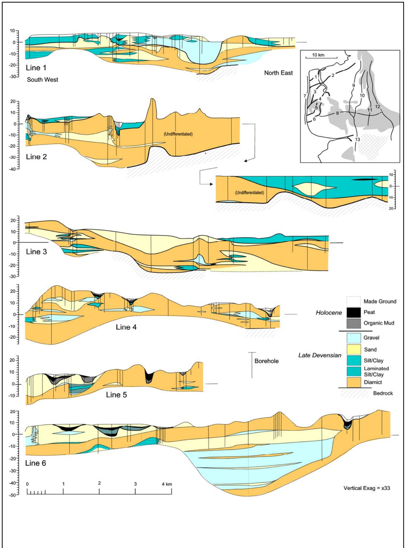
Figure 19: Borehole series compiled to produce serial sections for lines directed across the moraine in an up-ice direction, moraine dip sections. Inset map shows the location of lines 1-6
