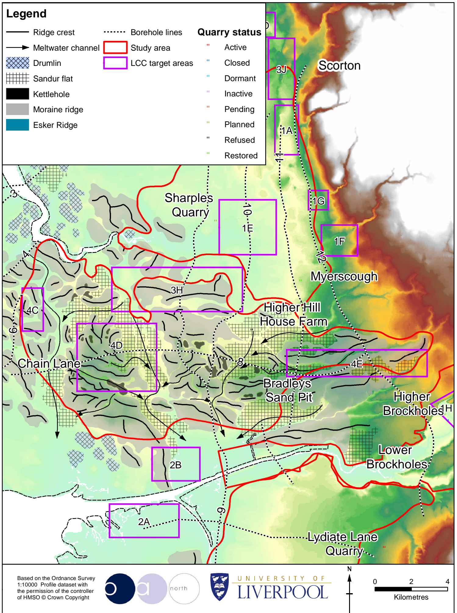
Figure 23: Distribution of Lancashire CC study areas, extraction sites, the geomorphology and the lineations of boreholes
