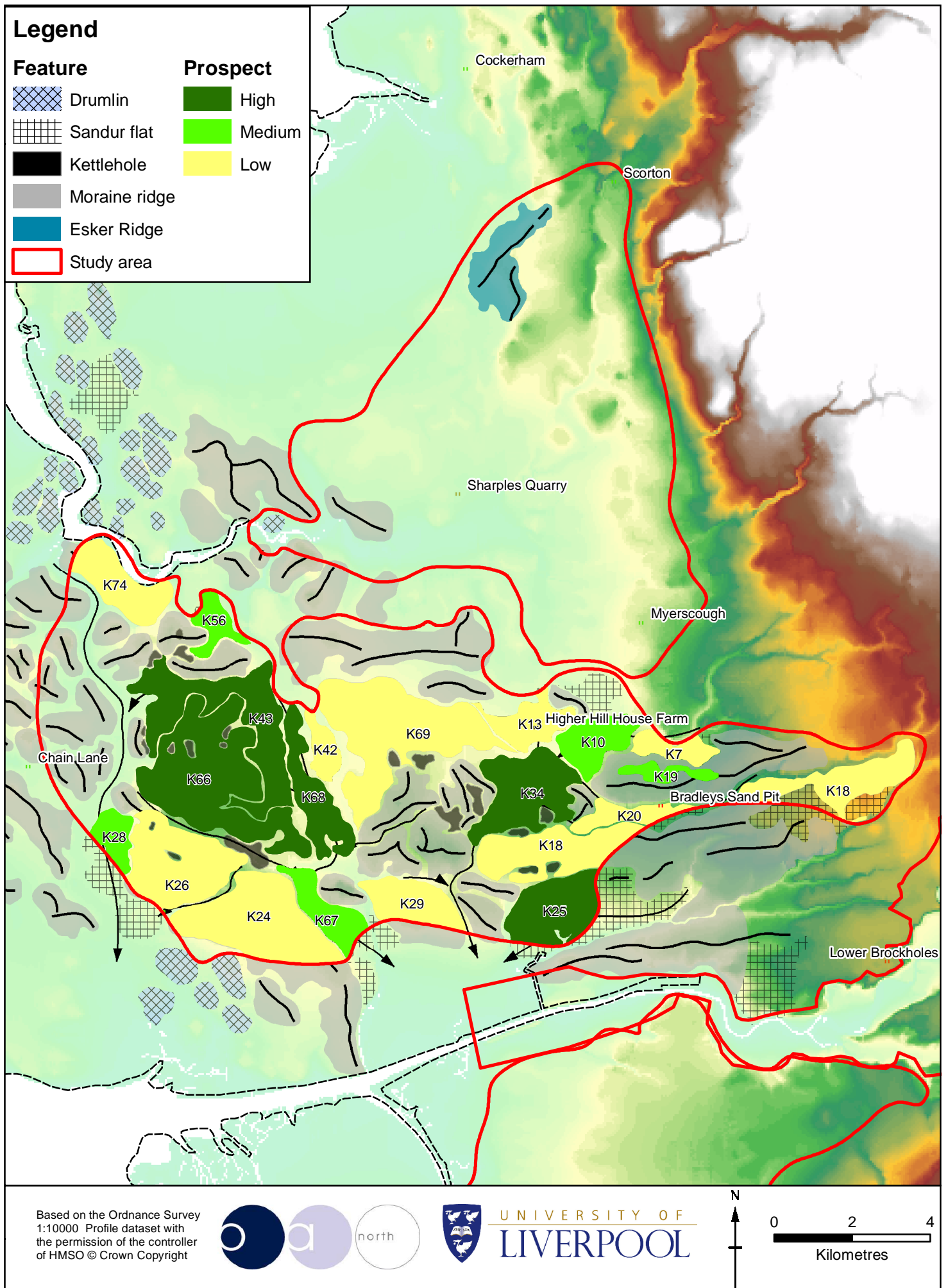
Figure 24: Resource Block ranking in terms of aggregate quality and quantity
