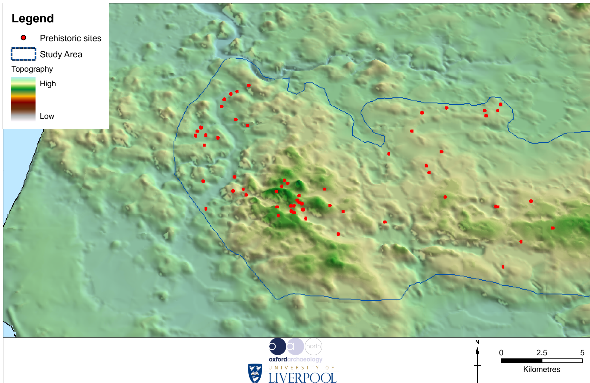
Fig 59: Enhanced topographical model of the study area highlighting coincidence of prehistoric sites and sand islands
