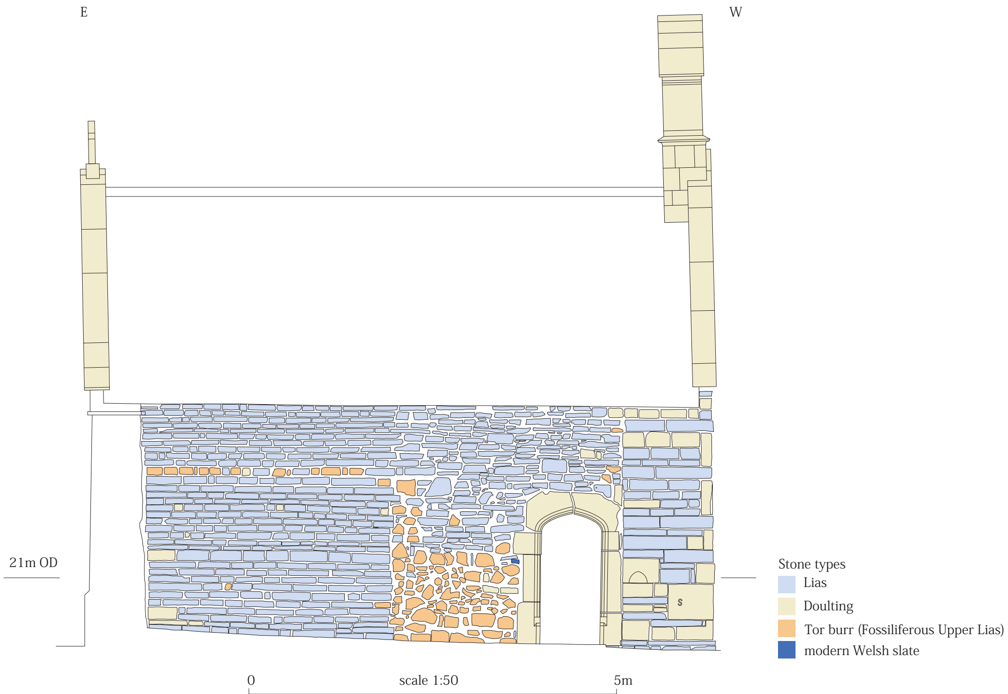
Fig. 5 External North elevation, showing stone types.
