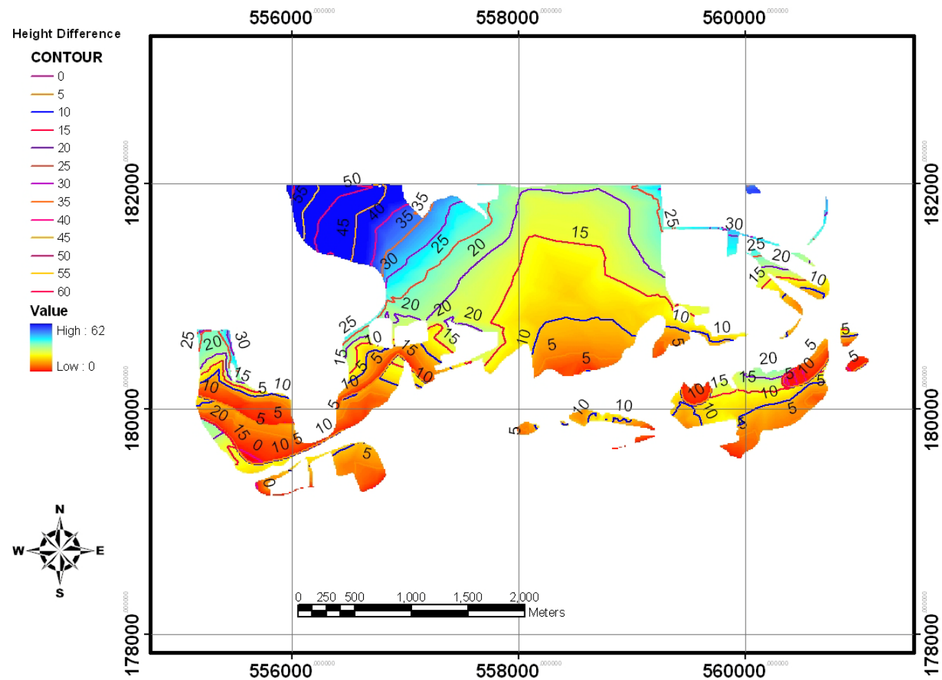
Fig. 15 Geology: Corbets Tey Formation (Lynch Hill and Hackney Gravels); Isopachs
