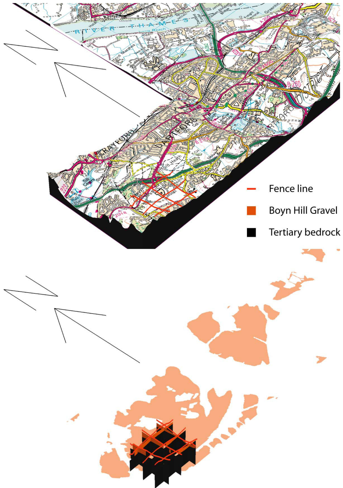
Fig. 19 Geology: Bexley Heath Hospital; investigation of Boyn Hill Gravel boundary, using bespoke geological mapping and fence diagram
