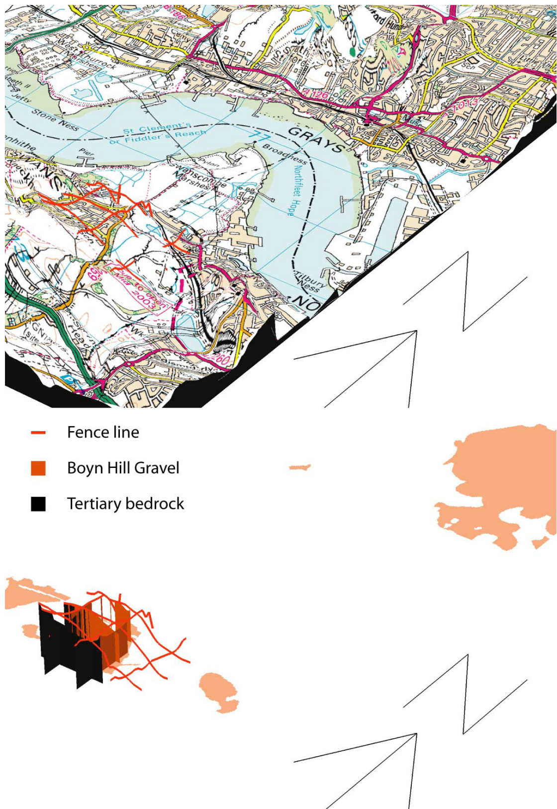
Fig. 18 Geology: Southfleet Road, Swanscombe Community School; Investigation of Boyn Hill Gravel boundary
