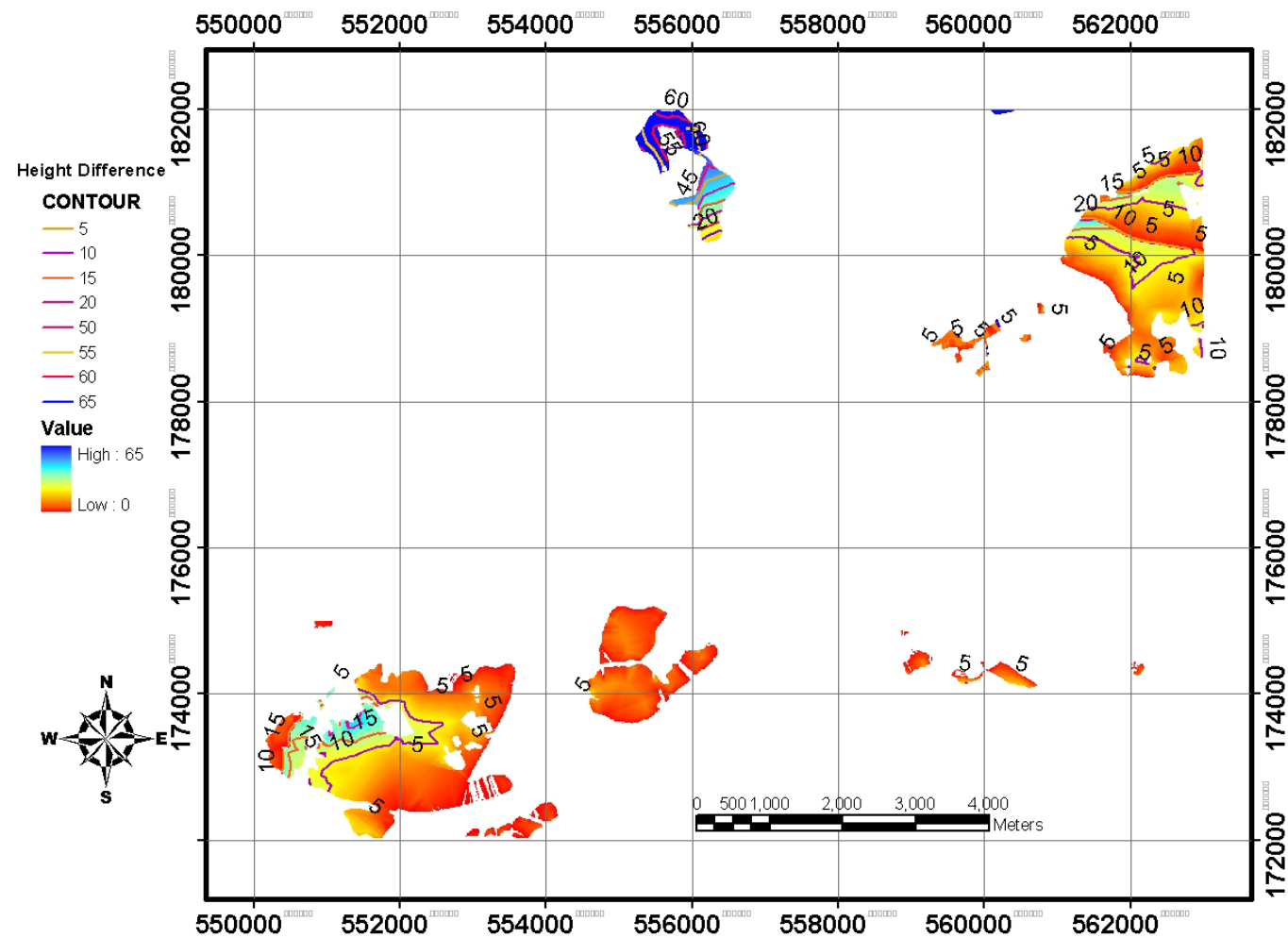
Fig. 13 Geology: Orsett Heath Formation (Black Park and Boyn Hill Gravels); Isopachs
