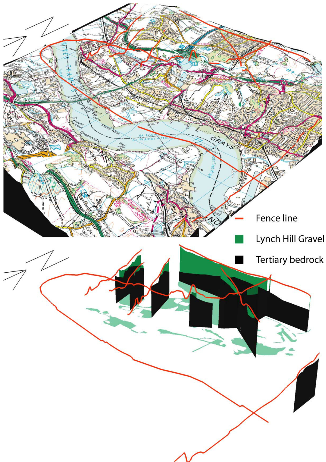
Fig. 14 Geology: Corbets Tey Formation (Lynch Hill and Hackney Gravels); Long profile fence diagram
