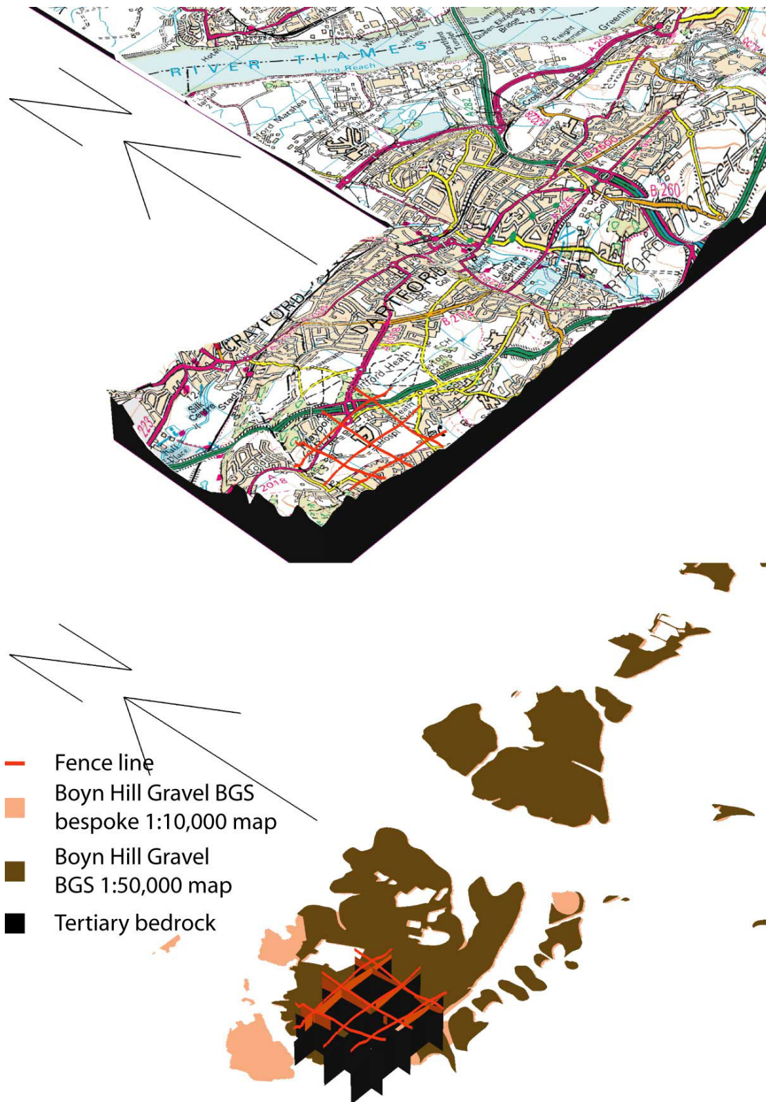
Fig. 20 Geology: Bexley Heath Hospital; Investigation of Boyn Hill Gravel boundary, comparing bespoke geological mapping and 1:50,000 geological mapping
