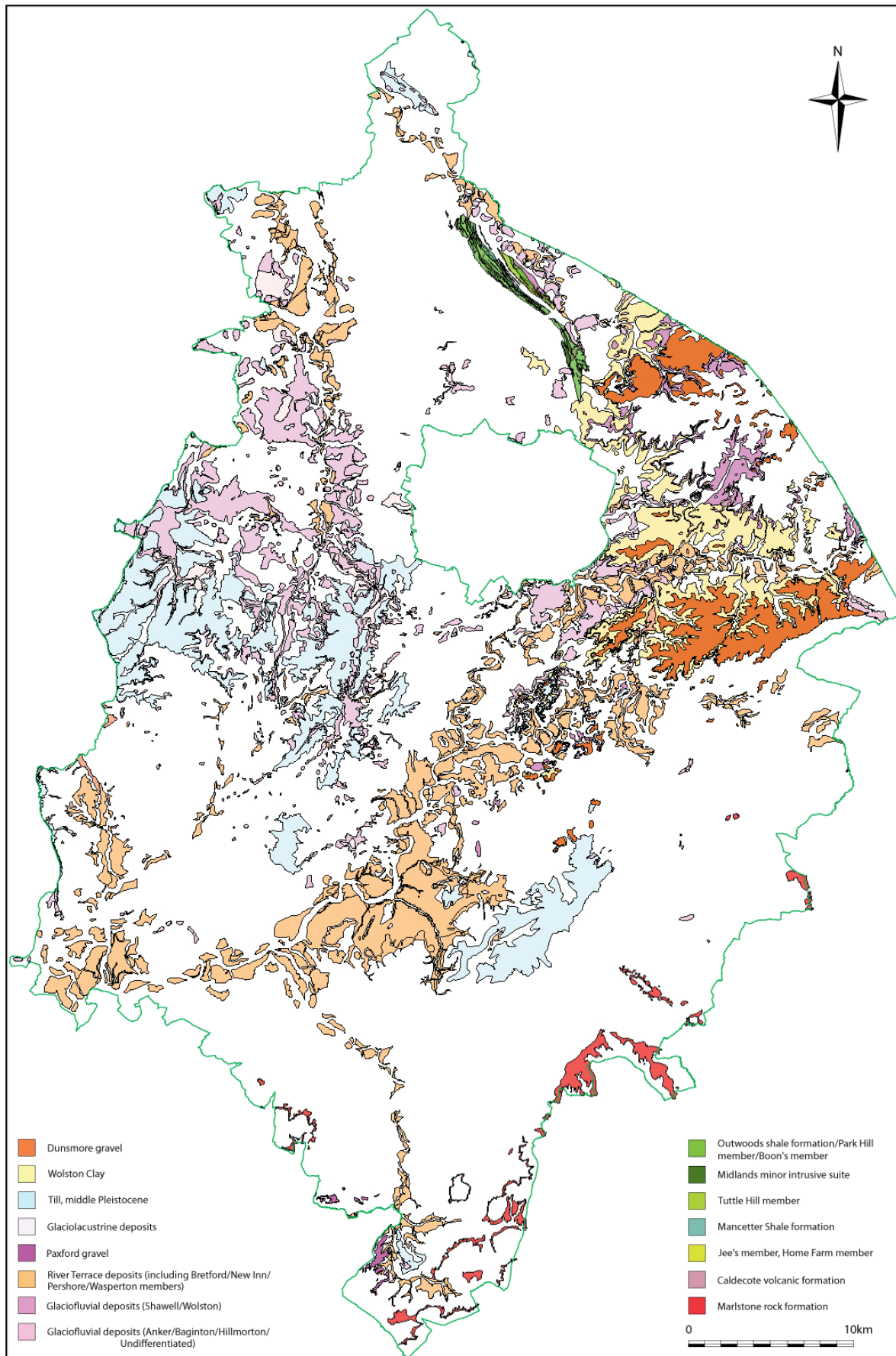
Figure 9 – Mineral Resources
