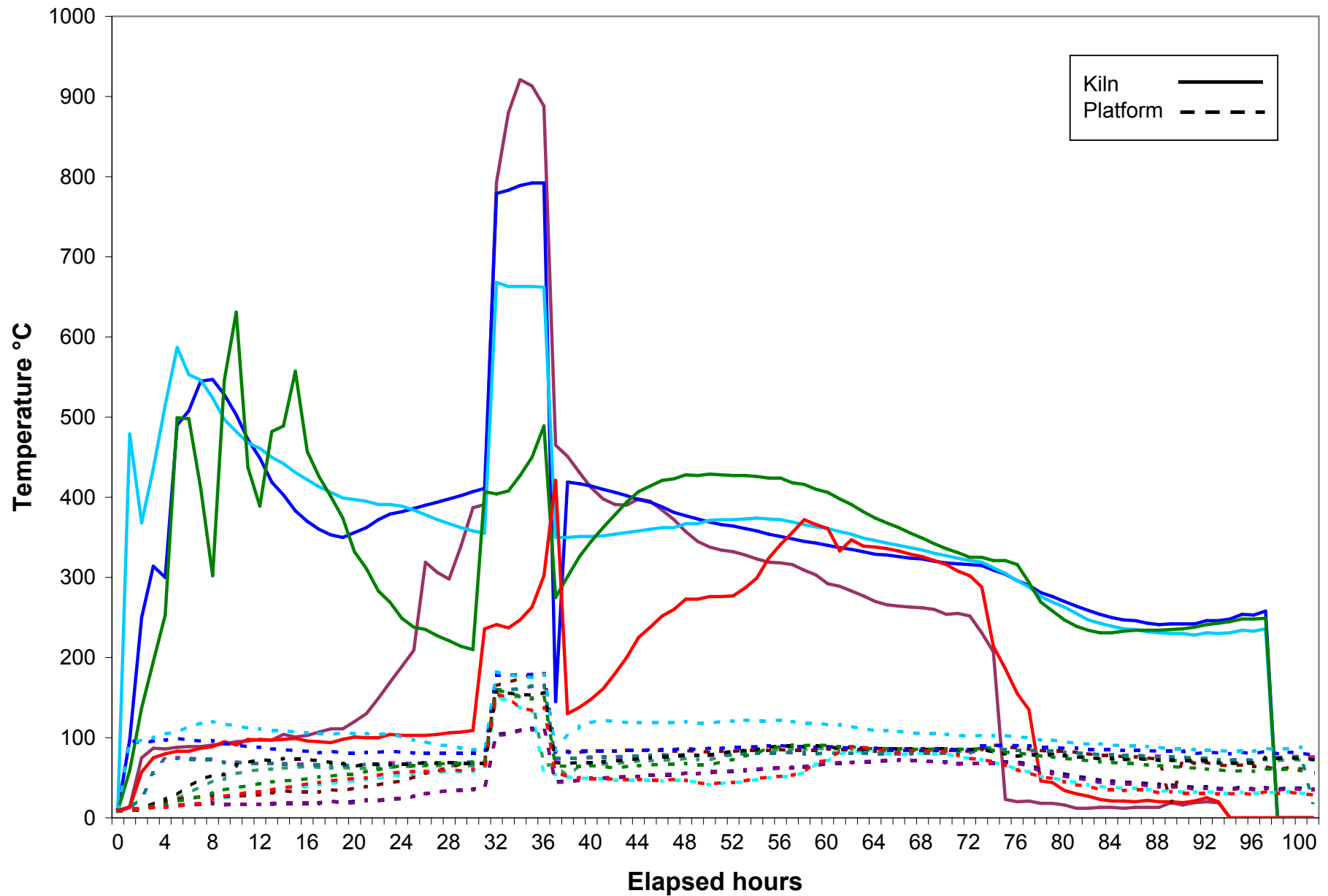
Figure 2: Dalby Experimental Charcoal Burn - Kiln & Platform Temperatures
