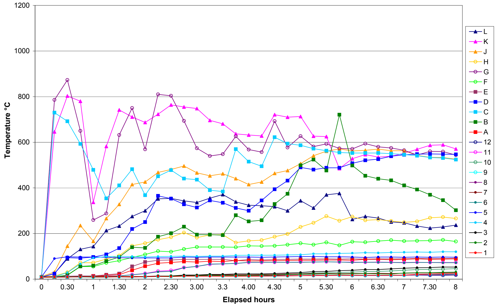
Dalby Traditional Charcoal Kiln - All Temperatures - Initial 8 hrs
