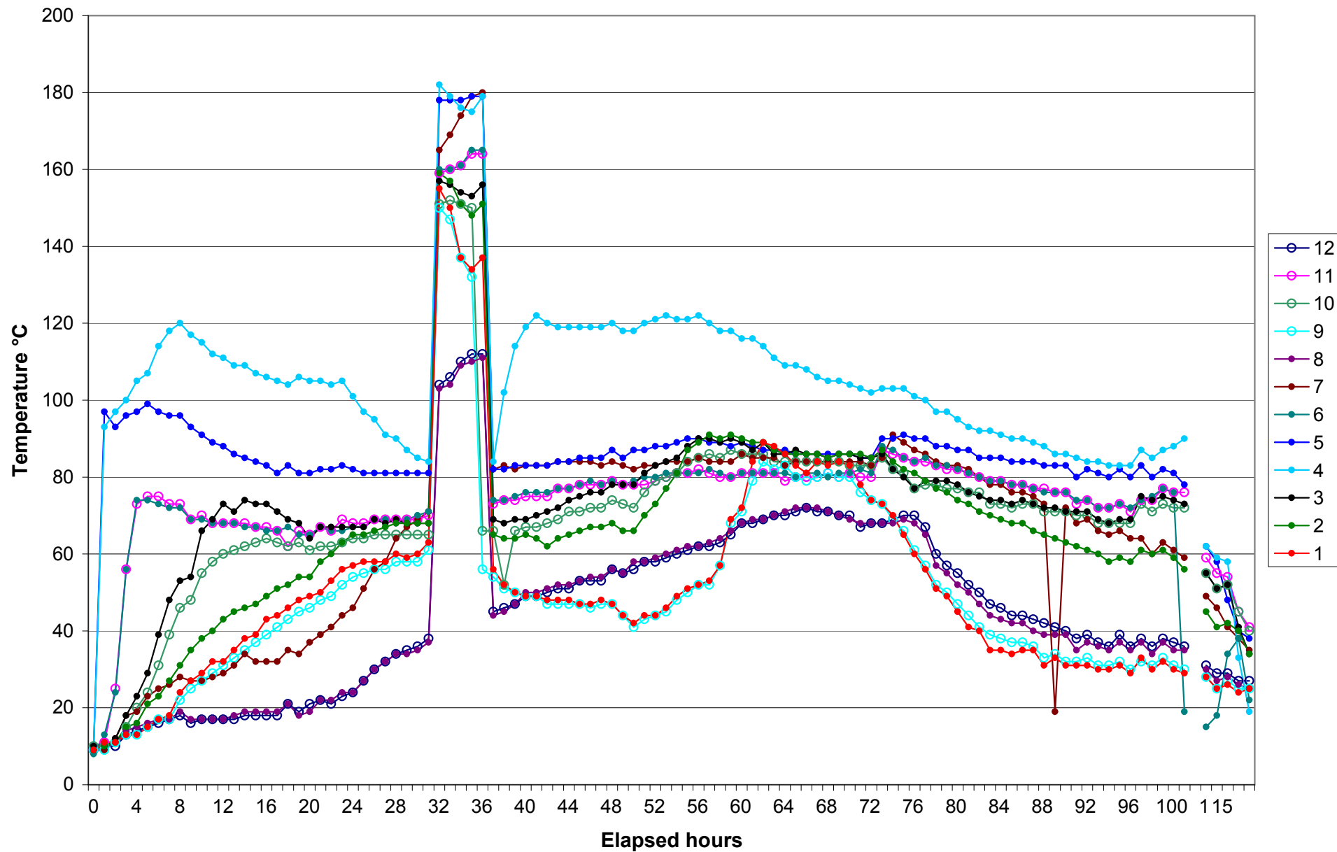
Dalby Traditional Charcoal Kiln - Ground Temperatures
