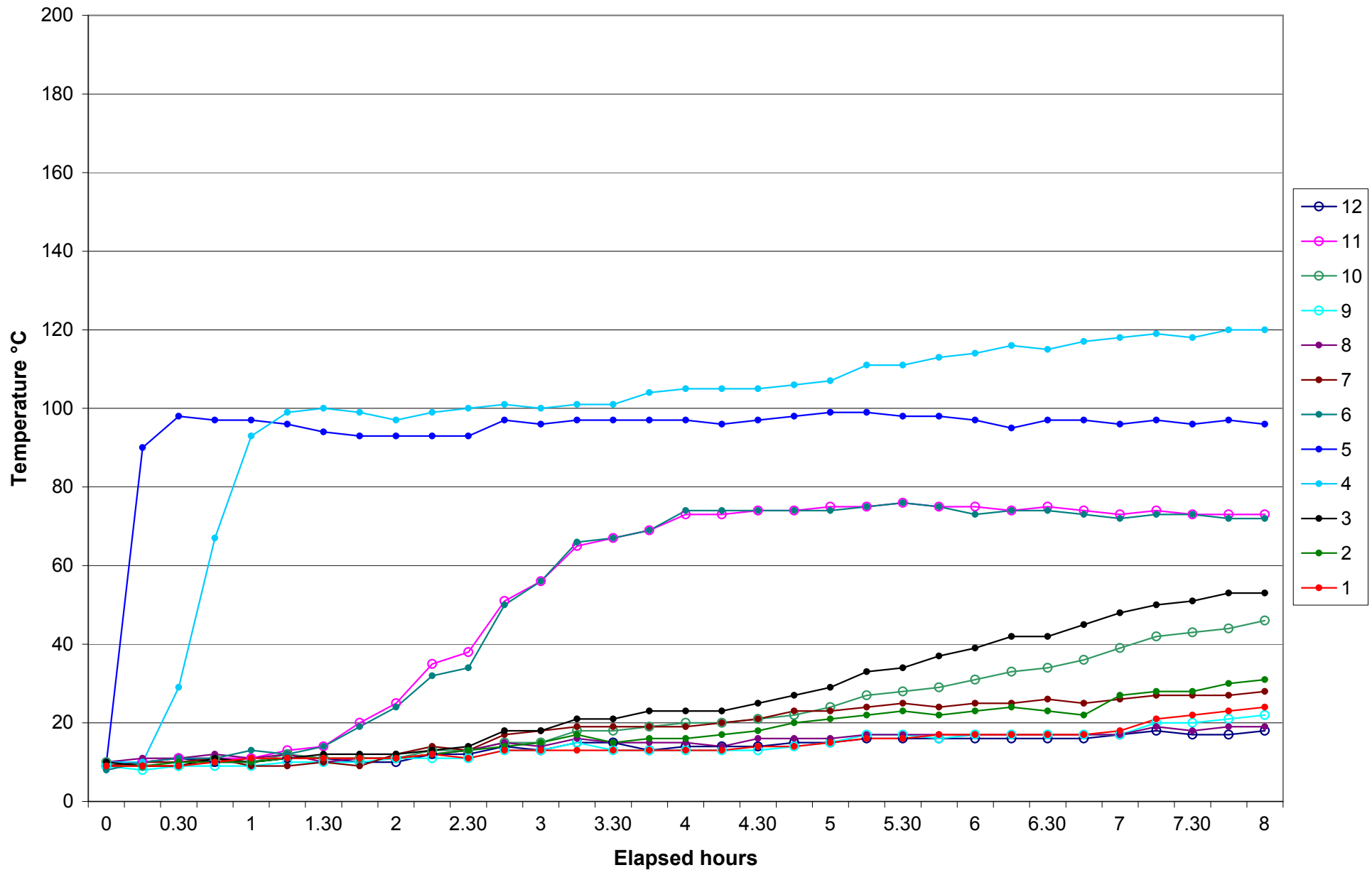
Dalby Traditional Charcoal Kiln - Ground Temperatures - Initial 8 hrs
