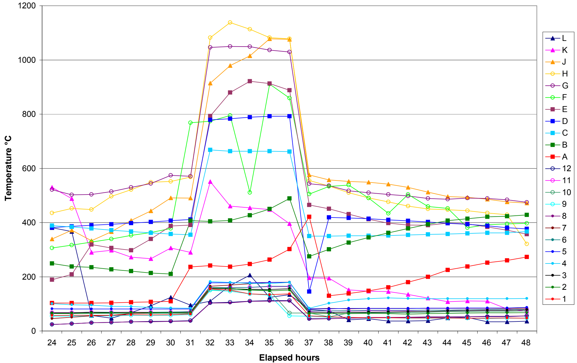
Dalby Traditional Charcoal Kiln - All Temperatures - Second 24 hrs
