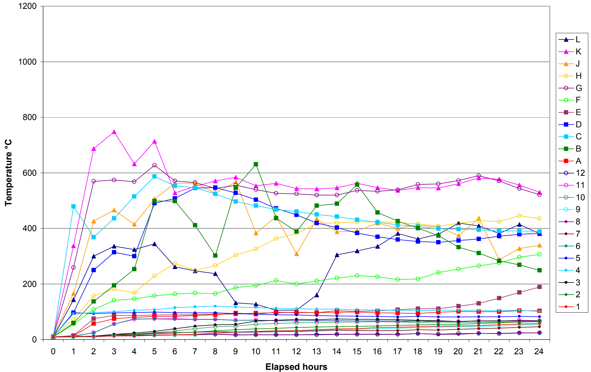
Dalby Traditional Charcoal Kiln - All Temperatures - First 24 hrs
