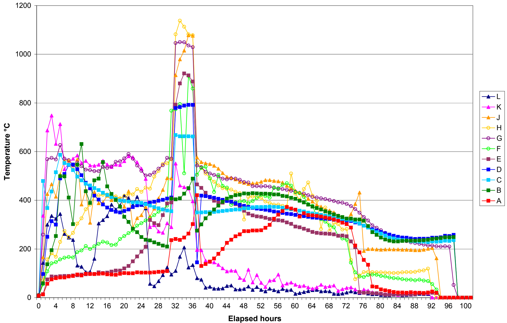
Dalby Traditional Charcoal Kiln - Kiln Temperatures
