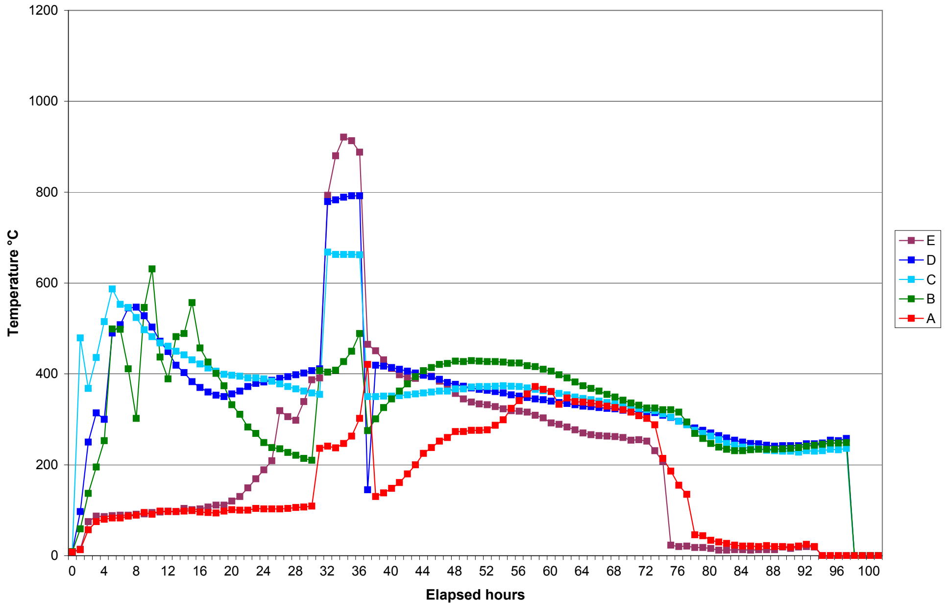
Dalby Traditional Charcoal Kiln - Kiln Temperatures - Pts. A to E
