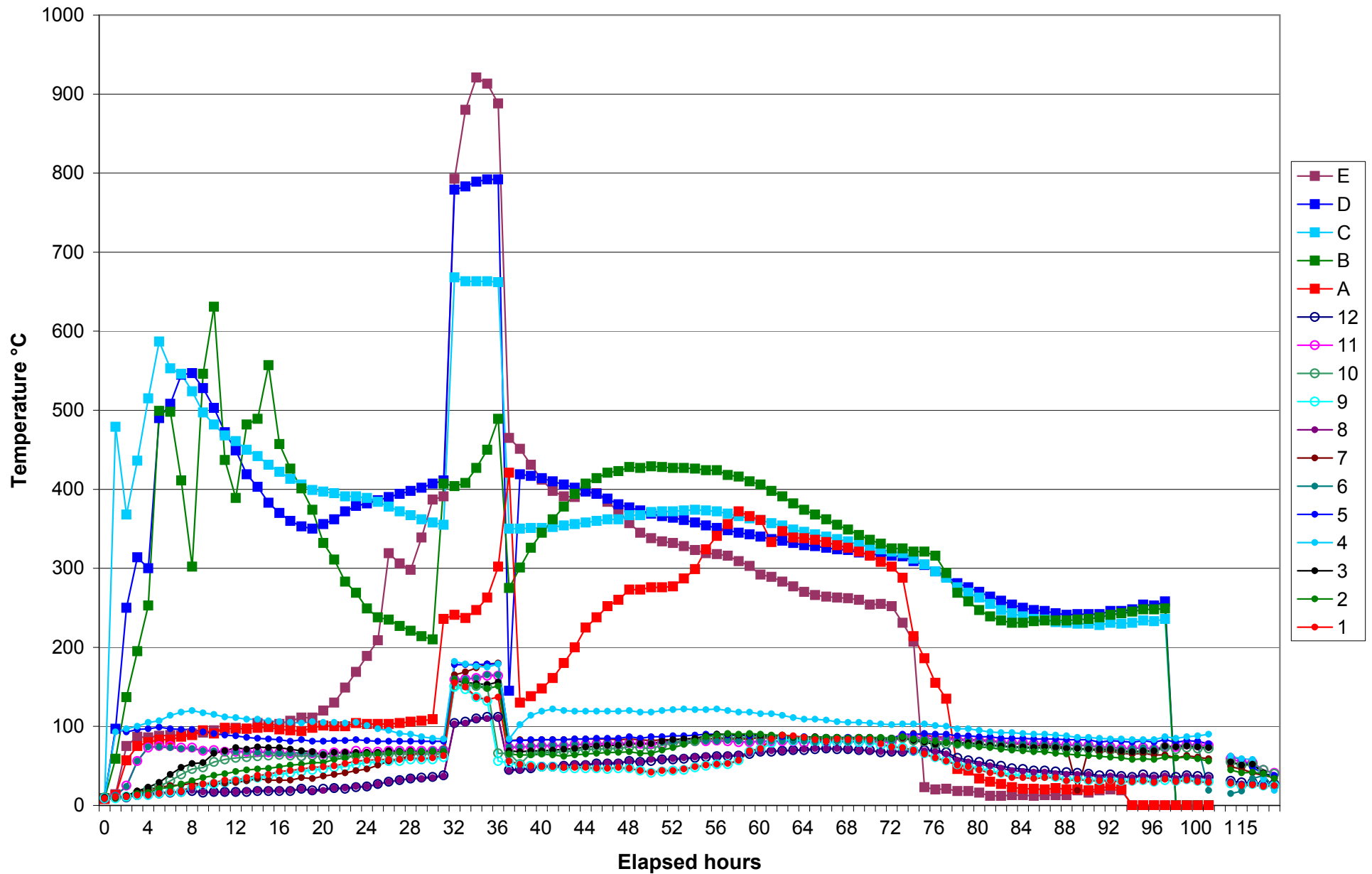
Dalby Traditional Charcoal Kiln - Ground & Kiln (Pts. A to E) Temperatures
