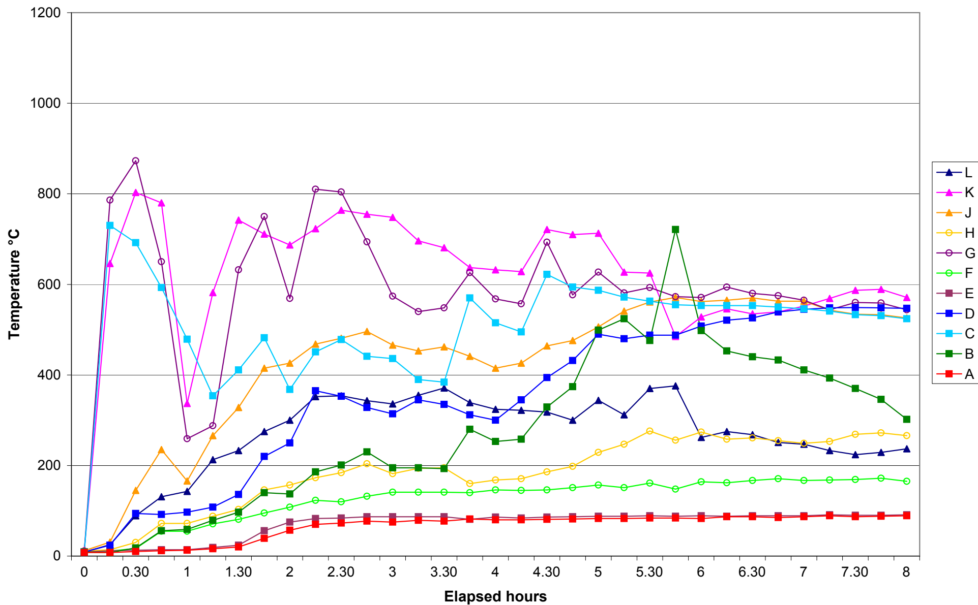
Dalby Traditional Charcoal Kiln - Kiln Temperatures - Initial 8 hrs
