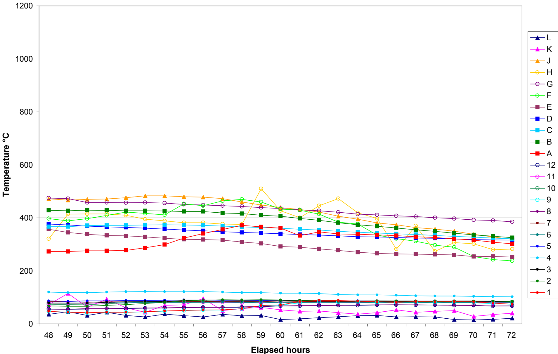
Dalby Traditional Charcoal Kiln - All Temperatures - Third 24 hrs
