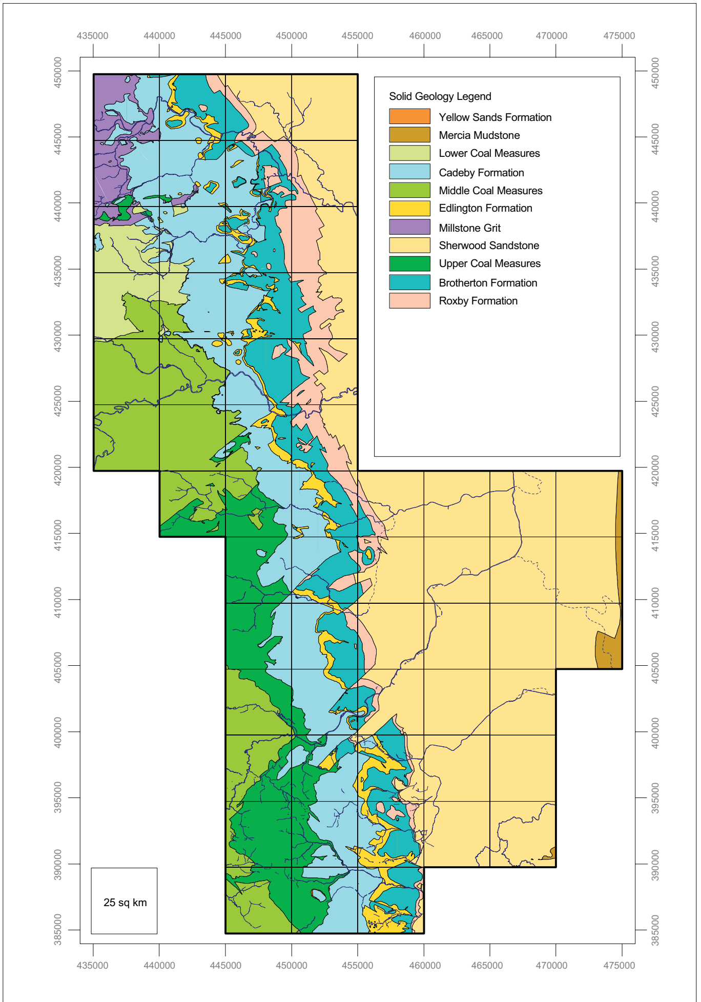
Fig. 1.2. Solid geology
