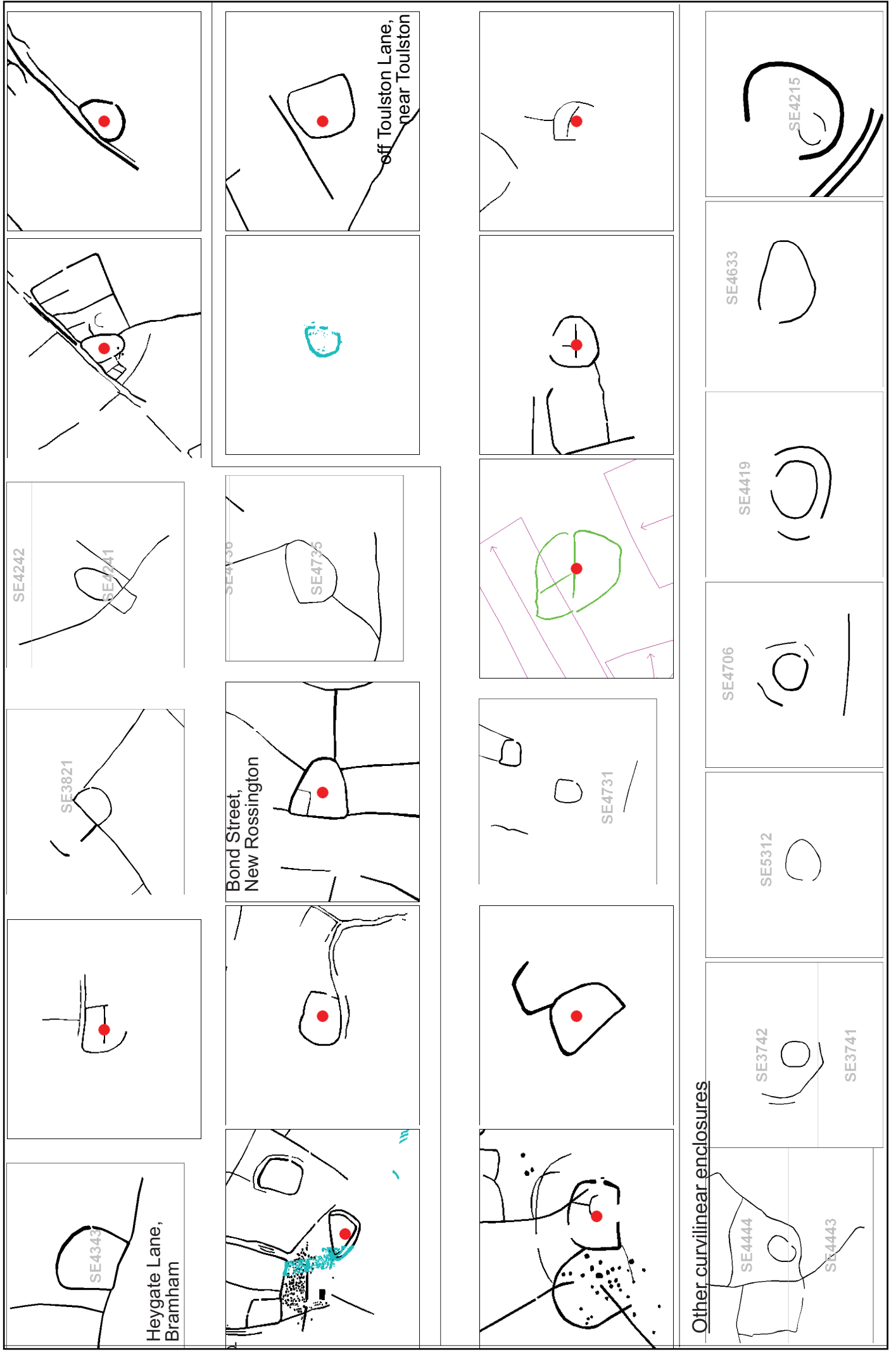
Fig. 6.10. Examples of D-shaped enclosures
