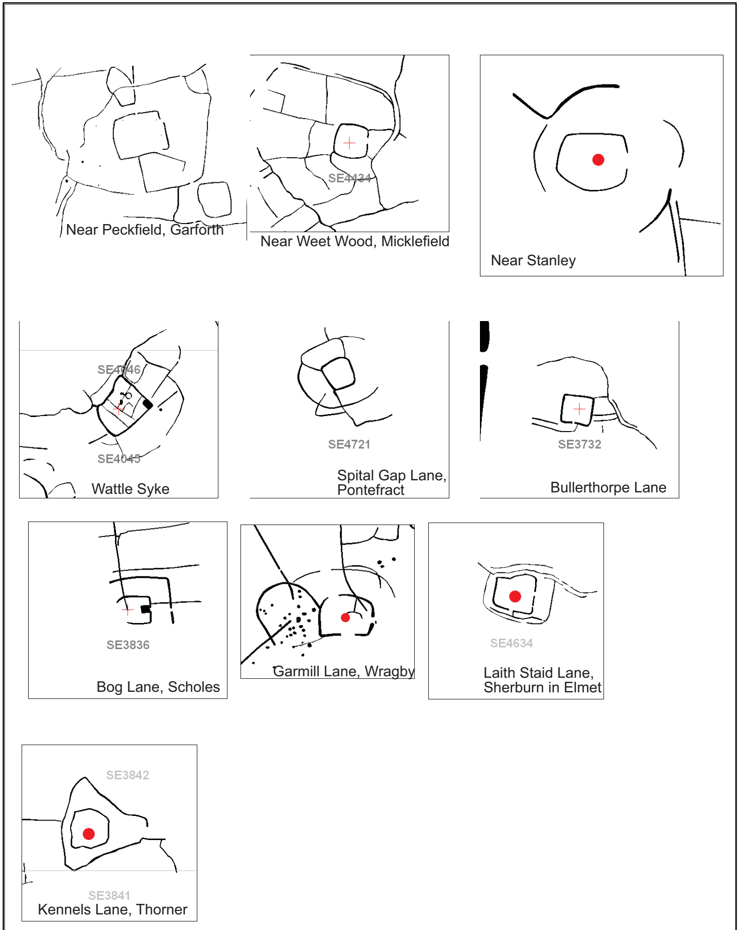
Fig. 6.16. Examples of enclosures with outer compounds
