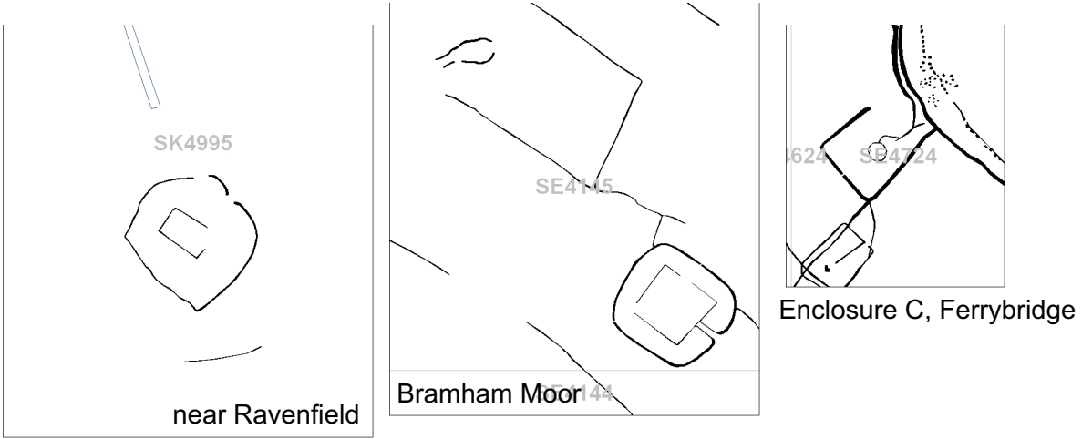
Fig. 6.20. Examples of possible shrines or ritual enclosures
