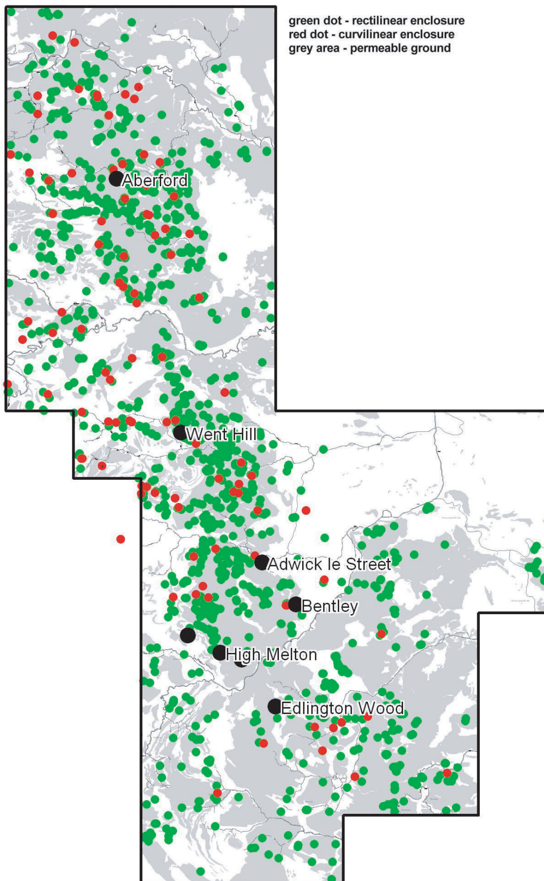
Fig. 6.11. Distribution of rectilinear and curvilinear enclosures
