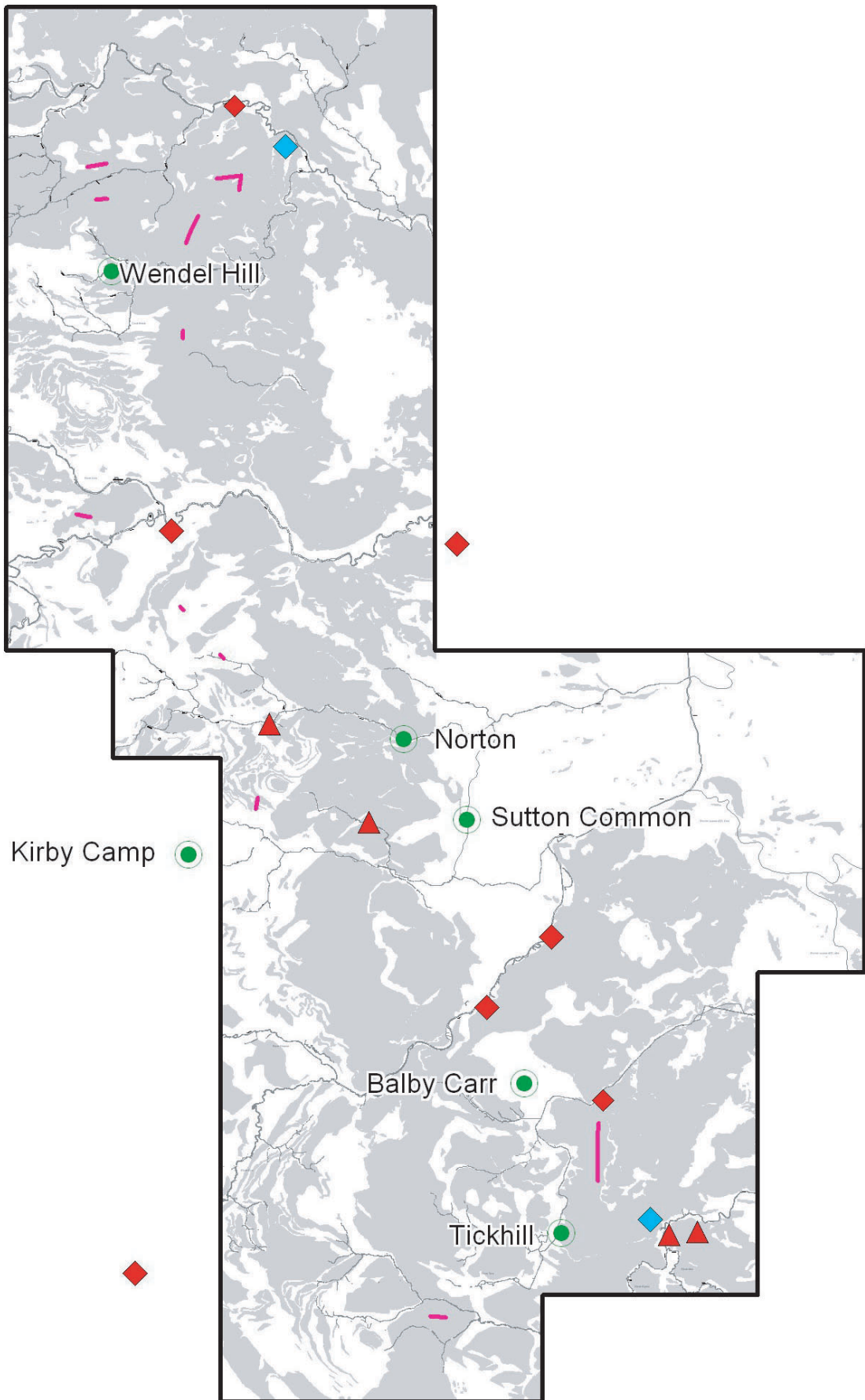
Fig. 6.21. Distribution of Iron Age forts, Roman forts and fortlets and Roman roads
