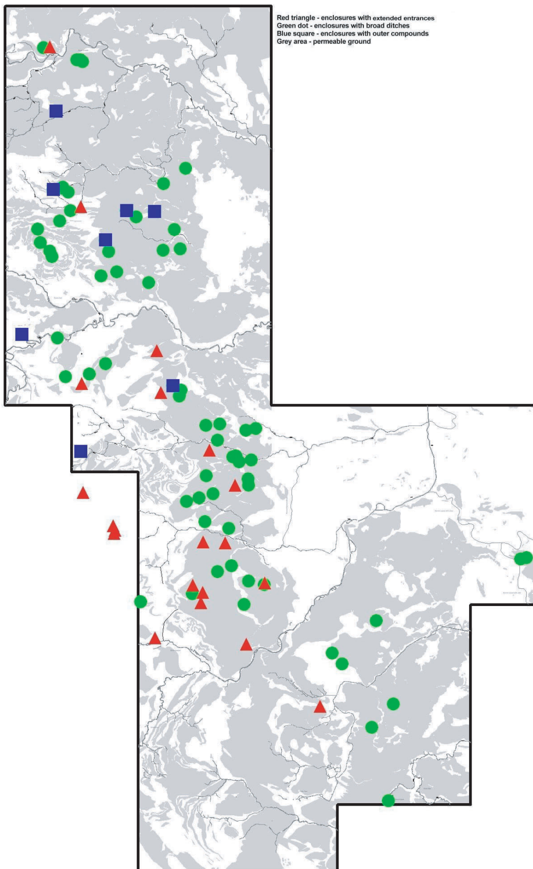
Fig. 6.14. Distribution of different types of enclosures
