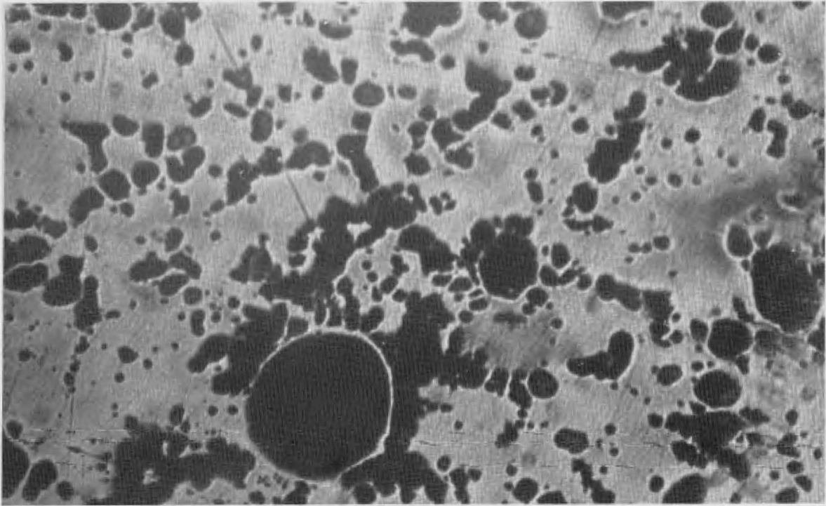
Plate XIV. Blister copper alloy. Mag. \times 300 . (with permission of the Institute of Archaeology, London.)
