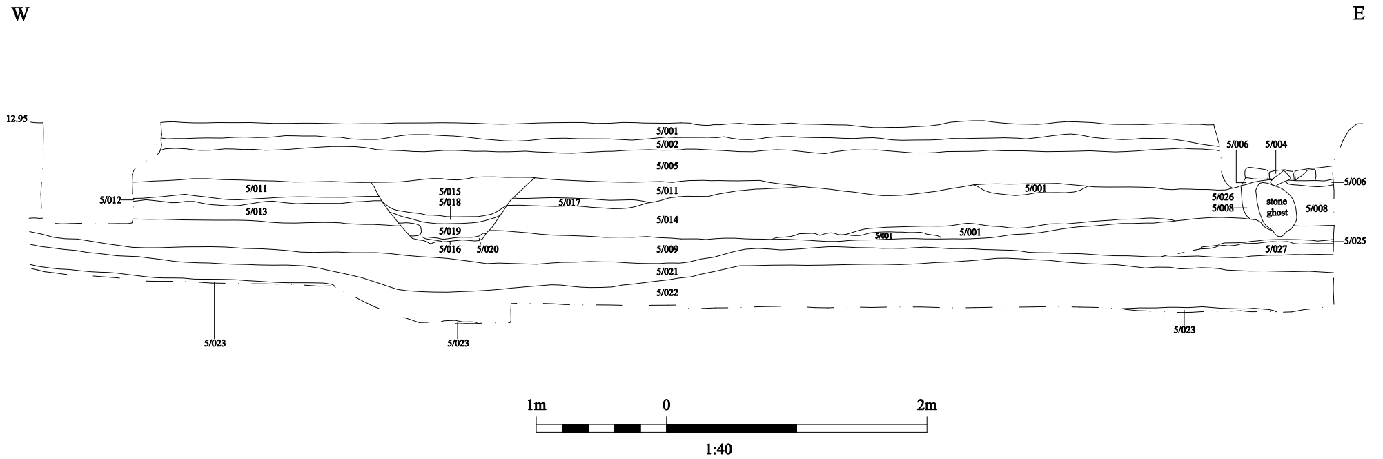
Figure 12: South facing section of Trench 5
