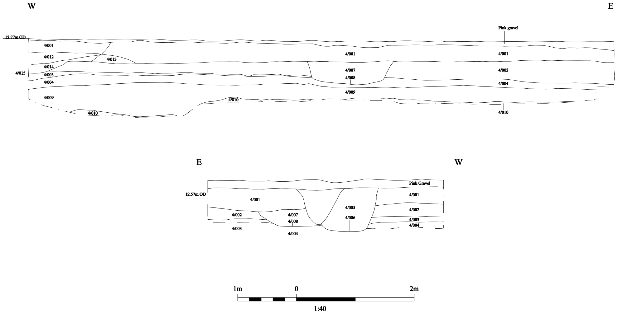
Figure 11: Trench 4: North & South Facing Sections
