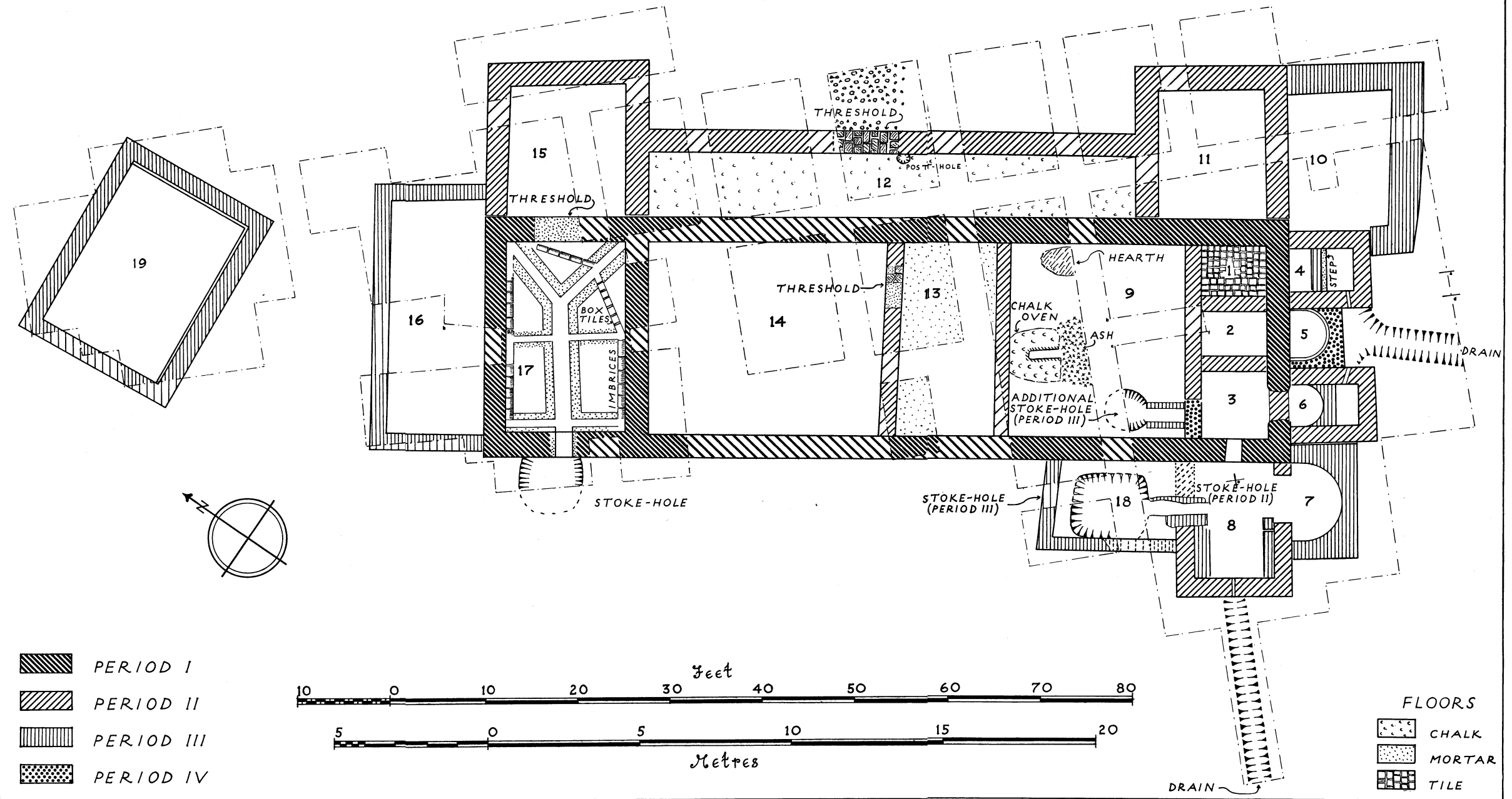
Fig. 2. Composite plan of the villa and outhouse
