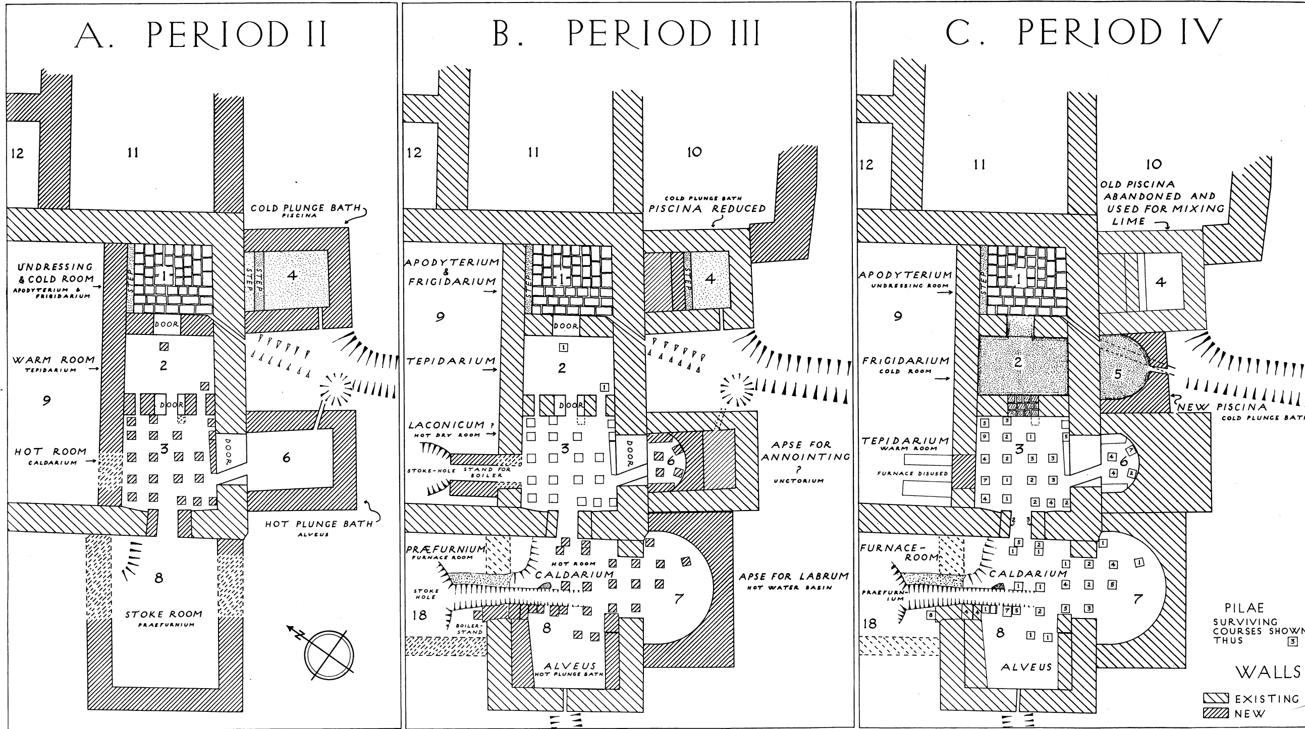
Fig. 3. Details of the Periods II-IV alterations of the bath block
