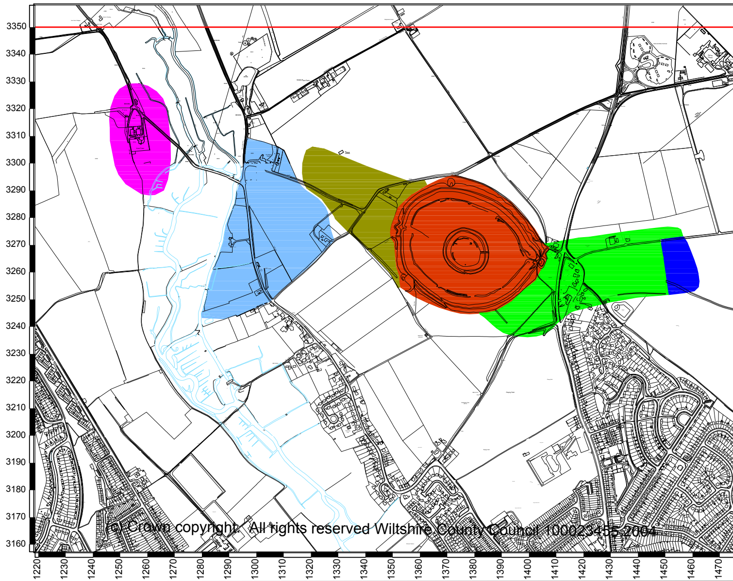
The Archaeology of Wiltshire's Towns: Sorviadunum Fig. 11: Plan Form - Medieval
