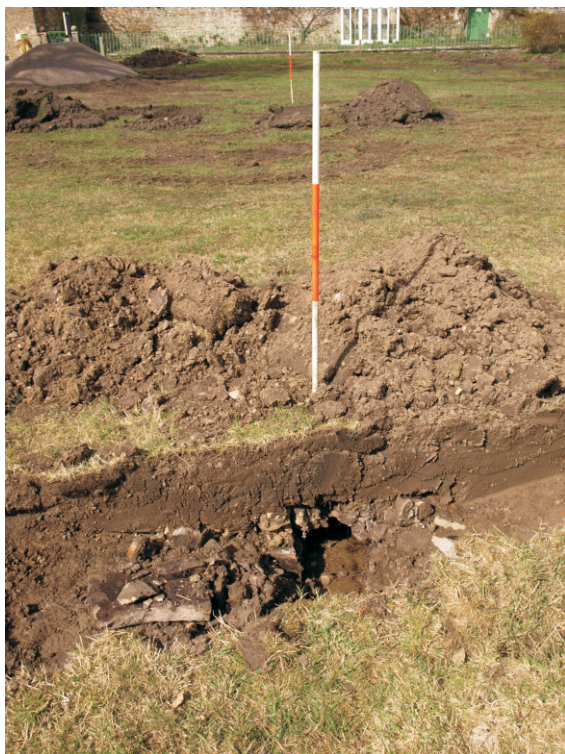
Image 180 Culvert 020 exposed in Trench E, looking N.
