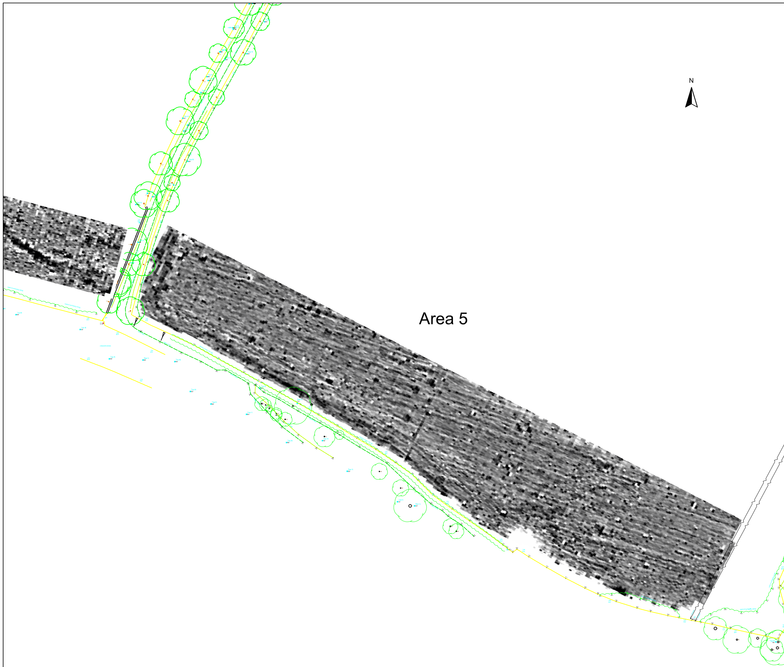
Greyscale plot of processed magnetometer data - Area 5
