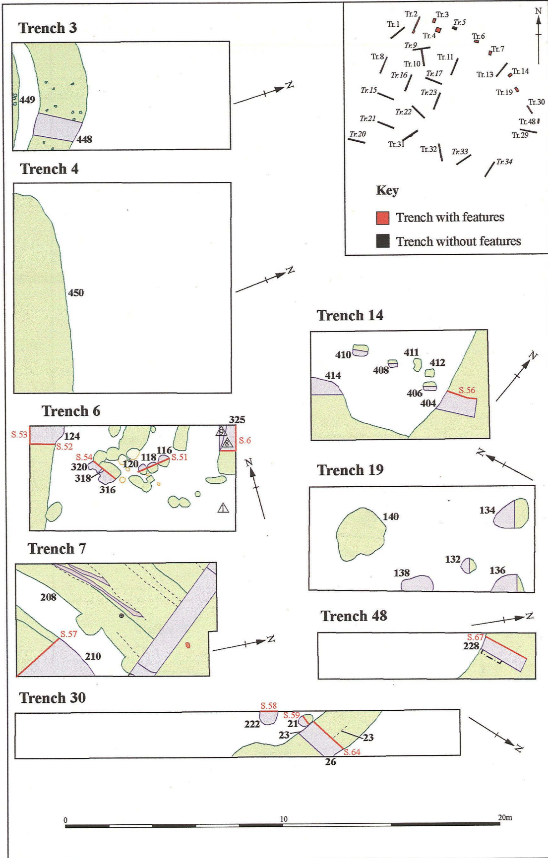
Figure 6: Trench plans
