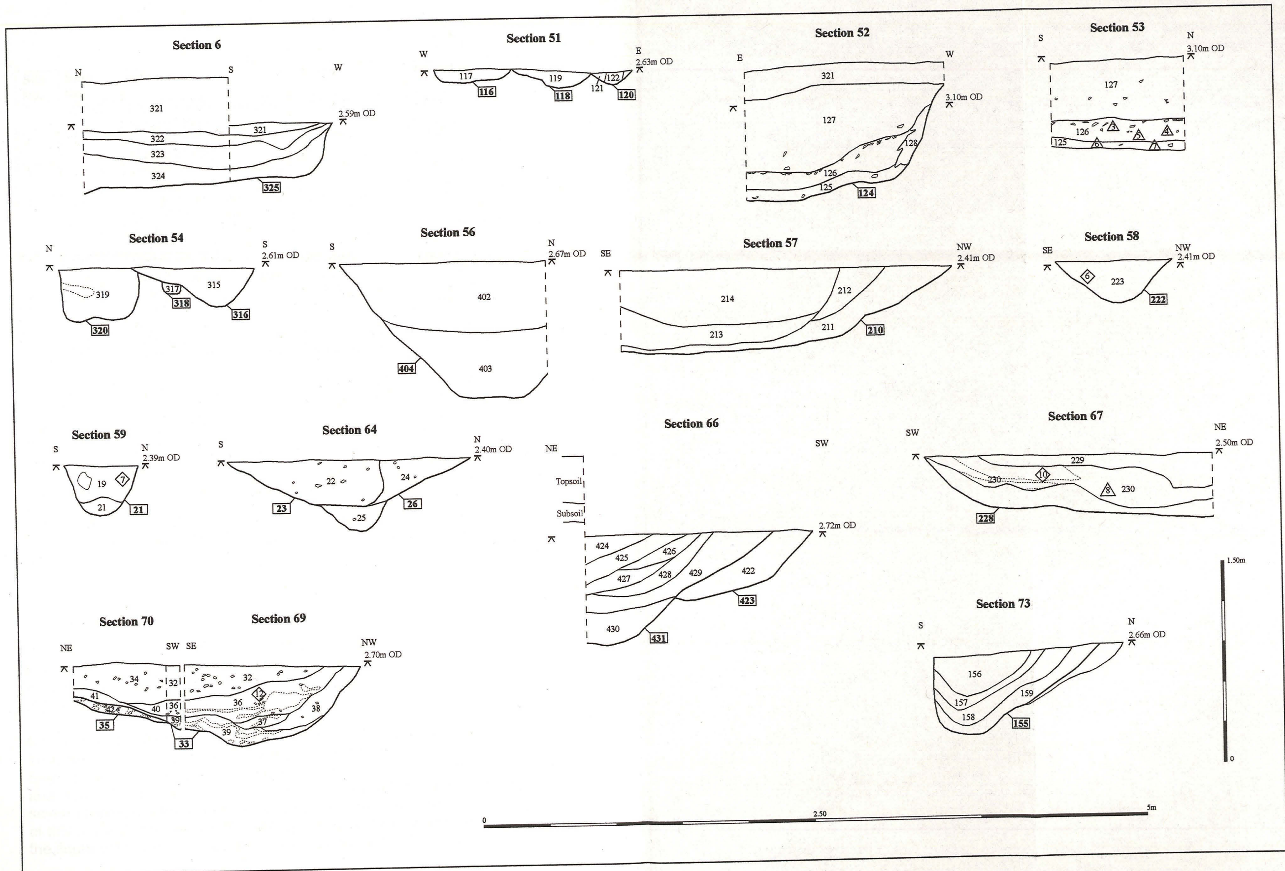
Figure 7: Section drawings
