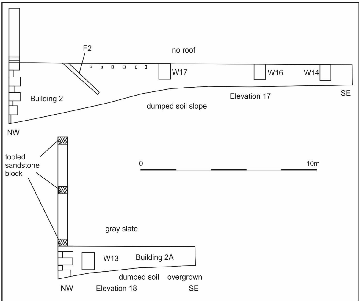
Illus 19 Building 2 elevation 17 and Building 2A elevation 18 annotated with numbers used in this survey
