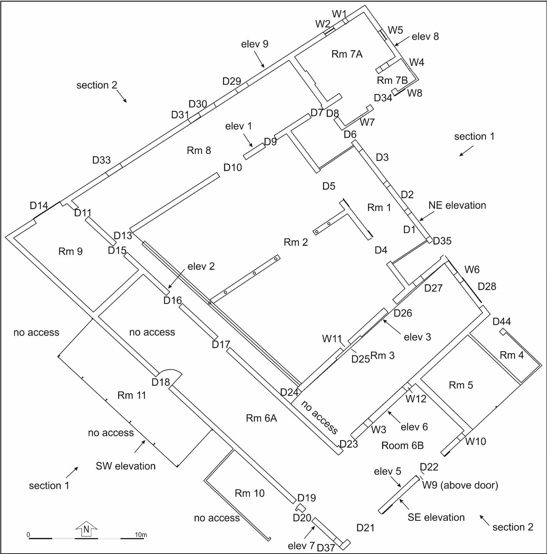
Illus 8 Building 1 annotated with numbers used in this survey including room, door, window, feature, elevation and section numbers (from copyright Bell Ingram Design)
