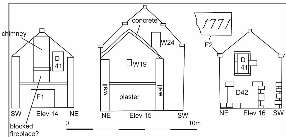
Illus 18 Building 2 elevations 14-16 annotated with numbers used in this survey
