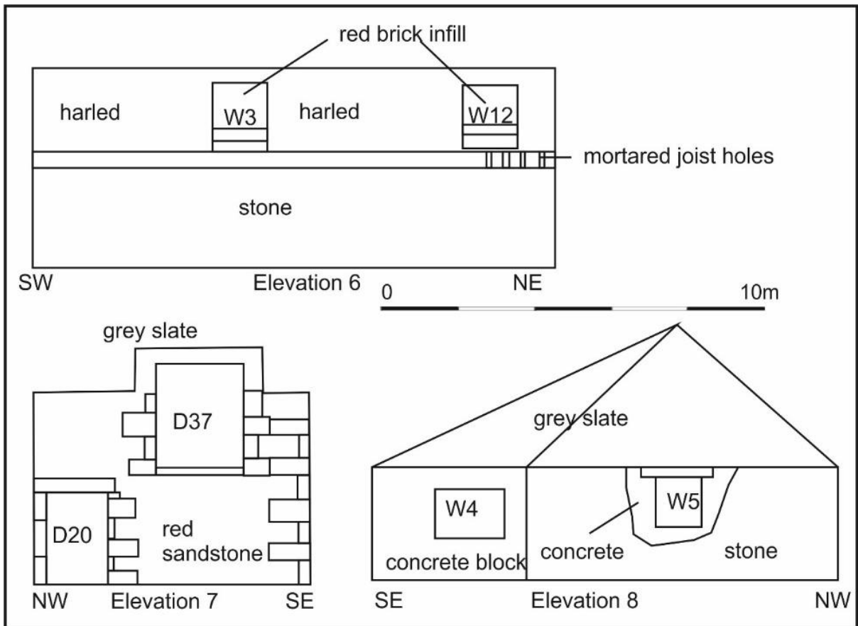
Illus 13 Building 1 elevations 6-8 annotated with numbers used in this survey
