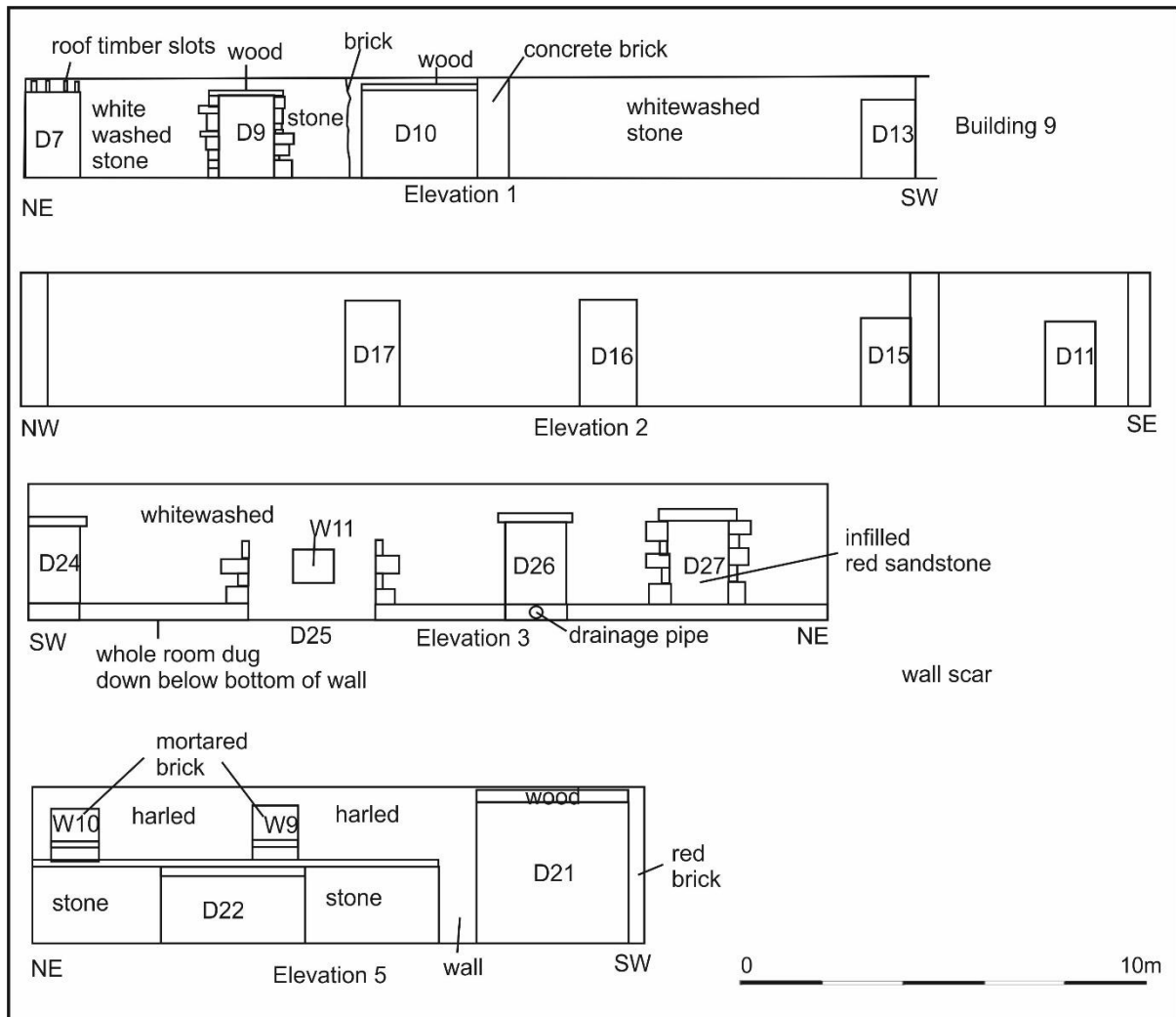
Illus 12 Building 1 elevations 1, 2, 3 and 5 annotated with numbers used in this survey
