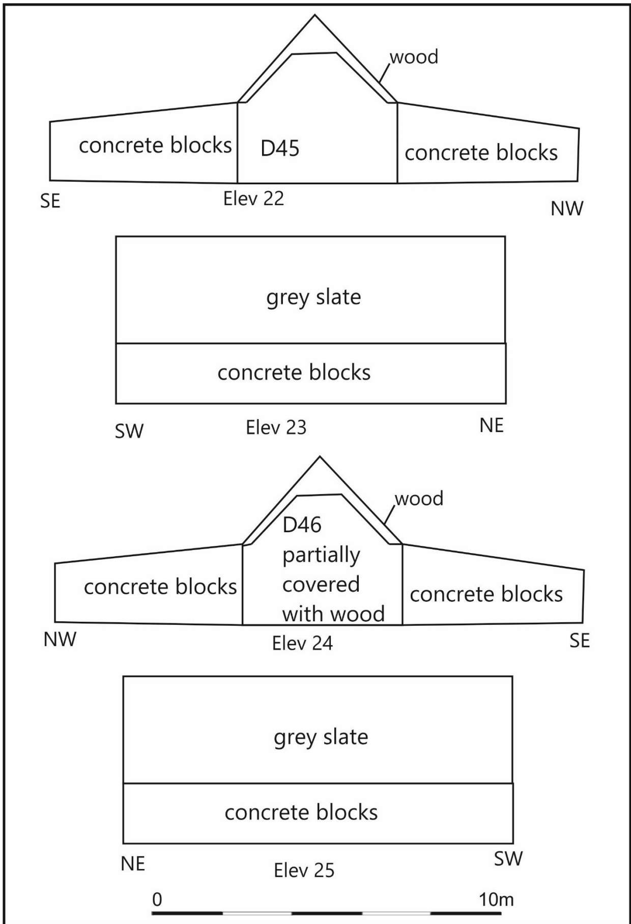
Illus 31 Building 4 elevations
