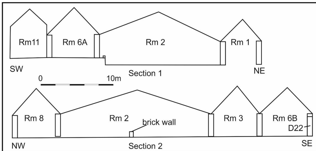
Illus 15 Sections 1 and 2
