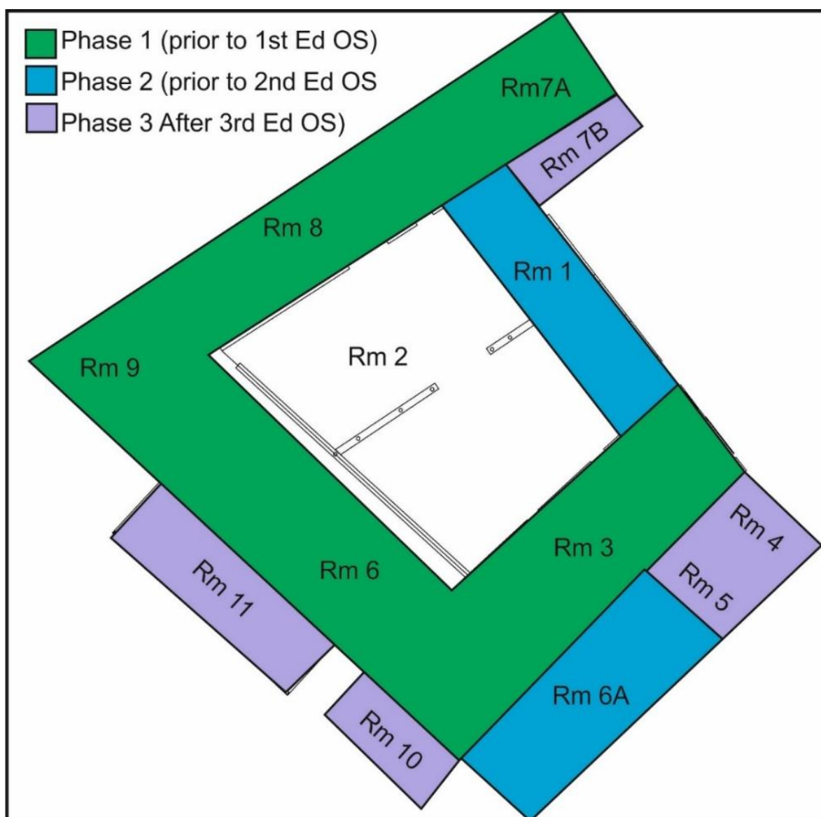
Illus 37 Building 1 phase plan
