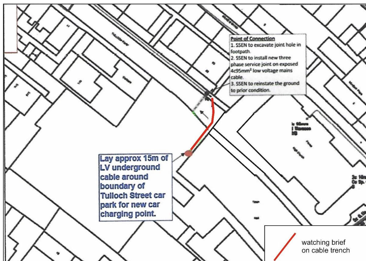
Illus 2 Site plan showing proposed development (copyright SSE)
