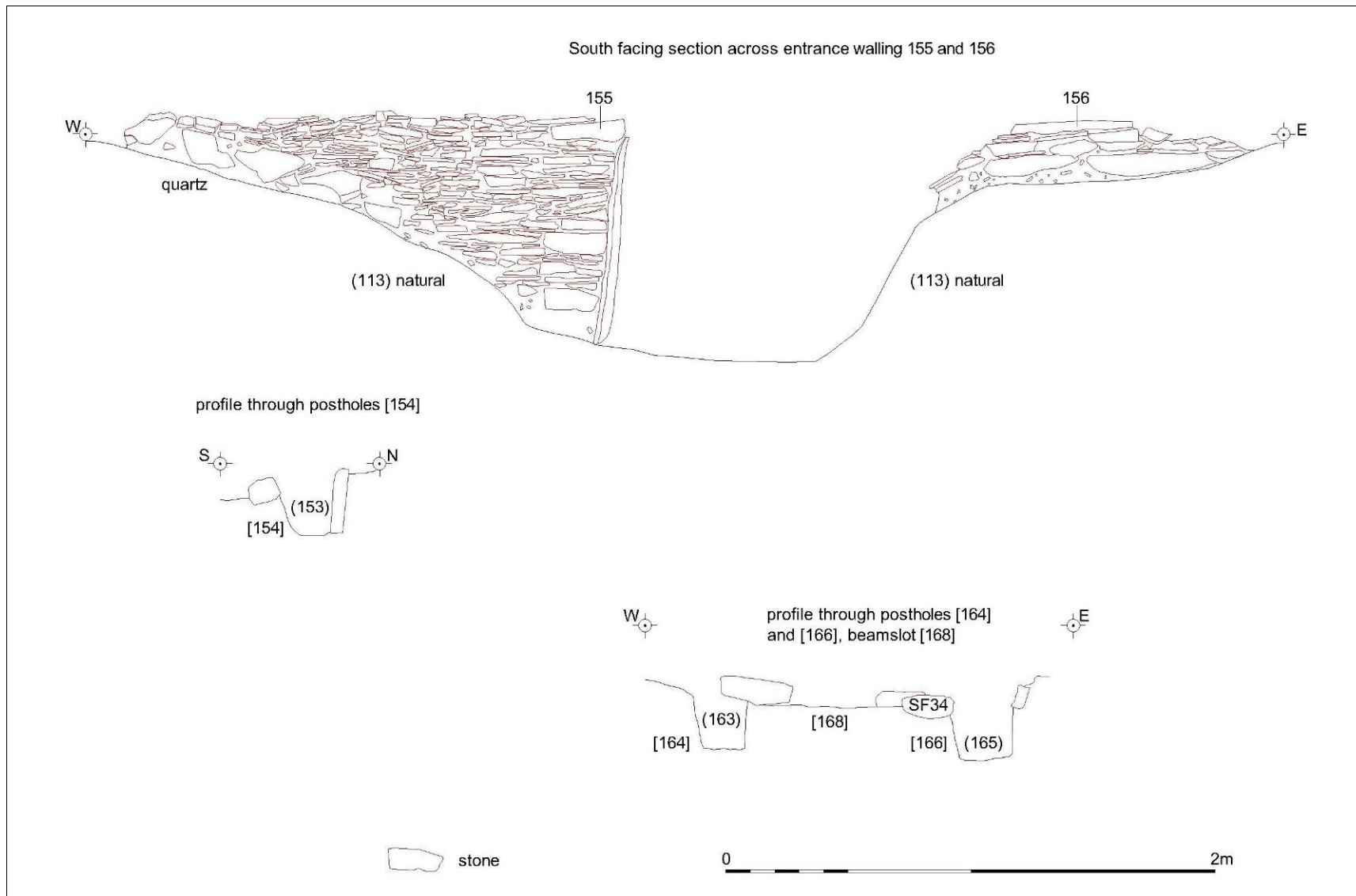
Fig 3 Elevation of entrance and revetment walls 155 and 156
