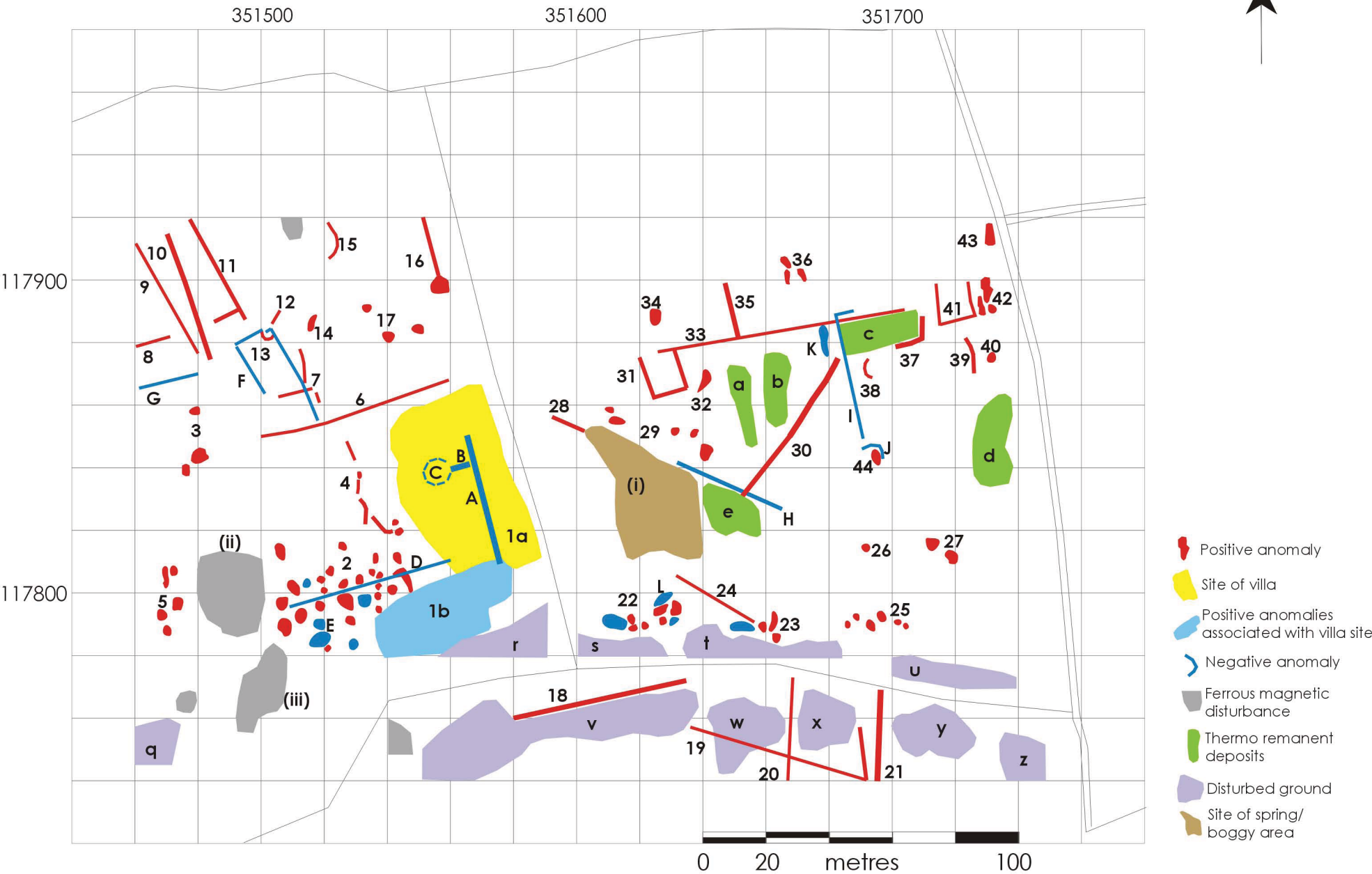
Figure 5: Gradiometry Interpretation
