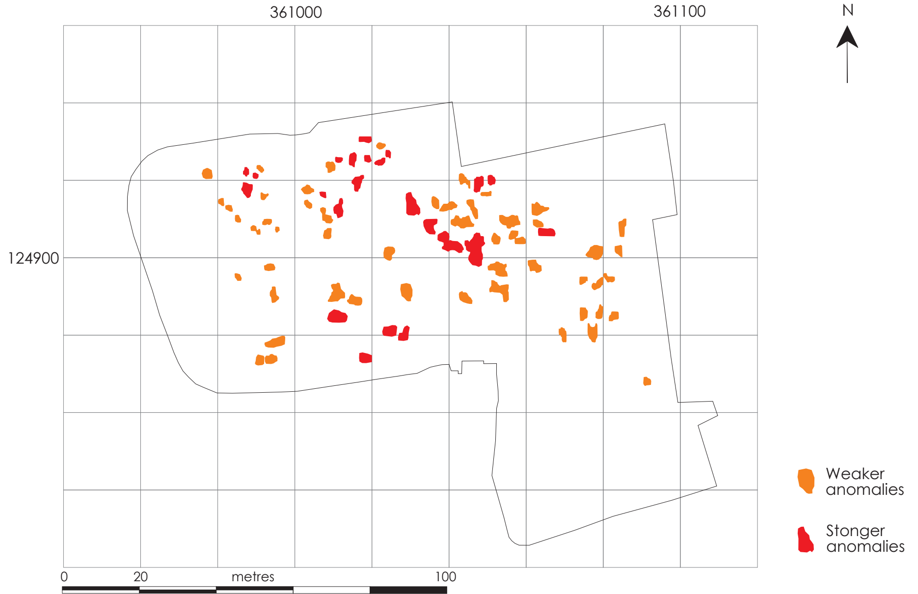
Figure 7: Non-linear anomalies
