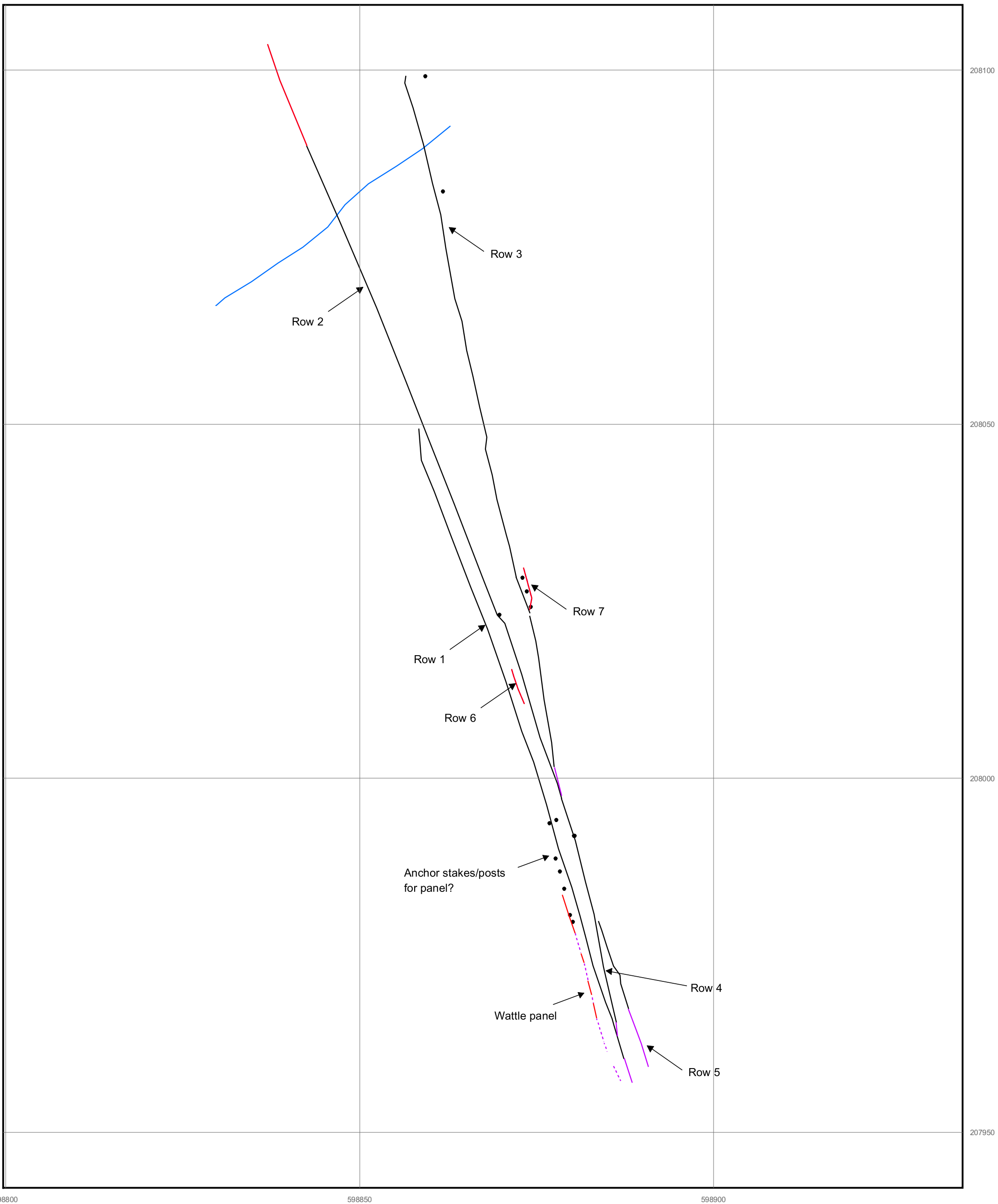
Pewet Island Fishtrap - Composite Plan
