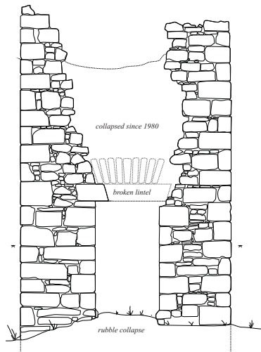
Drawing-14: engine house 2 west external elevation
