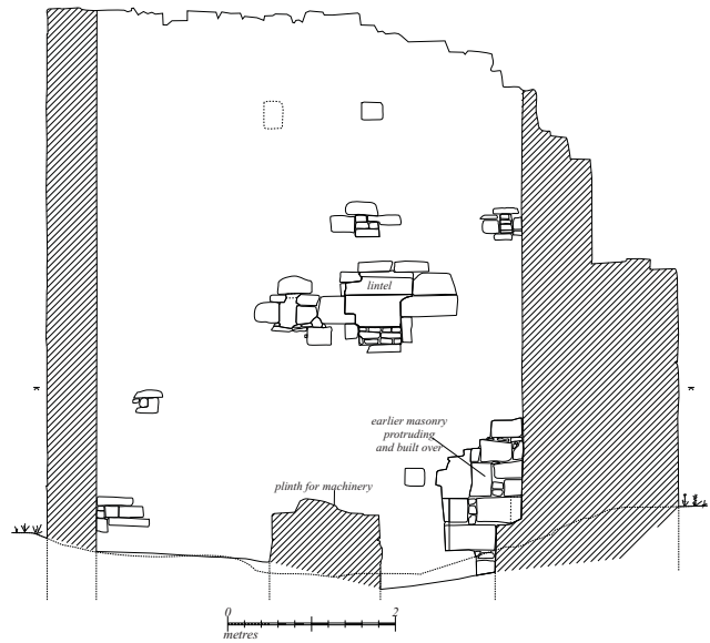
Drawing-15: engine house 2 north internal section
