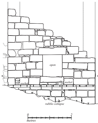
Drawing-03: Engine house 1 south external elevation
