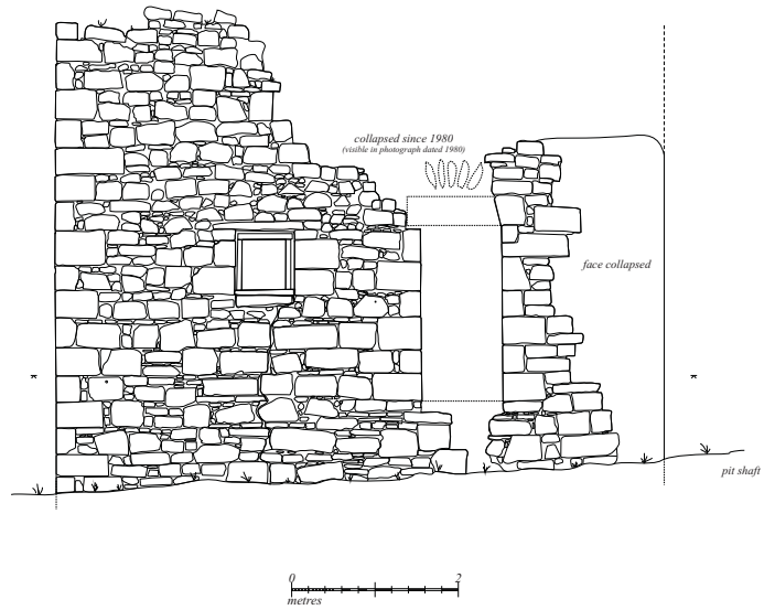
Drawing-11: engine house 2 south external elevation
