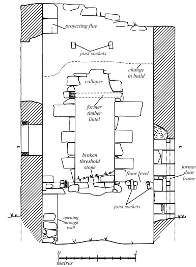
Drawing-06: engine house 1 north internal section
