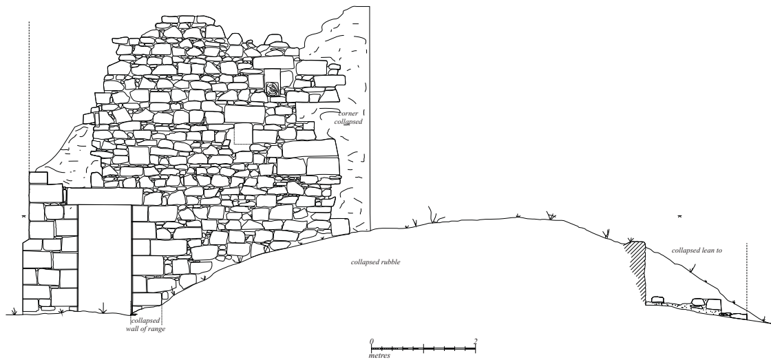
Drawing 4: Engine house 1 east external elevation
