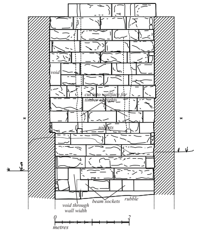
Drawing-18: engine house 2 east internal section
