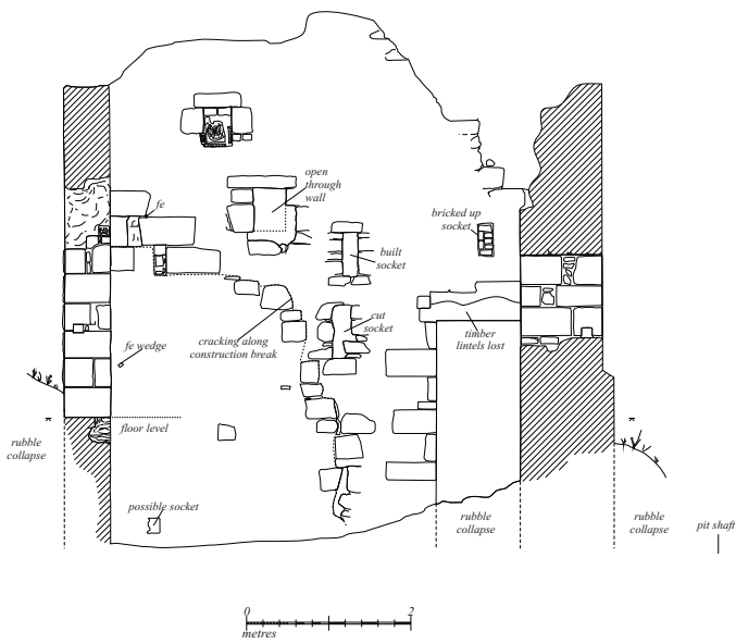
Drawing-07: engine house 1 east internal section
