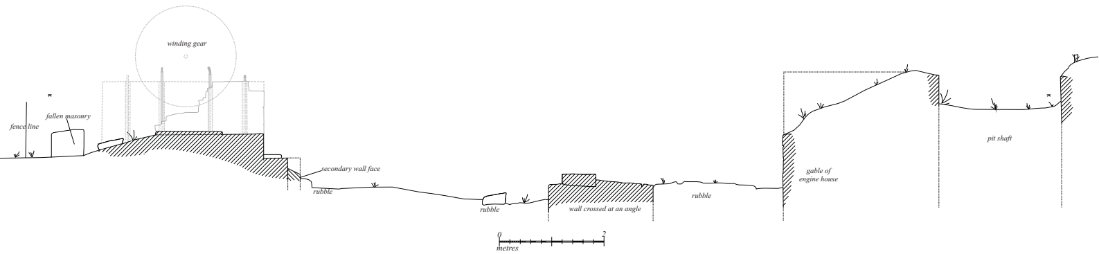
Drawing-24: section across site through winding gear and pit shaft
