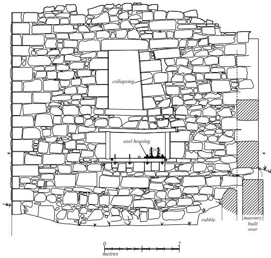
Drawing-10: engine house 1 west external elevation
