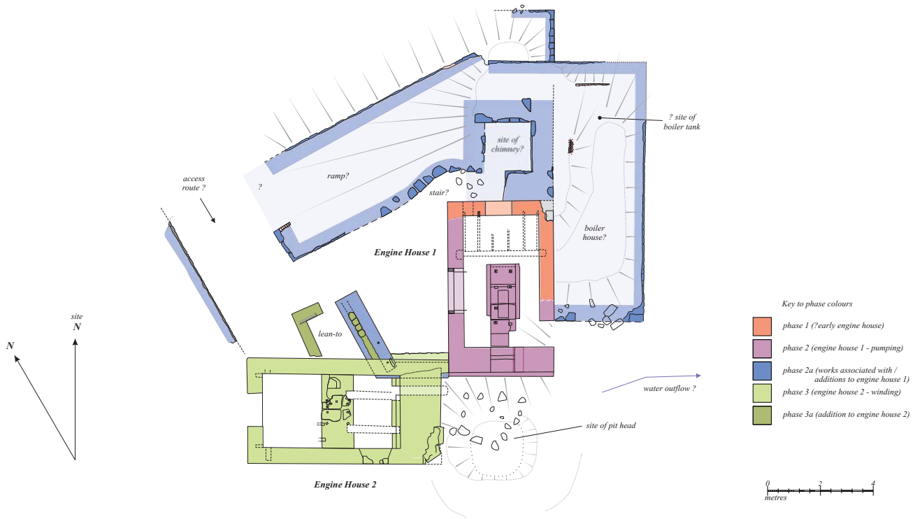
Moss Pit Engine Houses: Elevation locations
