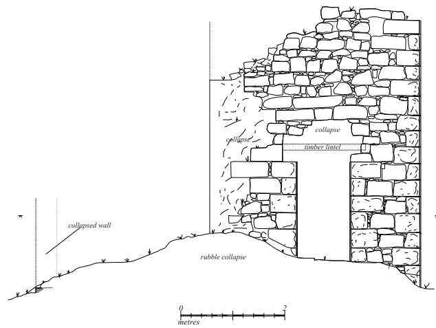
Drawing-05: Engine house 1 north external elevation
