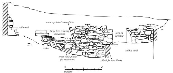
Drawing-21: west internal section
