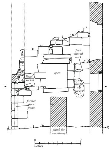
Drawing-08: engine house 1 south internal section
