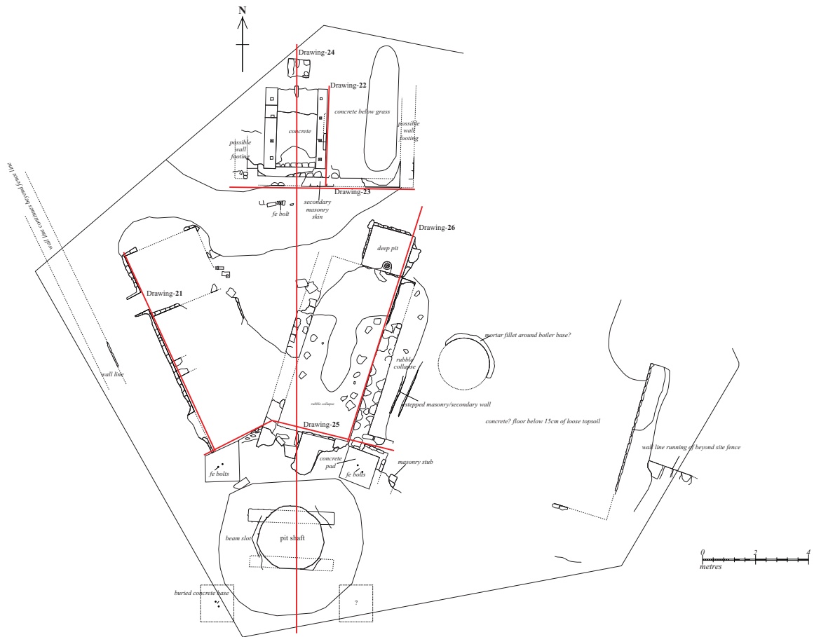
Temple Pit: Plan and elevation locations
