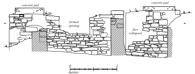
Drawing-25: south interior section across engine house
