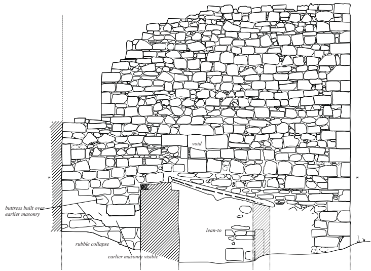
Drawing-13: engine house 2 north external elevation
