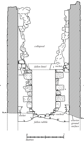
Drawing-17: engine house 2 west internal section
