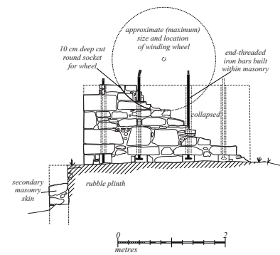
Drawing-22: winding gear elevation
