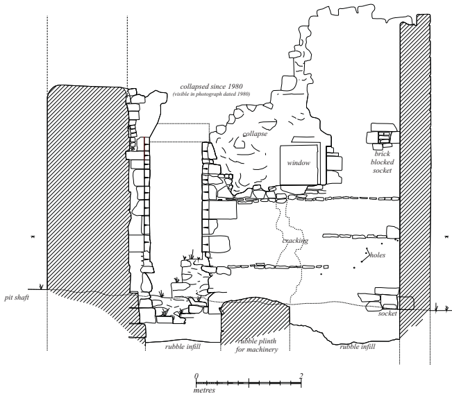
Drawing-16: engine house 2 south internal section
