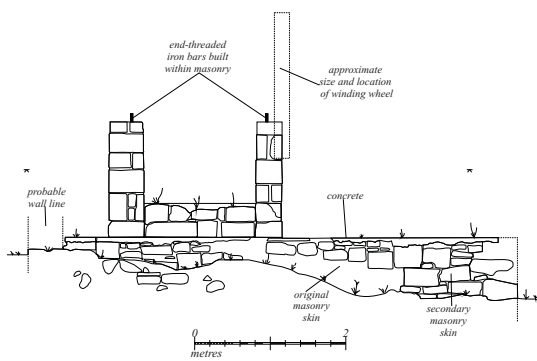
Drawing-23: winding gear front elevation
