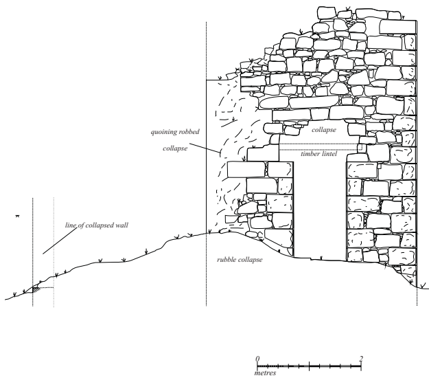
Drawing-05: engine house 1 north external elevation
