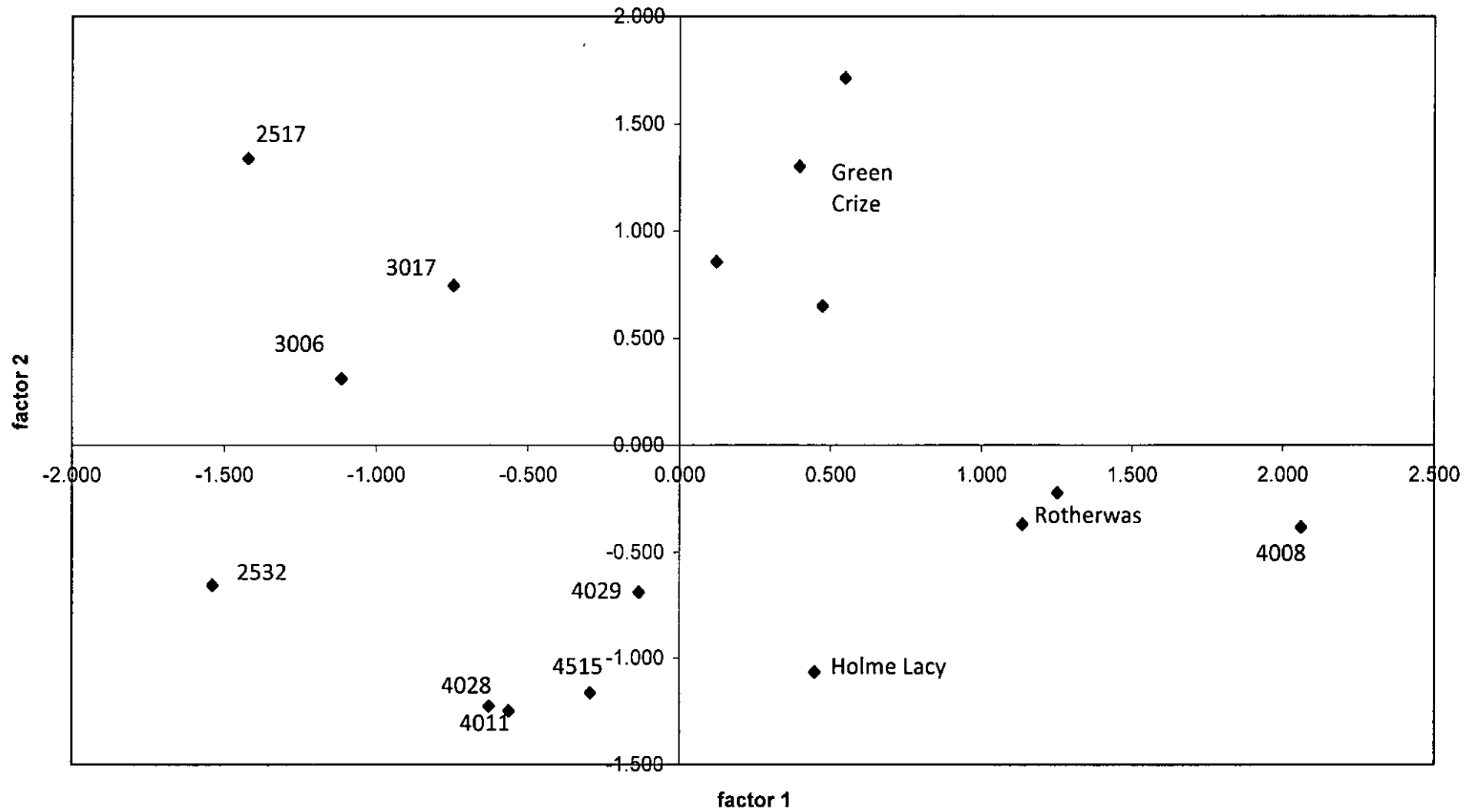
casewise factor scores: finer fraction
