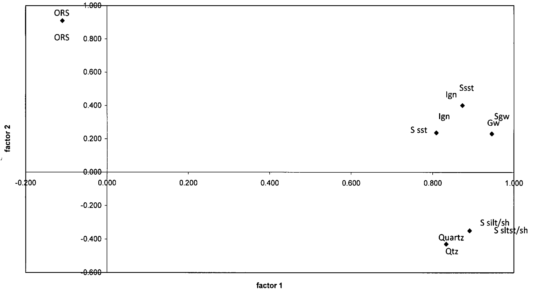
Unrotated factor loadings: coarser fraction
