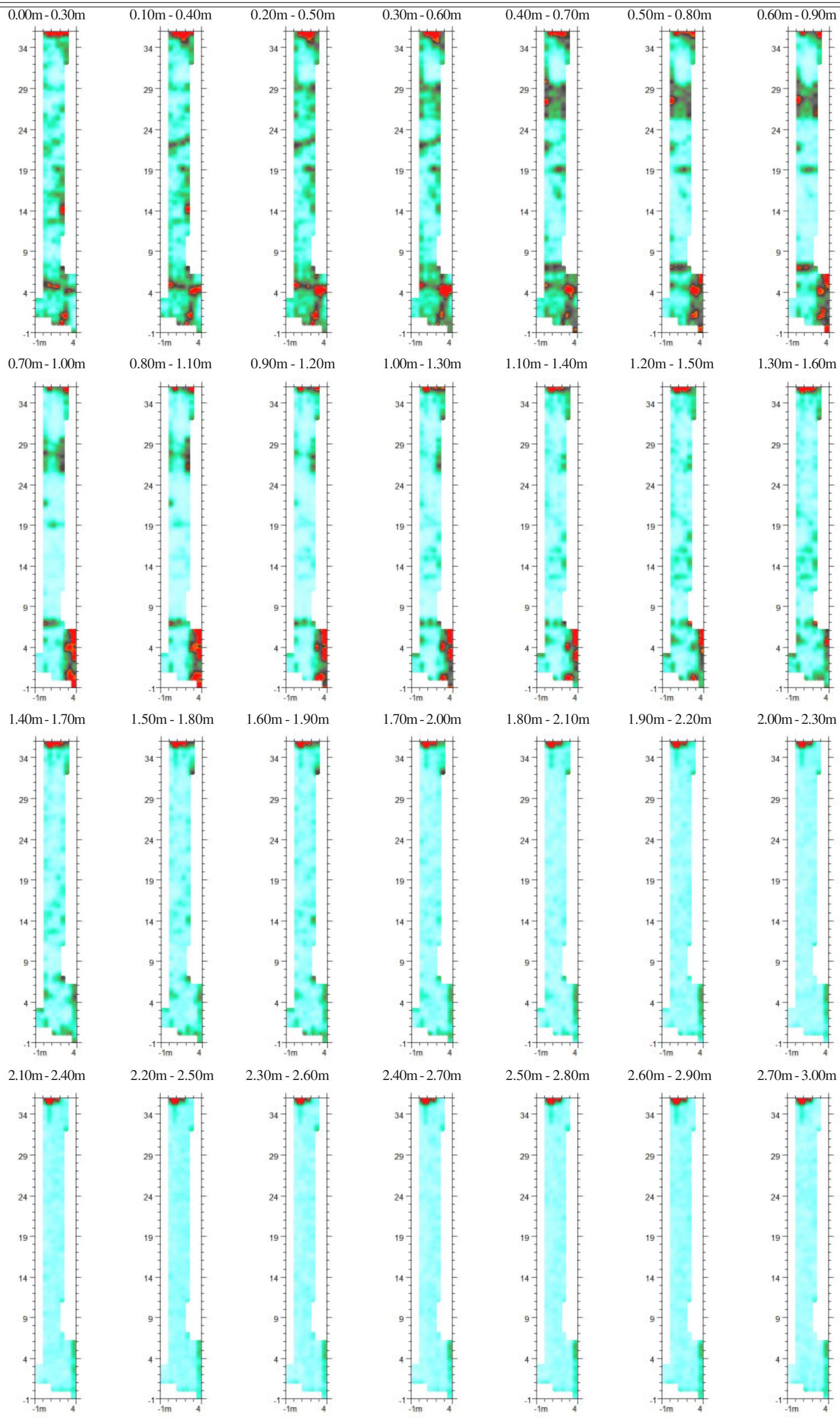
GSB PROSPECTION Ltd. 2009/09 Glastonbury Abbey GPR Filtered Data - Area IVD Figure G85
