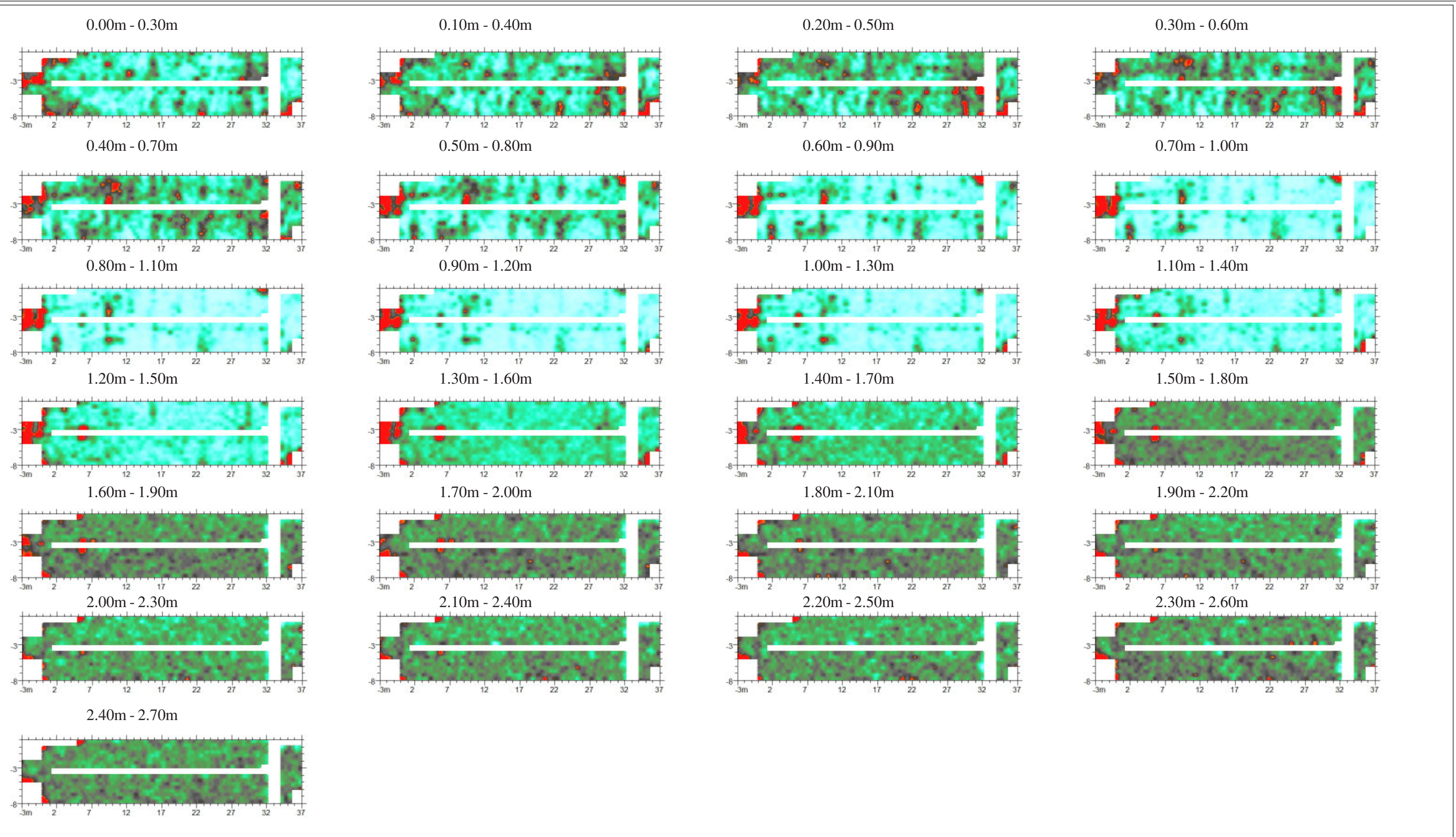
GSB PROSPECTION Ltd. 2009/09 Glastonbury Abbey GPR Filtered Data - Area IVF Figure G89
