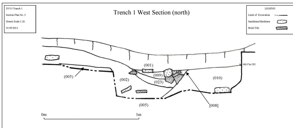
Figure 9: Section plan detailing the fill of foundation cut [008]
