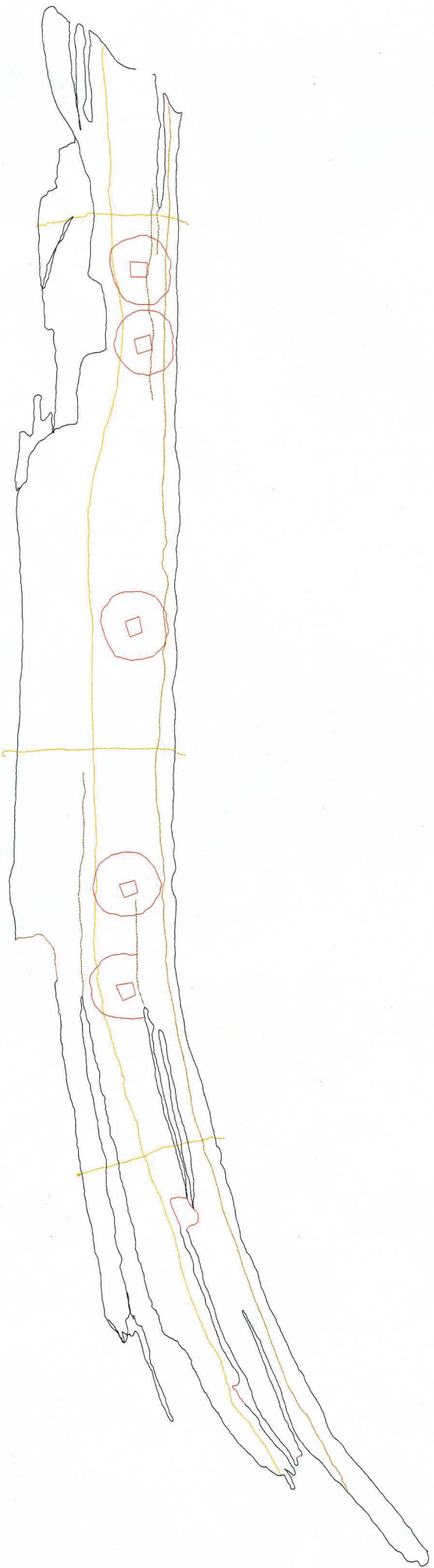
395 Portside Lower Edge Plank Fragment Lise B Brekmoe 18 September 2006
