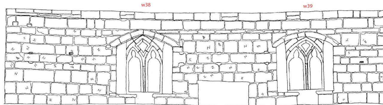
West Wall
