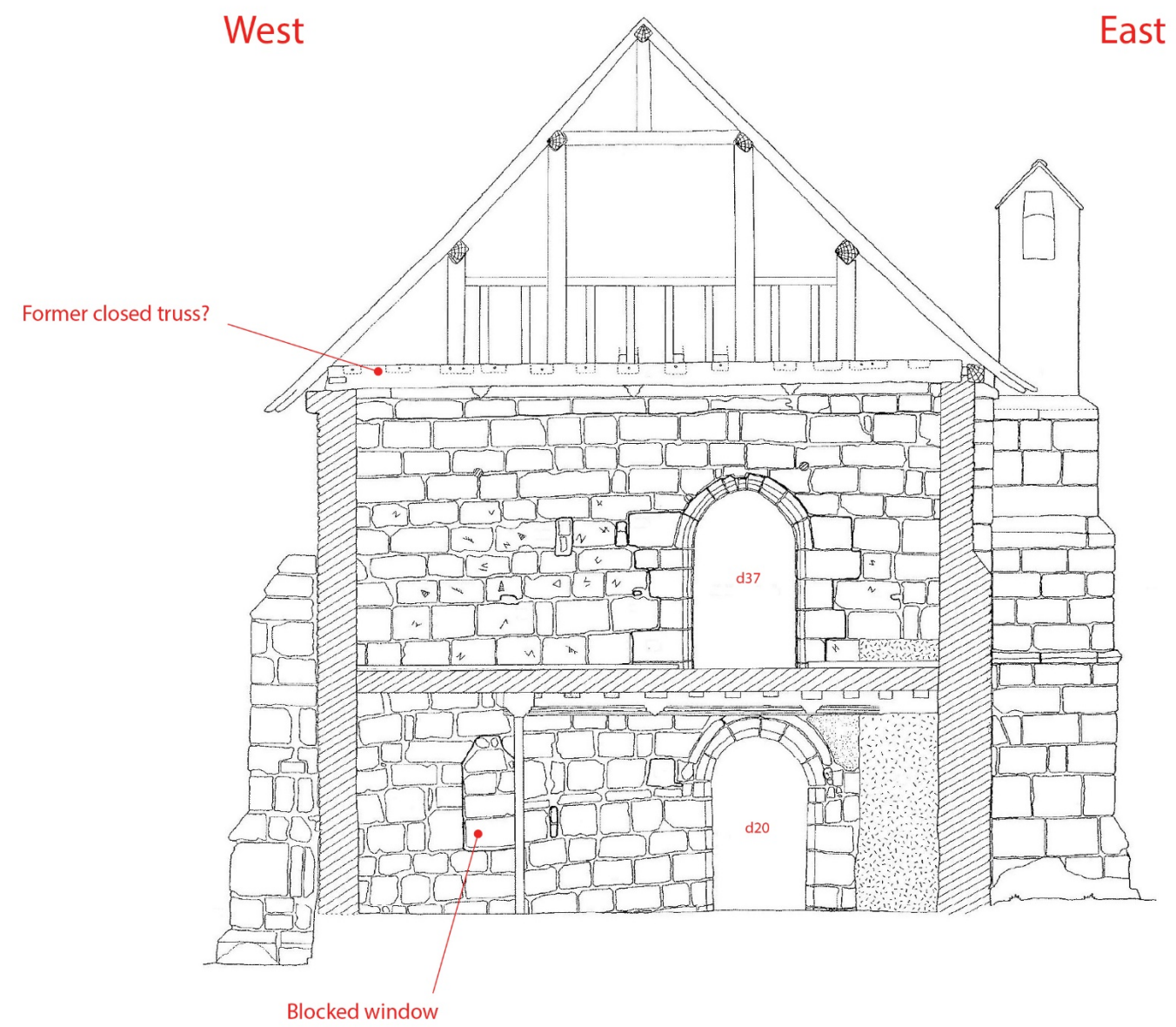
South Elevation
