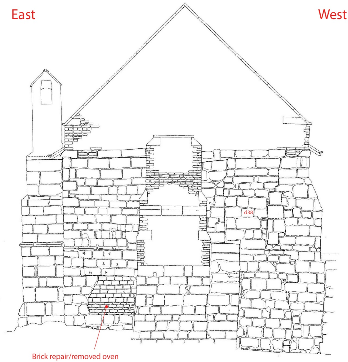
North Elevation
