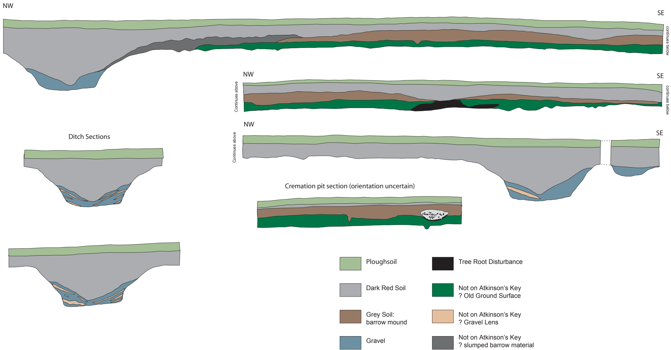
Figure 8: Netherhills Site 1 Sections (redrawn from Atkinson original)
