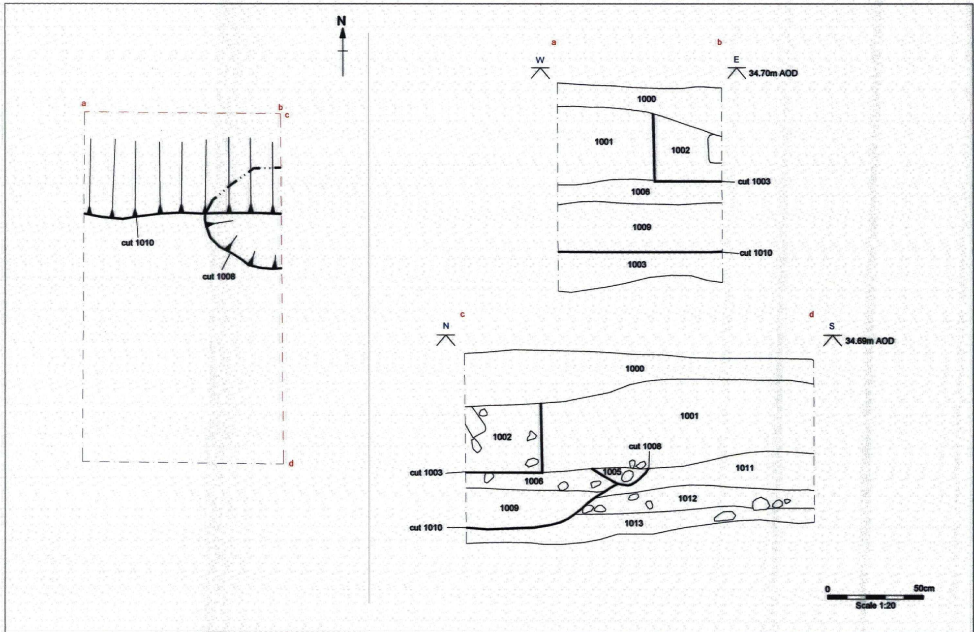
Figure 3. Evaluation Trench 1: Plan and Sections
