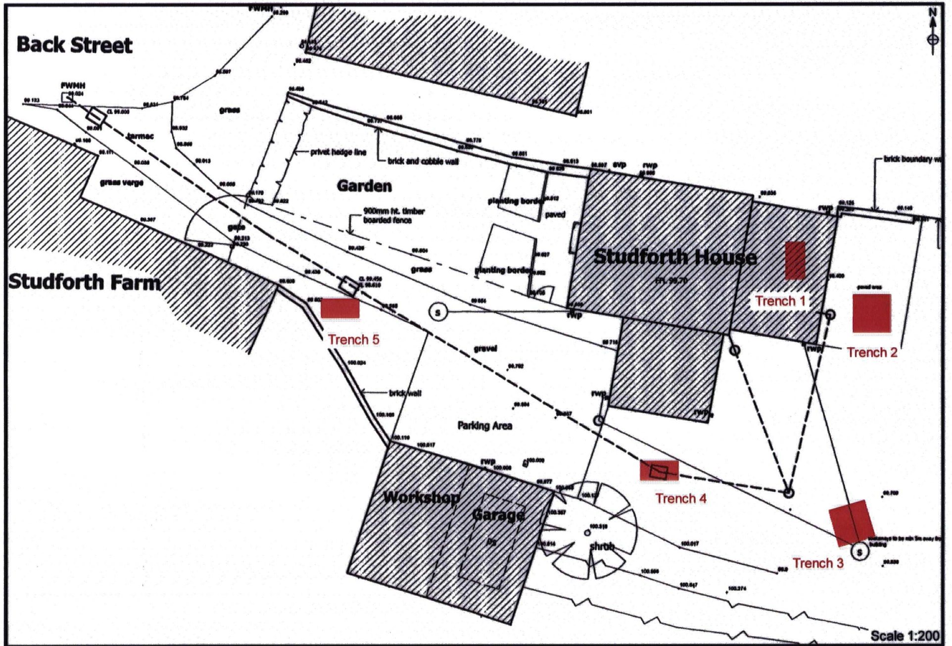
Figure 2. Evaluation Trench Location
