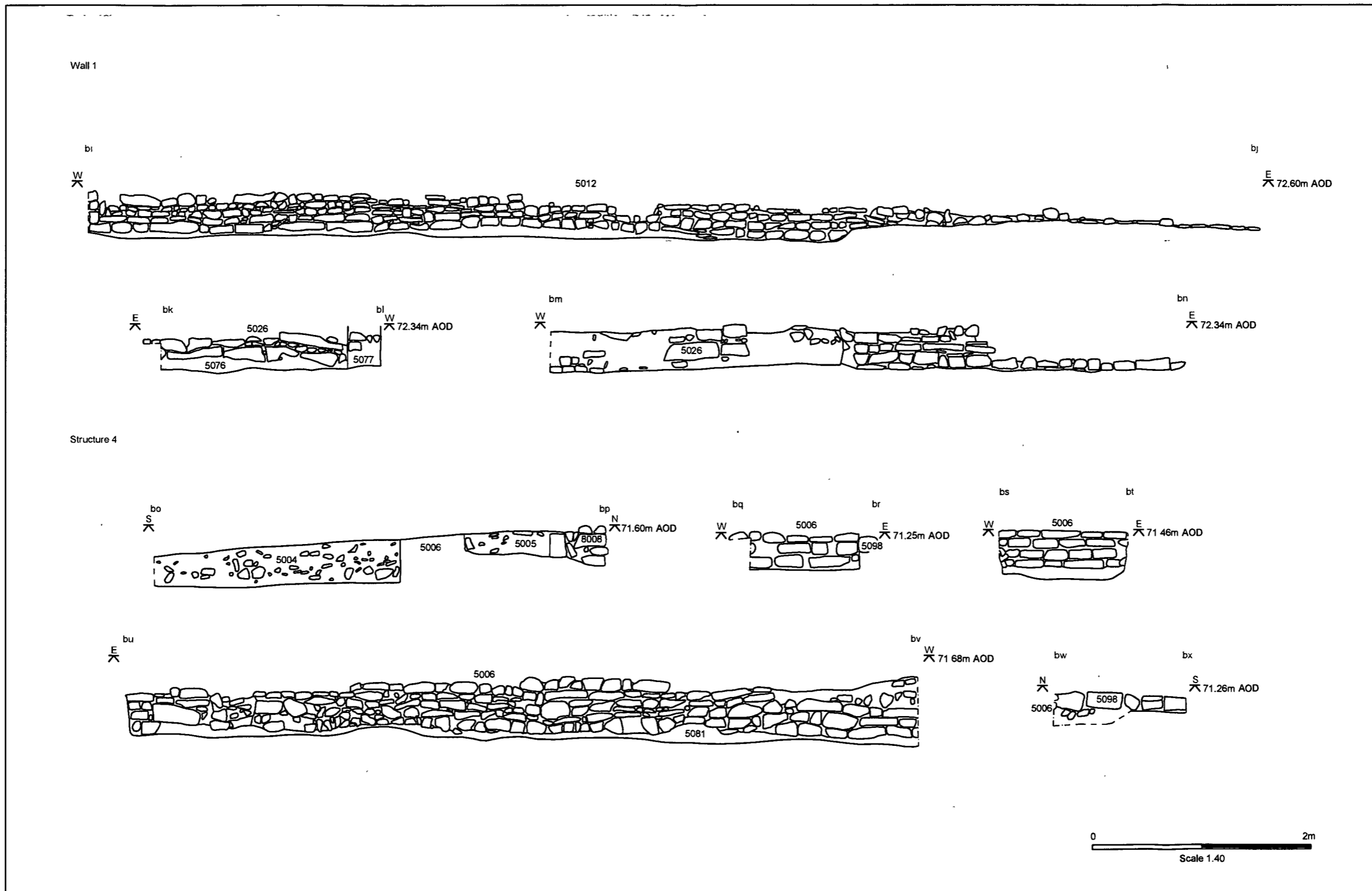
Figure 8. Period 4. Wall 1 and Structure 4 Elevations
