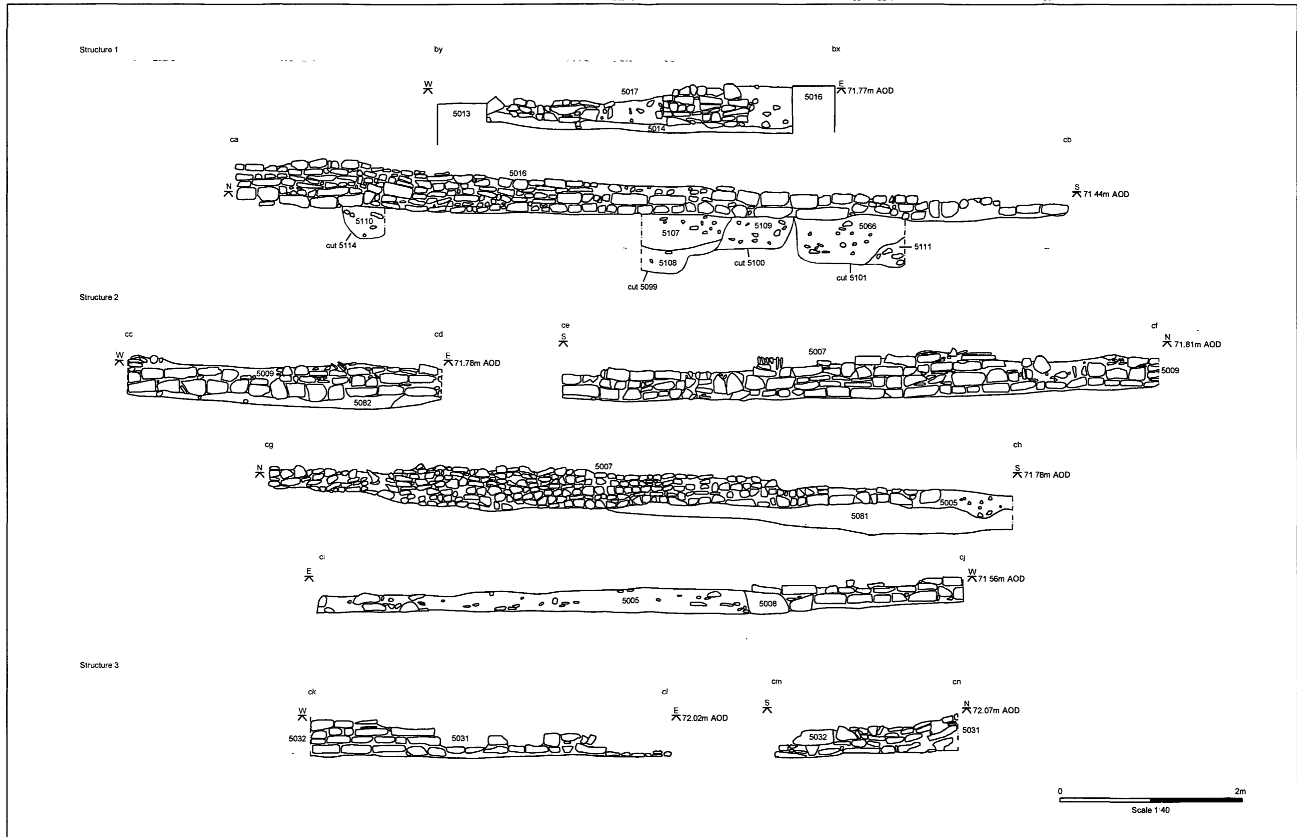
Figure 9. Period 4. Structures 1-3 Elevations
