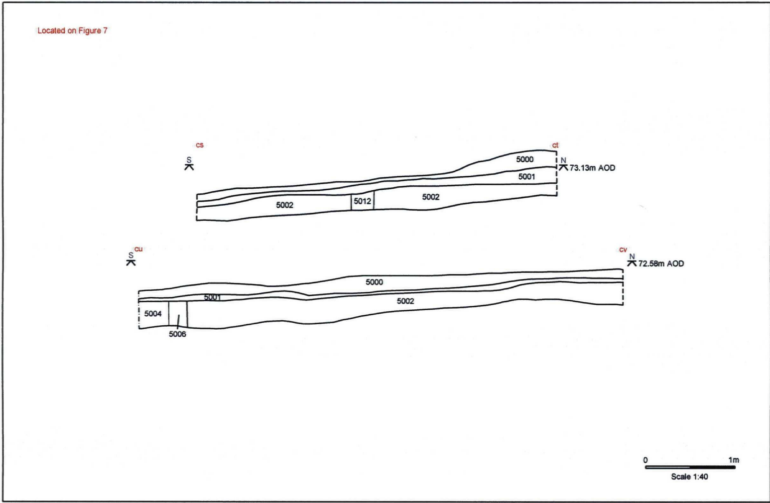
Figure 13. Period 6 Sections
