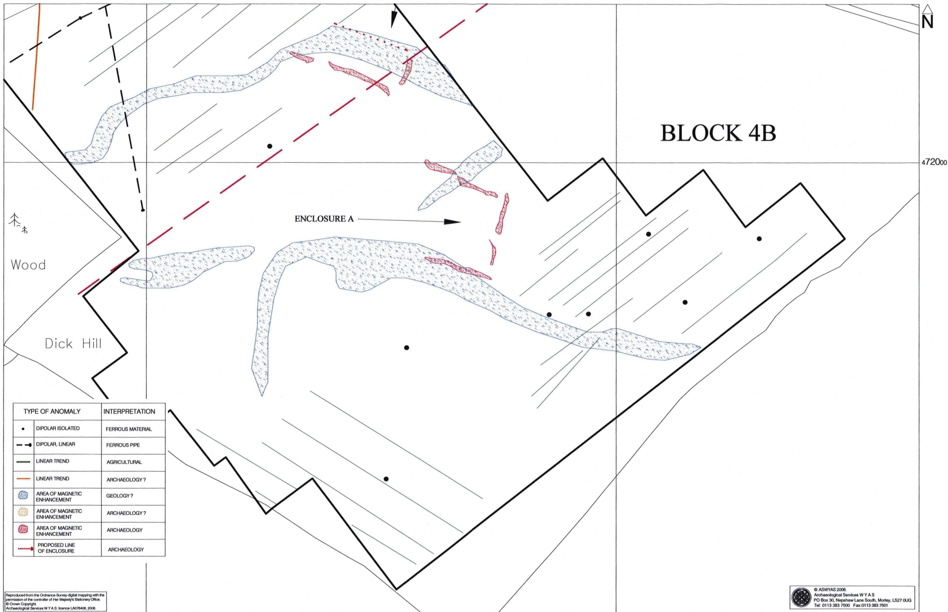
Fig. 23. Interpretation of magnetometer data: Block 4B (1:1000 @ A3)
