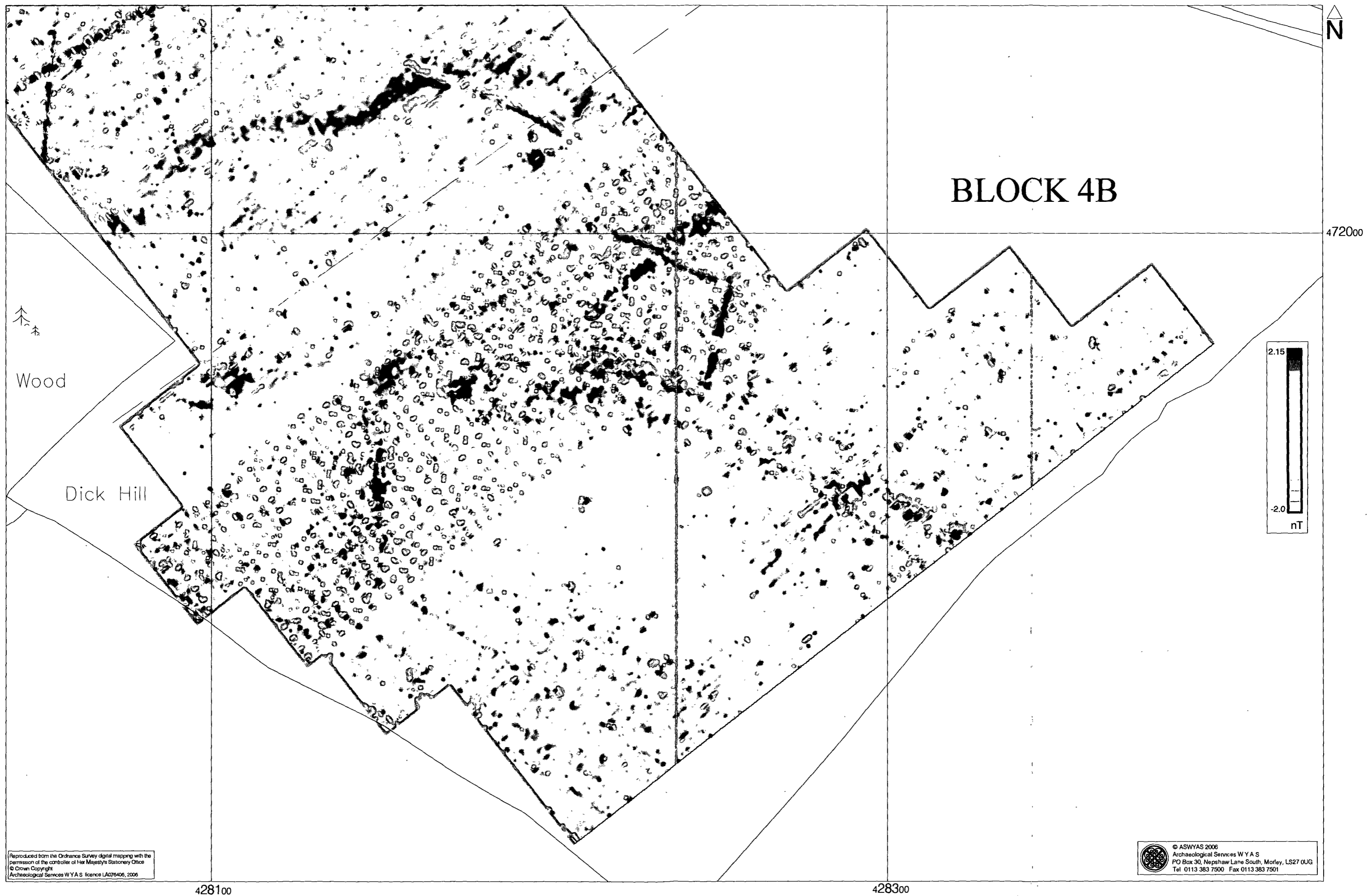
Fig. 22. Processed greyscale magnetometer data: Block 4B (1:1000 @ A3)
