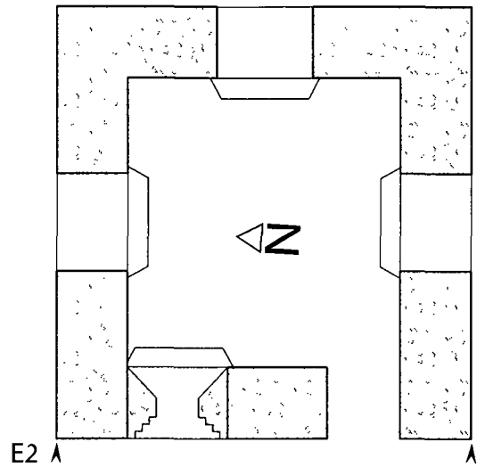
Figure 22b plan of Pill box 2
