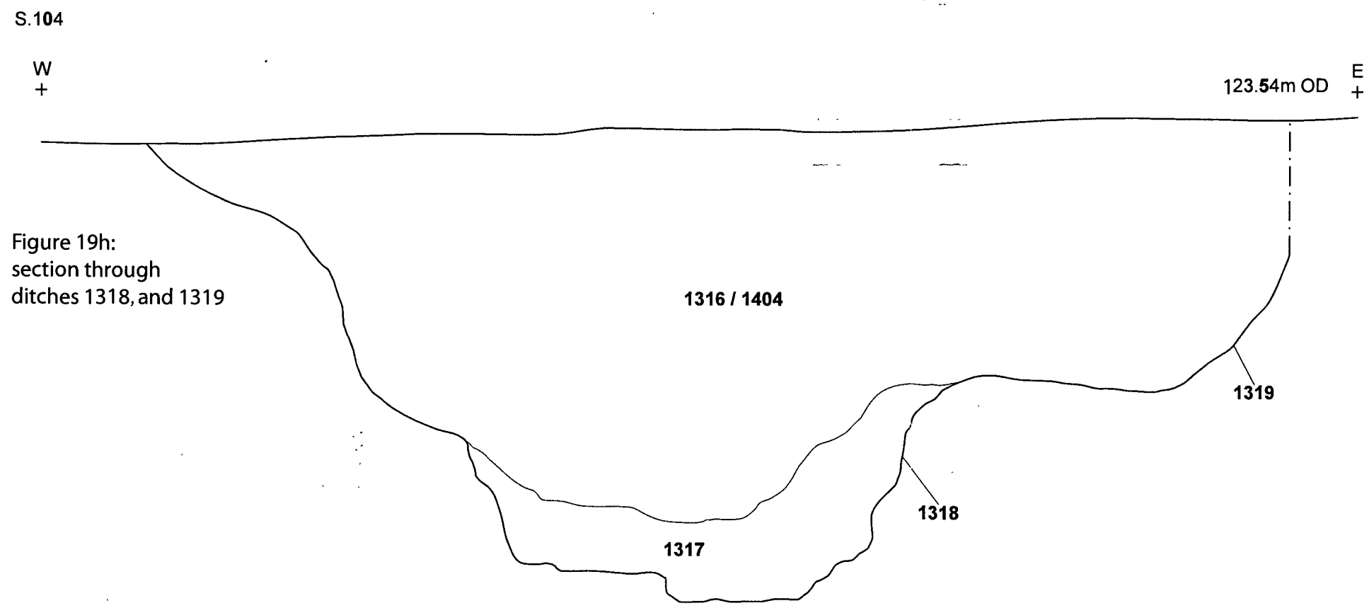
Fig. 19. Area C sections 96, 97, 98, 99, 100, 101, 102 and 104 (scale 1:20)
