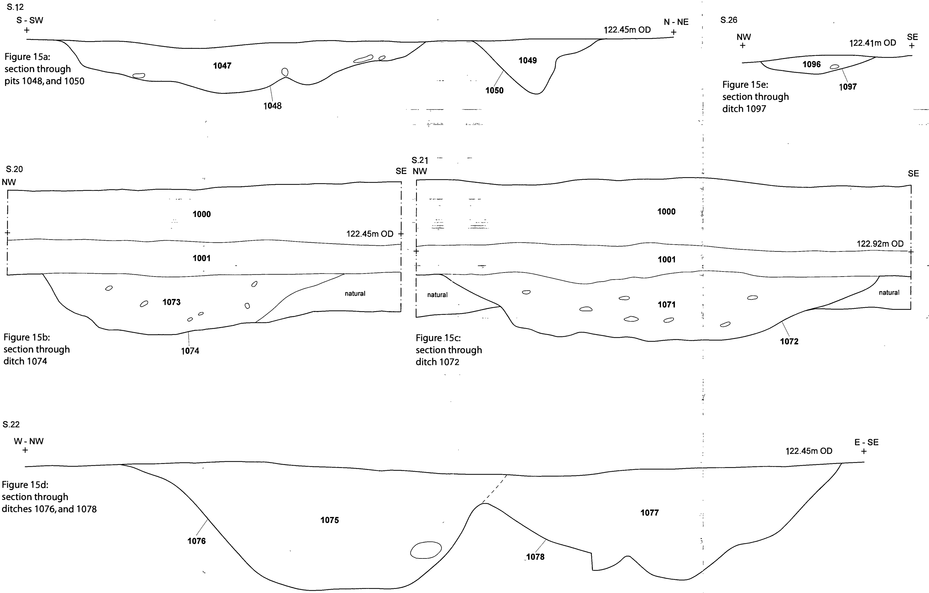
Fig. 15. Area B sections 12, 20, 21, 22 and 26 (scale 1: 10)
