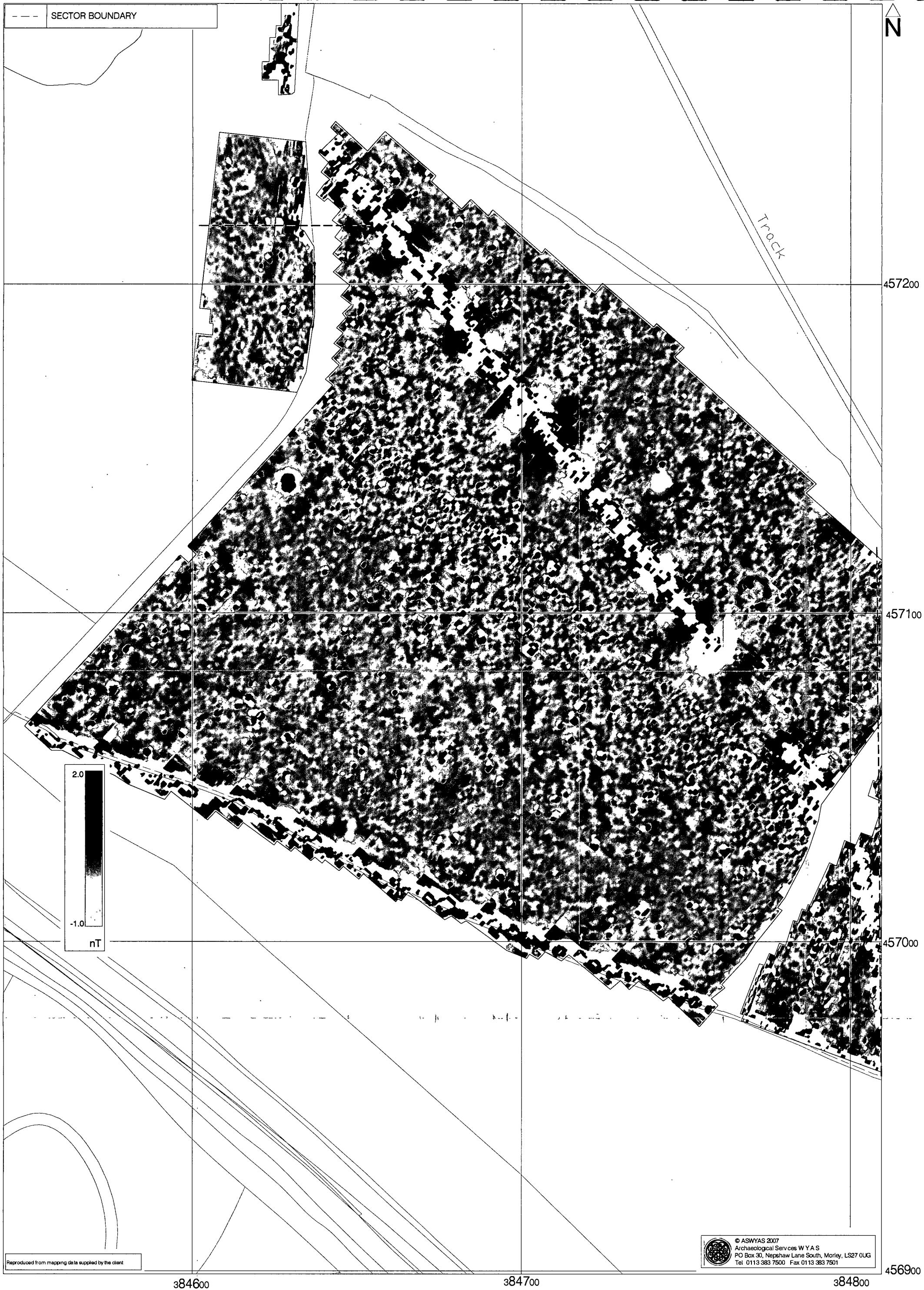
Fig. 9. Processed greyscale magnetometer data; environmental centre site - western sector (1:1000 @ A4)
