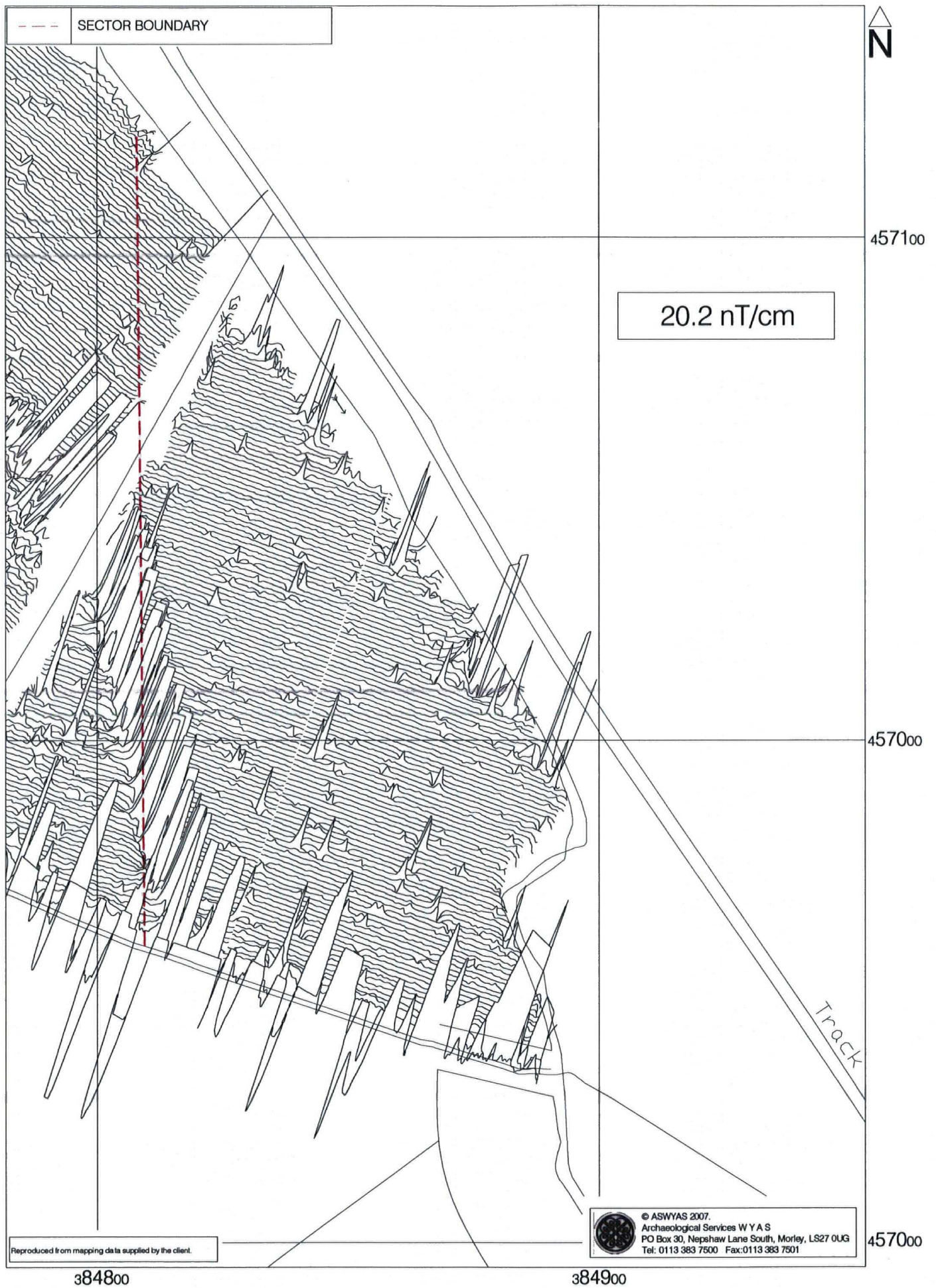
Fig. 13. XY trace plot of unprocessed magnetometer data; environmental centre site, east sector (1:1000 @ A4)
