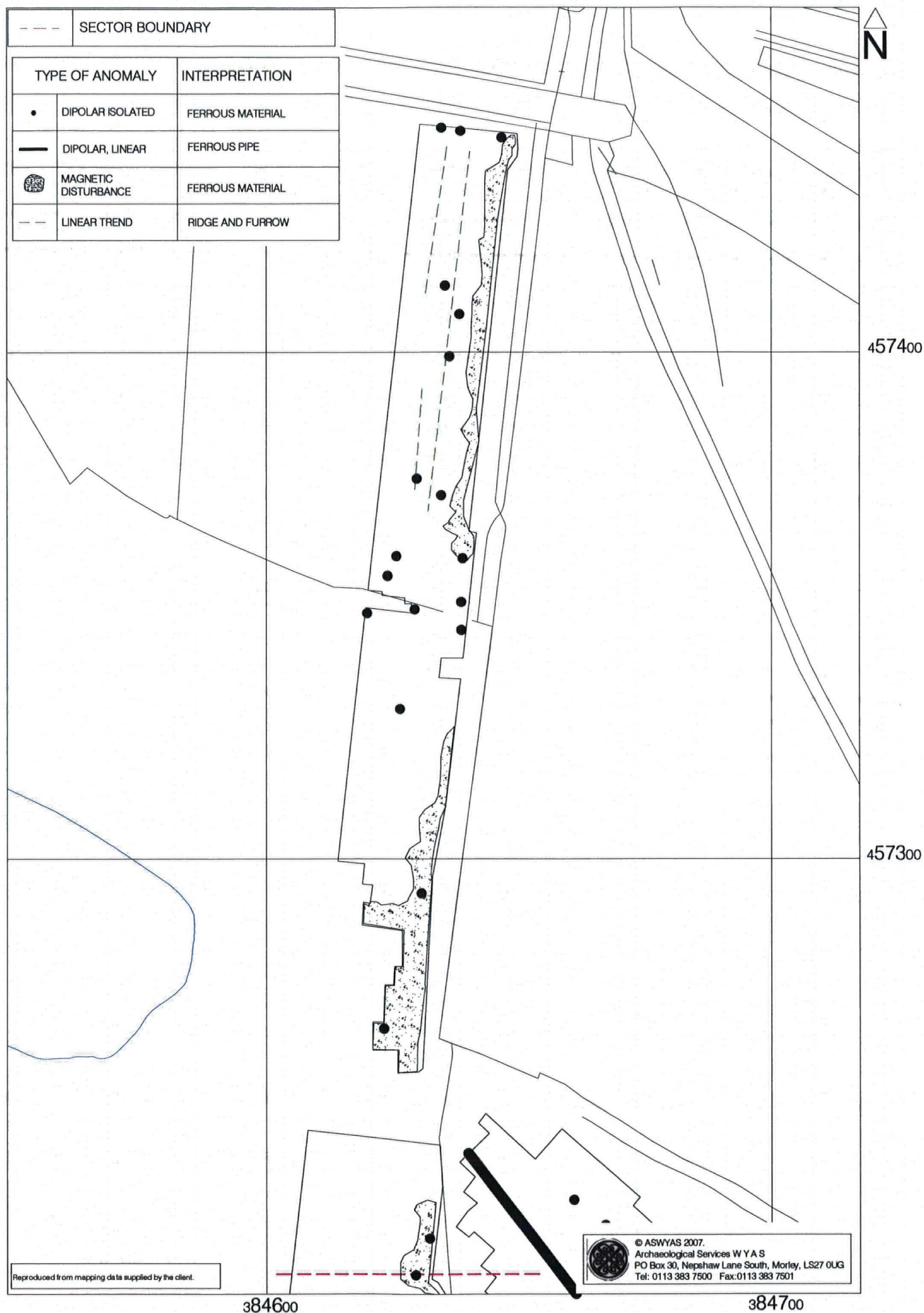
Fig. 8. Interpretation of magnetometer data; road corridor (1:1000 @ A4)
