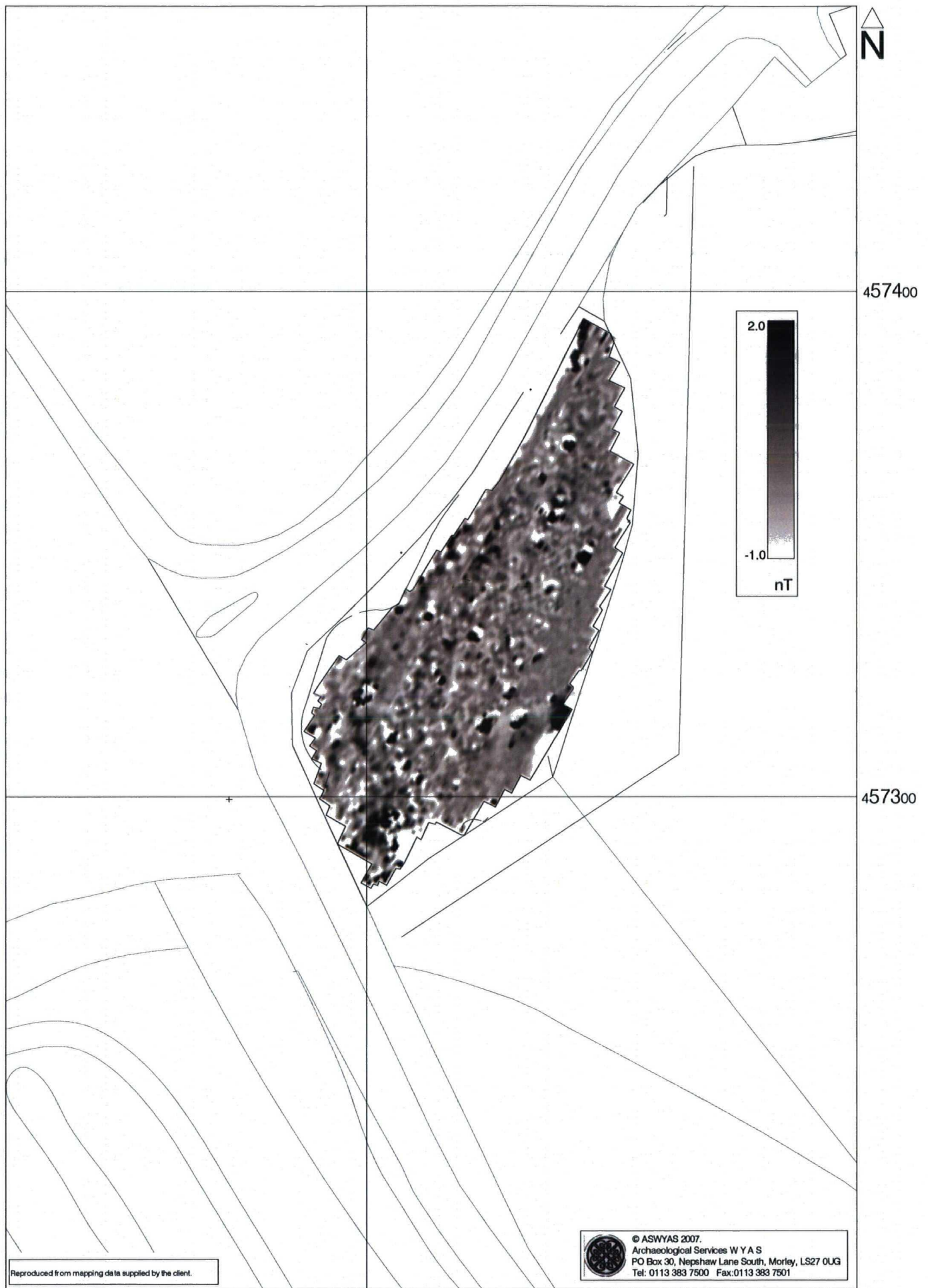
Fig. 3. Processed greyscale magnetometer data; hotel site (1:1000 @ A4)
