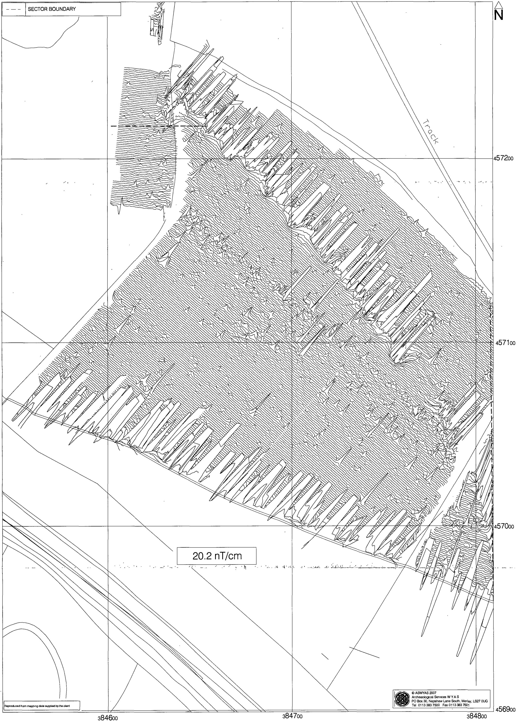
Fig. 10. XY trace plot of unprocessed magnetometer data; environmental centre site, western sector (1:1000 @ A4)
