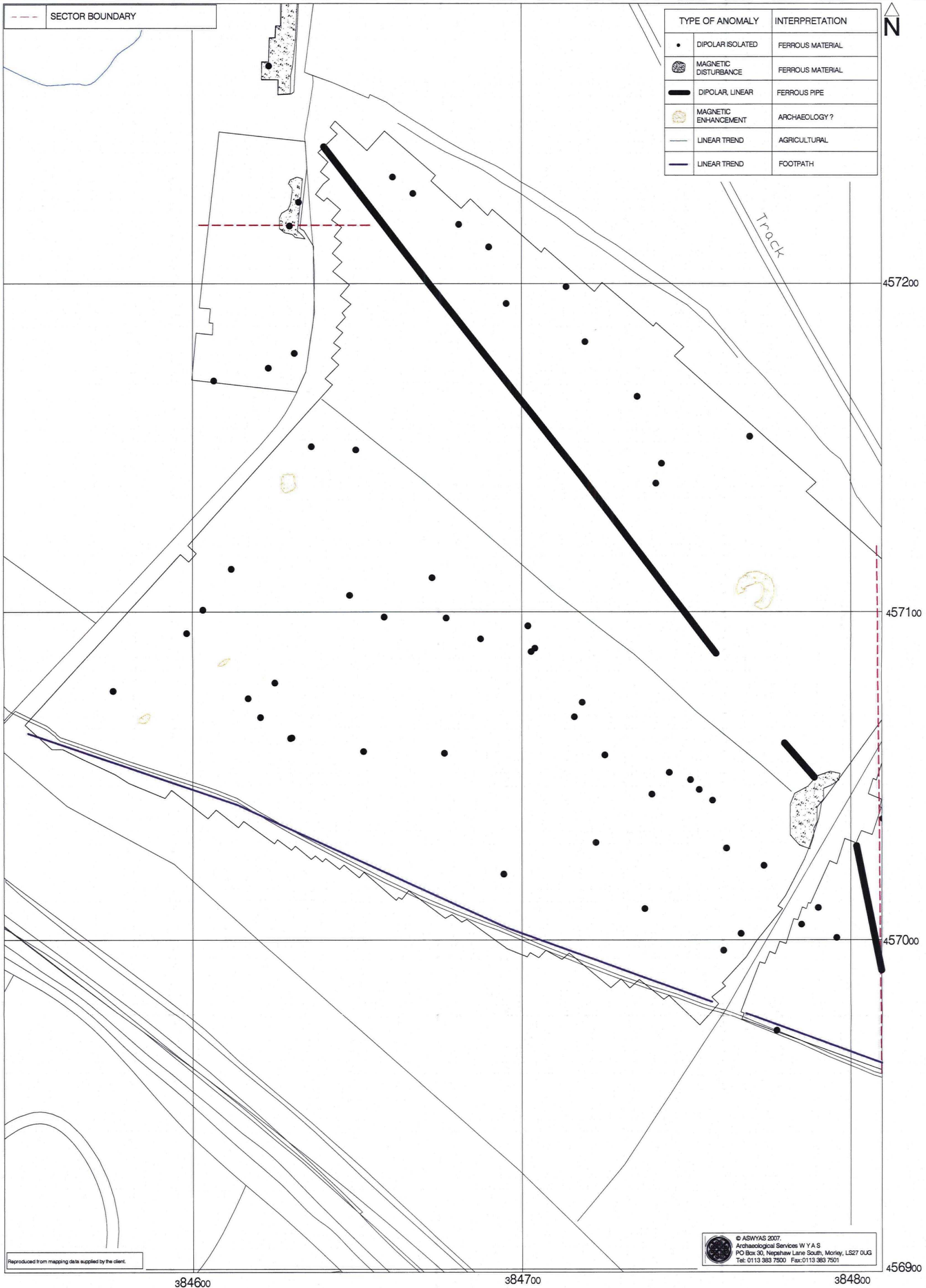
Fig. 11. Interpretation of magnetometer data; environmental centre site, western sector (1:1000 @ A3)
