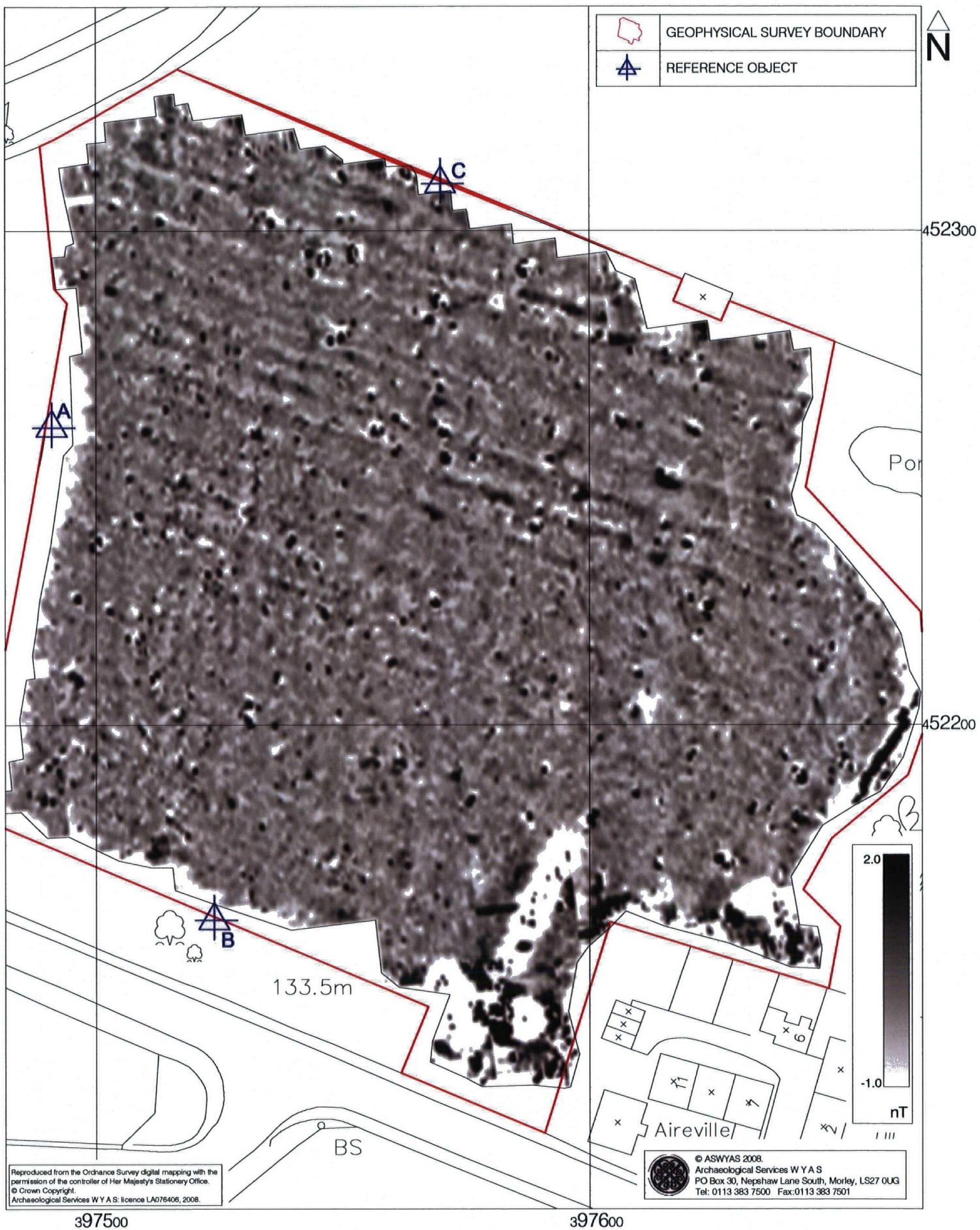
Fig. 2. Processed greyscale magnetometer data (1:1000 @ A4)
