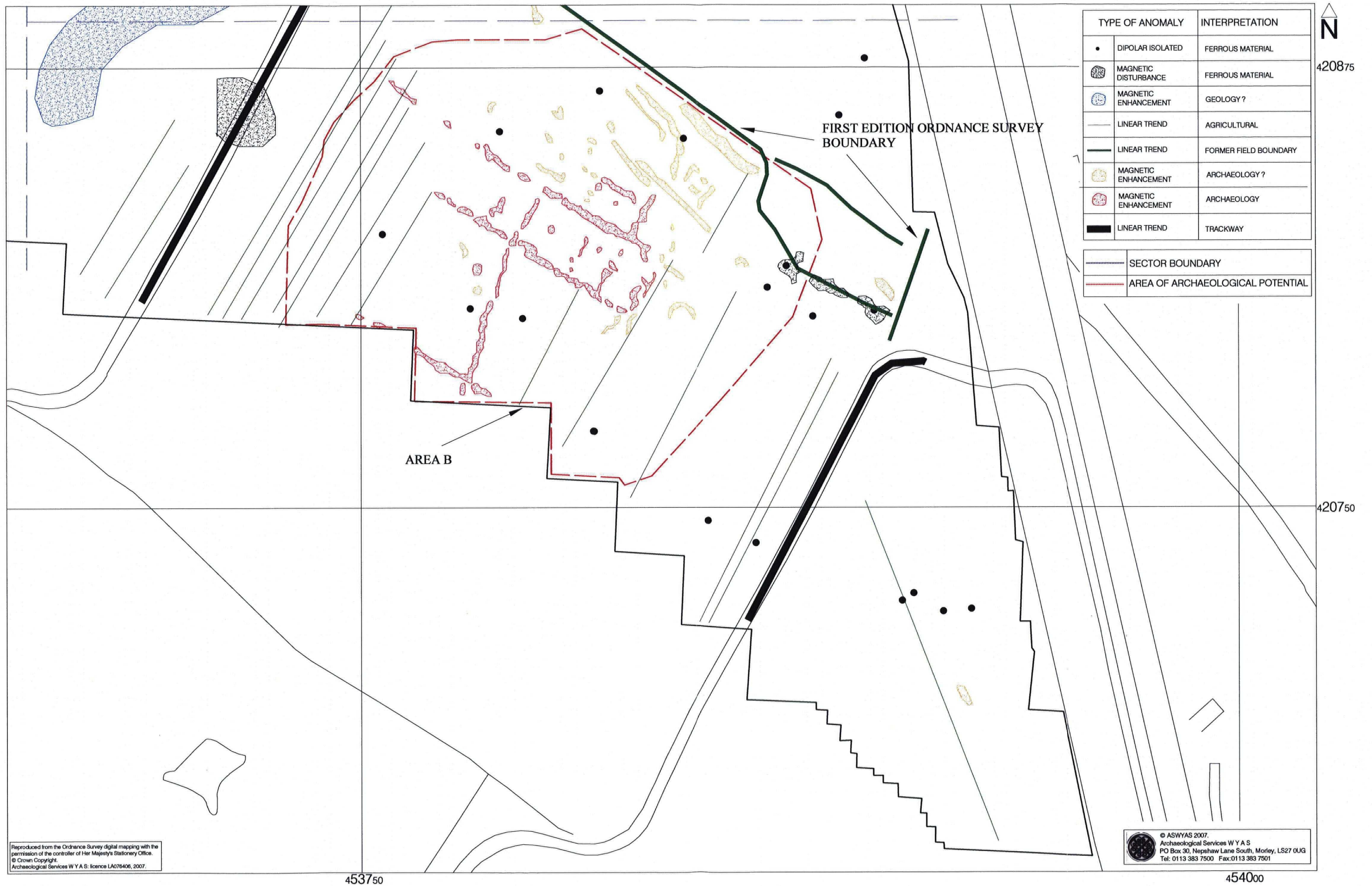
Fig. 11. Interpretation of magnetometer data; south-east sector (1:1000 @ A3)
