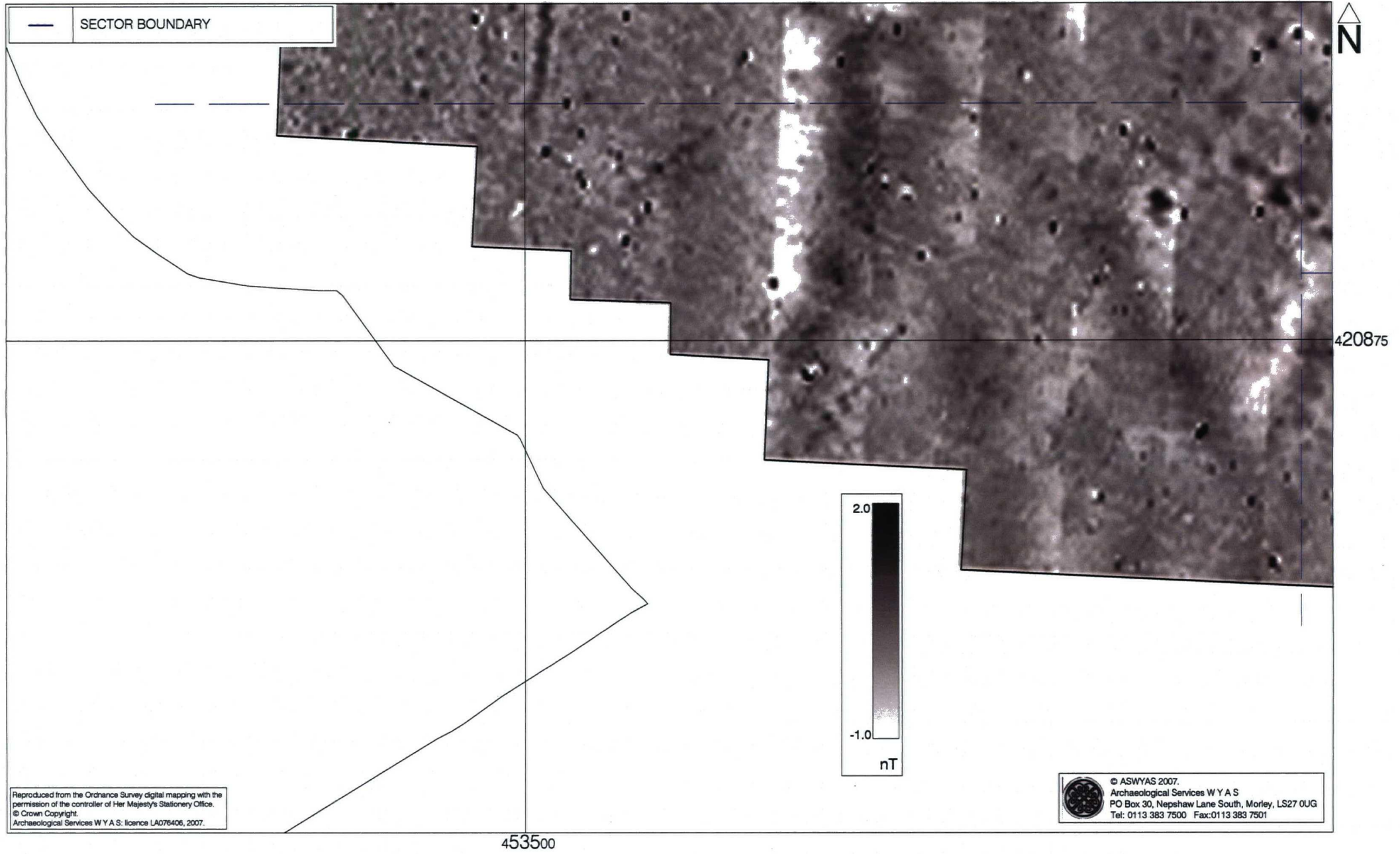
Fig. 12. Processed greyscale magnetometer data; south-west sector (1:1000 @ A4)
