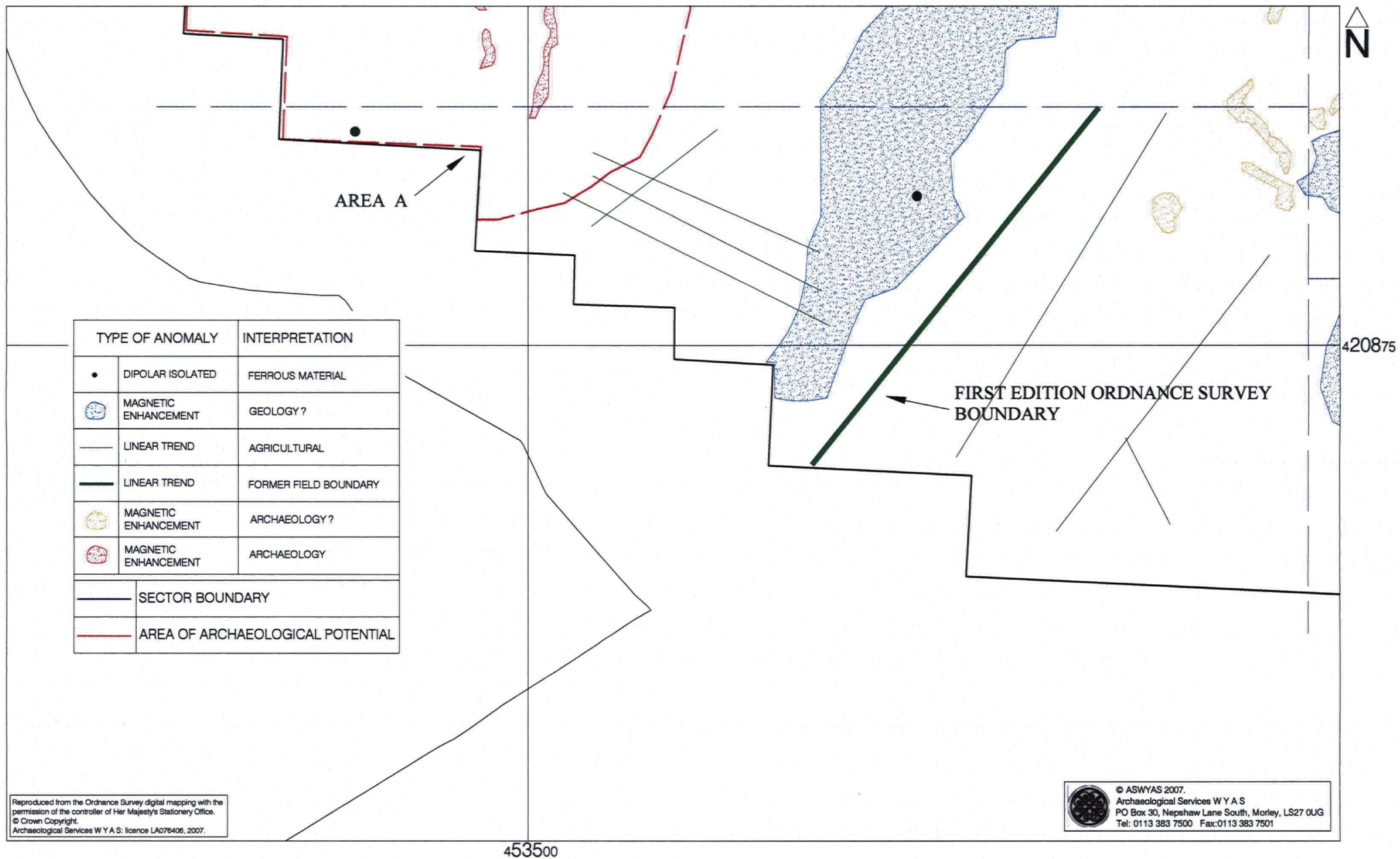
Fig. 14. Interpretation of magnetometer data; south-west sector (1:1000 @ A4)
