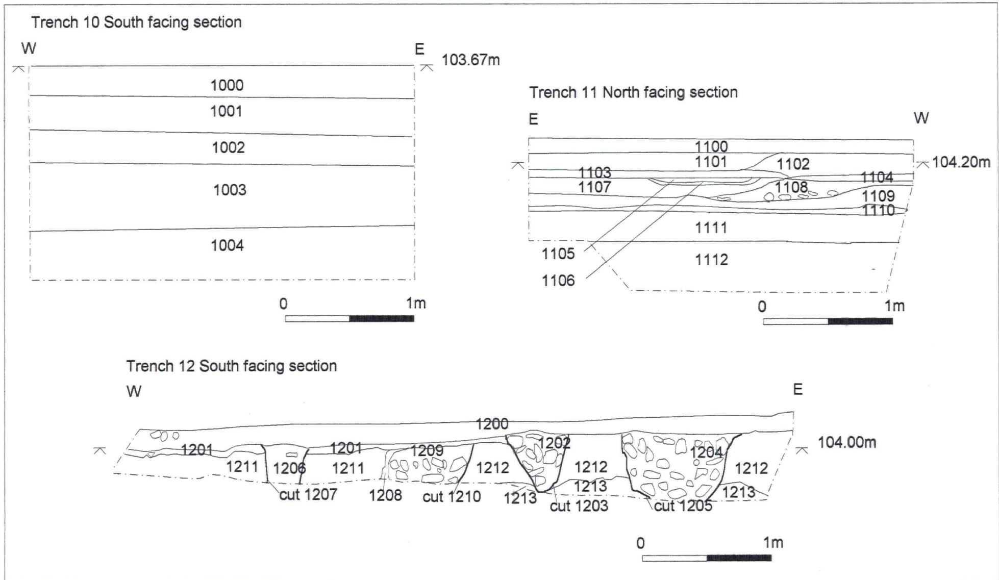
Figure 8. Trenches 10, 11 and 12 Sections.
