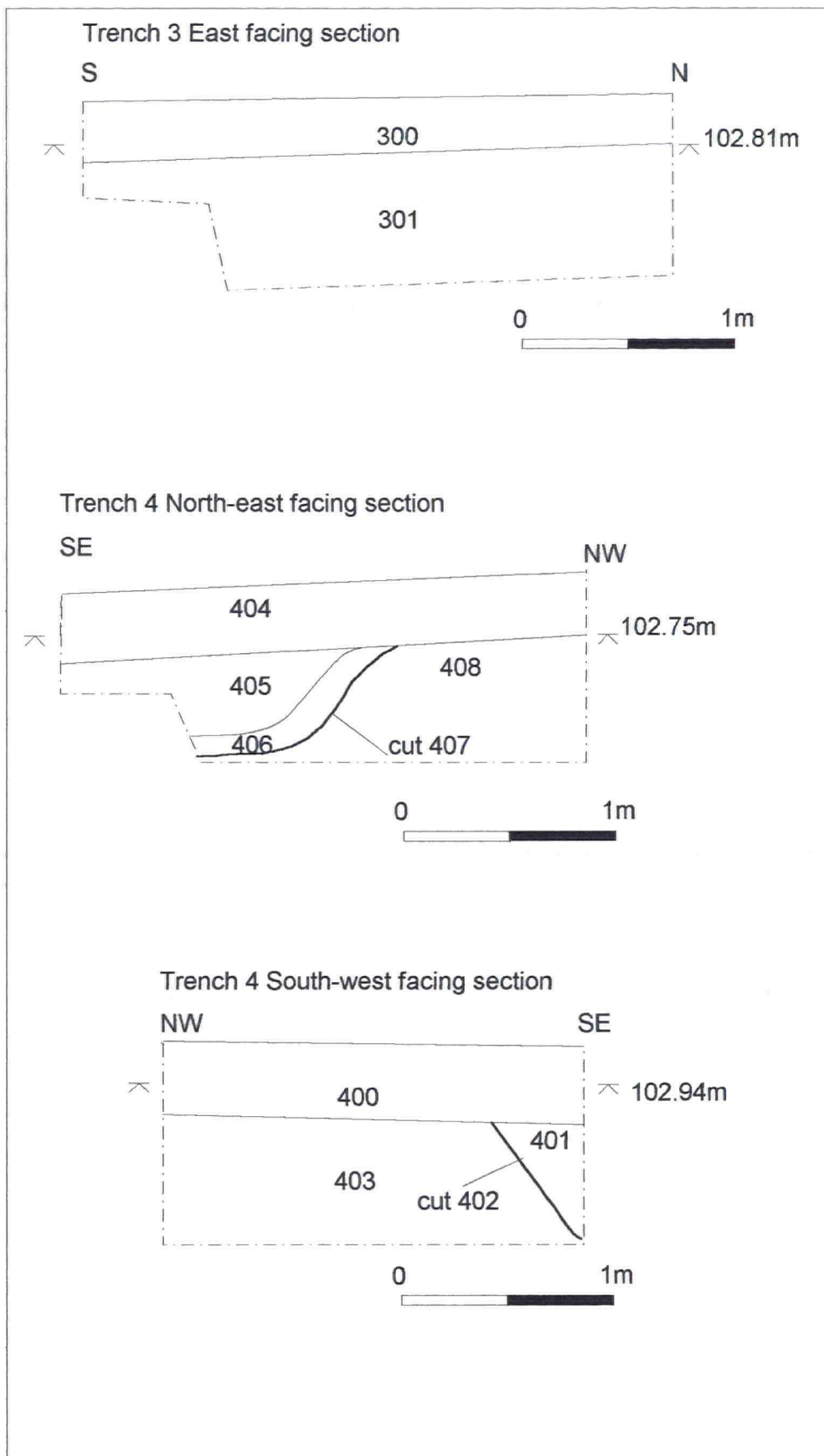
Figure 5. Trenches 3 and 4 Sections.
