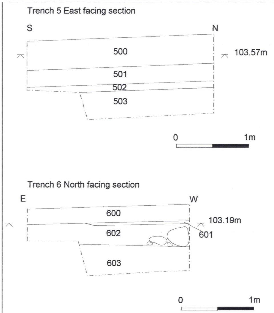
Figure 6. Trenches 5 and 6 Sections.
