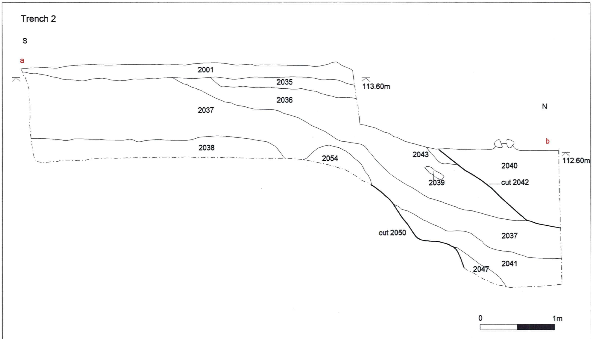
Figure 7. Trench 2 Section.
