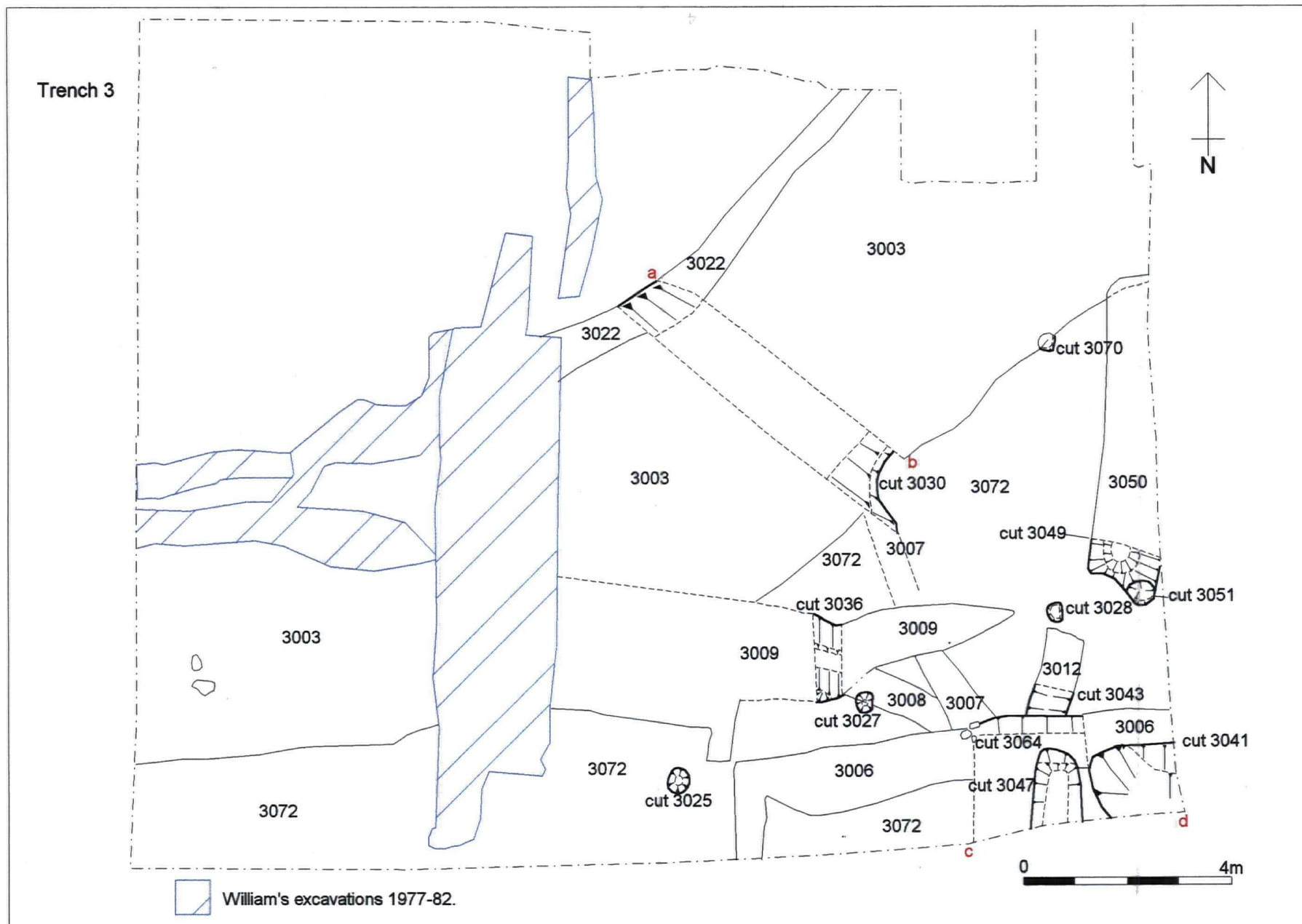
Figure 8. Trench 3 Plan.
