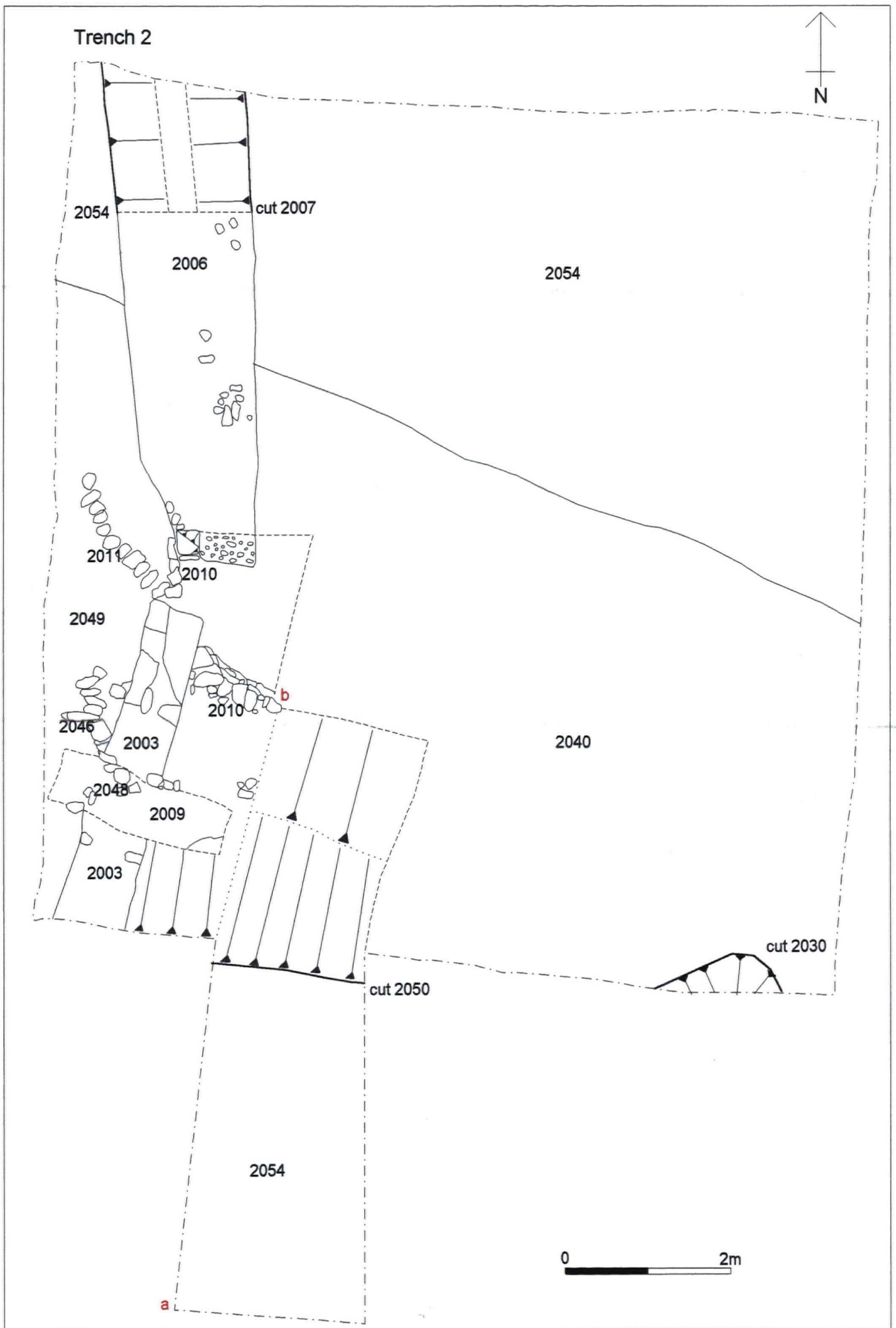
Figure 6. Trench 2 Plan.
