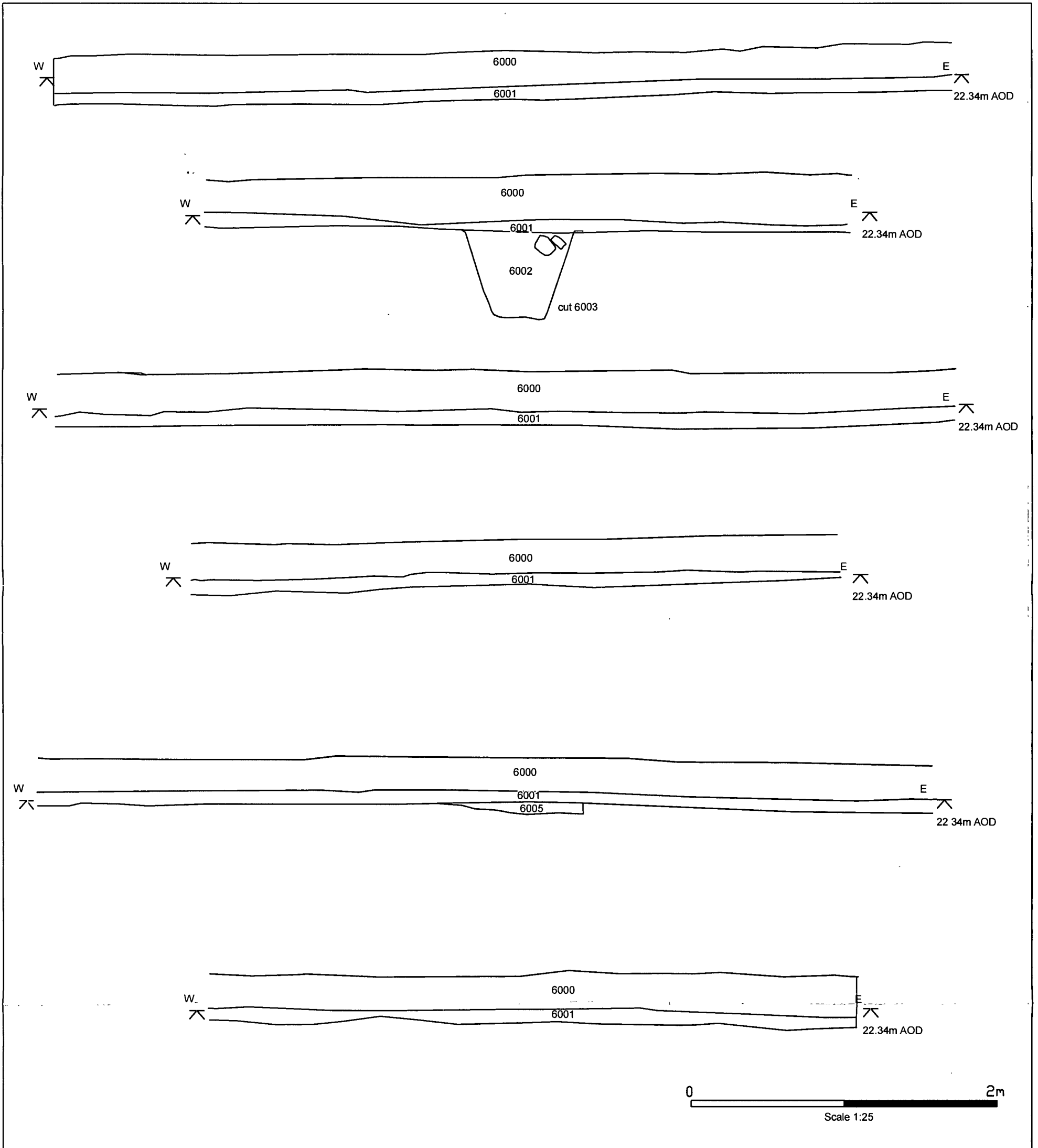
Figure 16. Trench 6 Sections.
