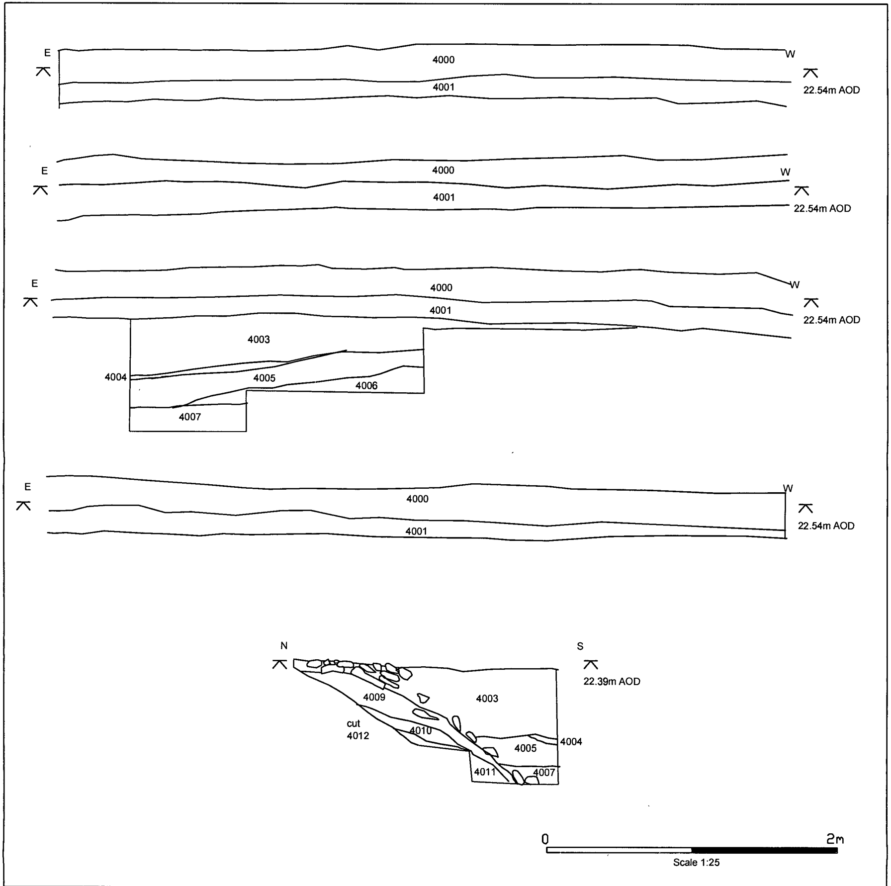
Figure 19. Trench 4 Sections.
