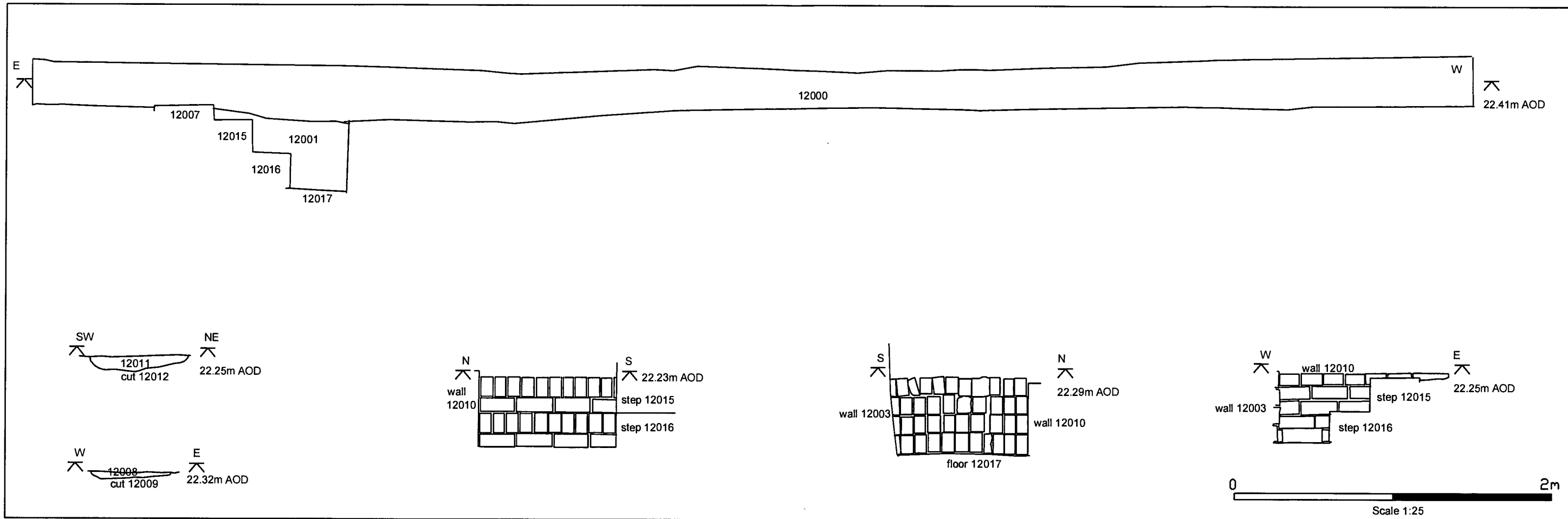
Figure 14. Trench 12 Sections.
