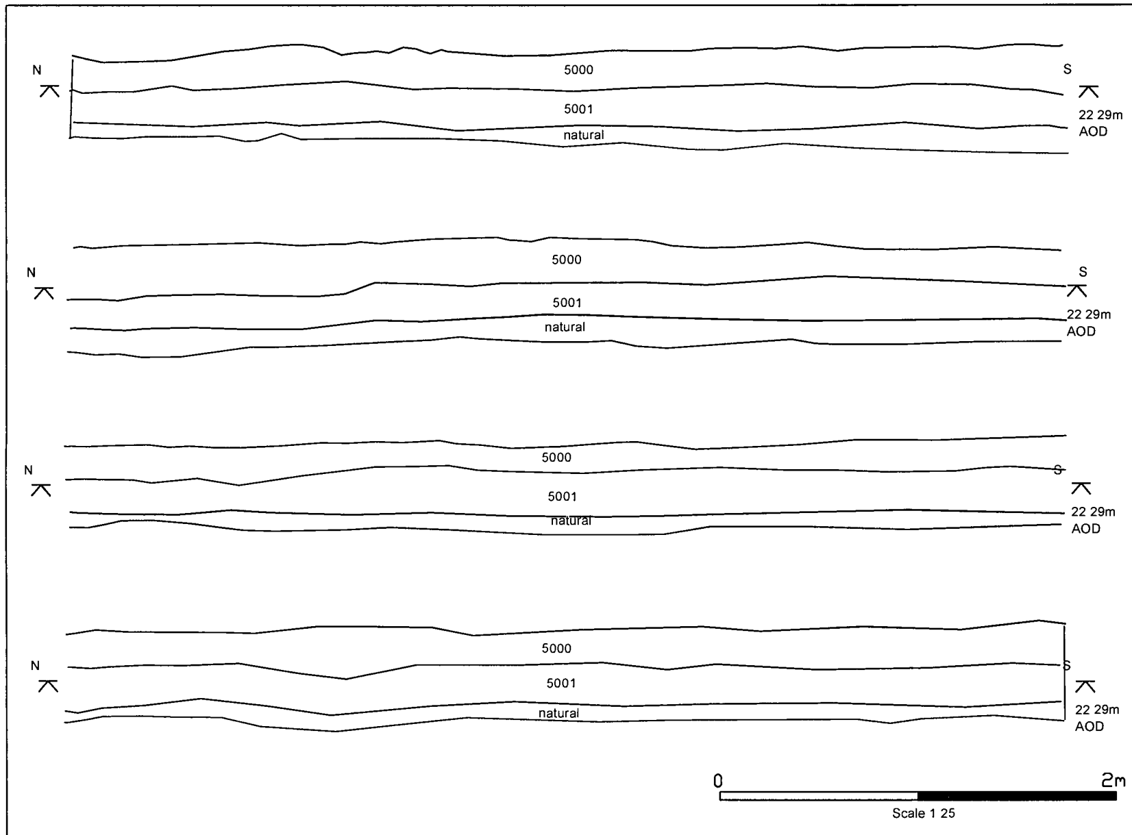
Figure 17 Trench 5 Sections
