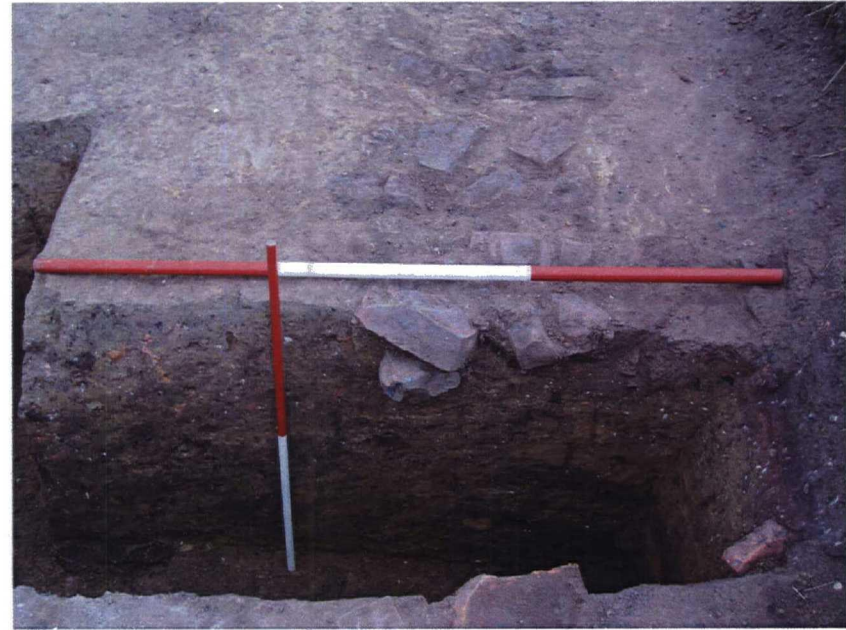
Plate 10. Trench 7 - Waster Bricks in Fill 7009. Facing South.
