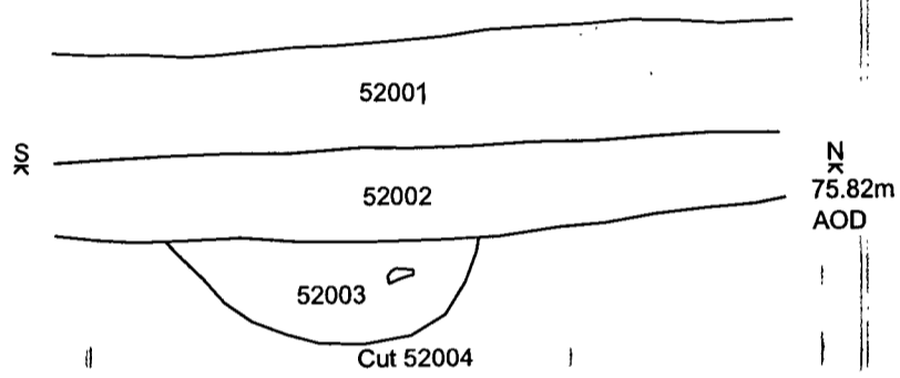
Trench 52 Section Scale 1.25
