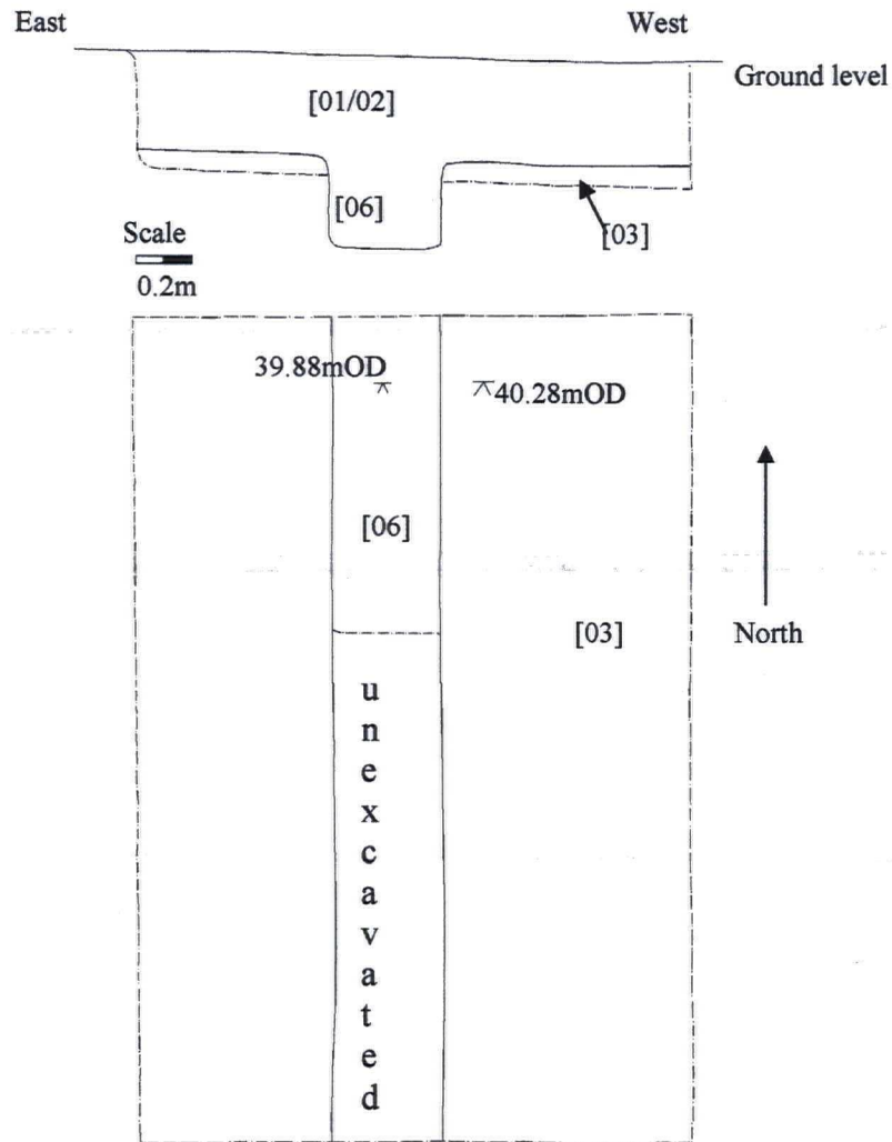
Figure 4. Trench 1. Plan and south facing section of 19 th century garden wall footings
