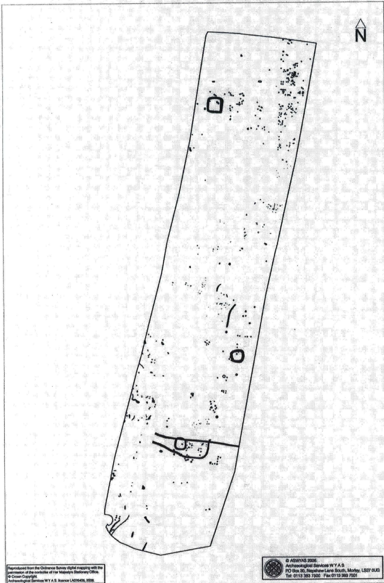
Fig. 11. Unphased features
