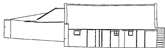
Building 14, South elevation (bids 13 & 12 projected)
