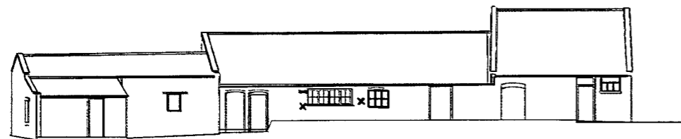
Buildings 21, 20, 19, East elevation
