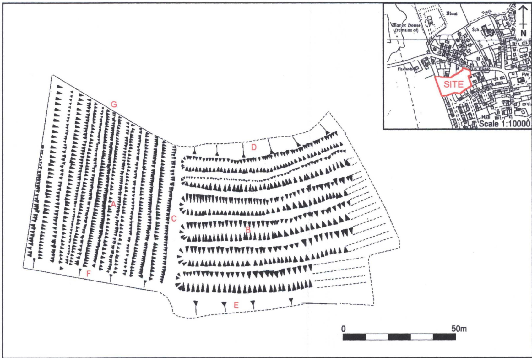
Figure 5. Earthwork plot.
